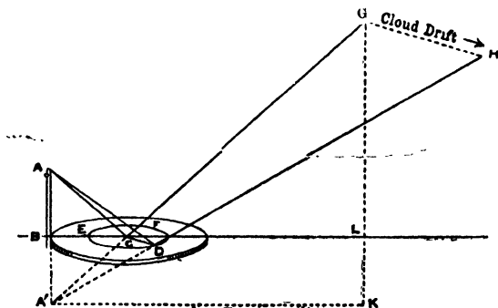
Fig. 11.—Principle of the nephoscope (From 'Meteorology' by A. E. M. Geddies, Blackie & Son, Limited.)
