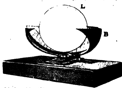
Fig. 12.—The Campbell-Stokes' sunshine recorder. From 'Meteorology' by A. E. M. Geddes, Blackie & Son, Limited
