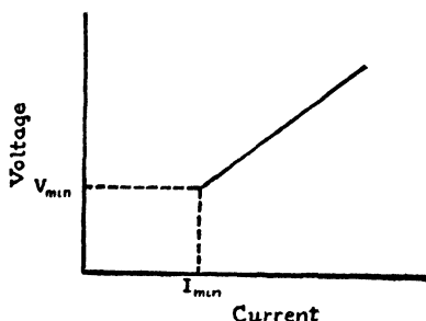
FIG. 4-2. Corona characteristic of a counter.
