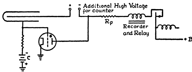
FIG. 7-2E. Combined quenching and recording circuit using a thyatron.
