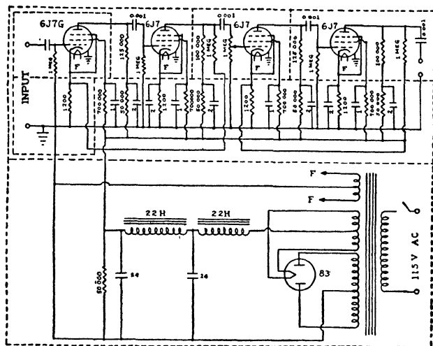
FIG. 7-8C. Four stage degenerative linear amplifier. Resistances in ohms, capacitances in microfarads. (Petruskas and Van Atta, Rev. Sci. Instr. 11, 104 (1940))
