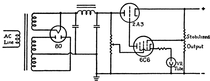
FIG. 7-6E. Voltage-regulating circuit for controlling relatively large currents.
