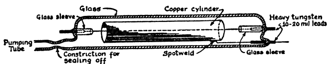
FIG. 5-1A. Glass envelope counter.
