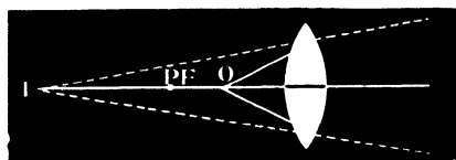
FIG. 262.—VIRTUAL FOCUS OF A CONVEX LENS.
