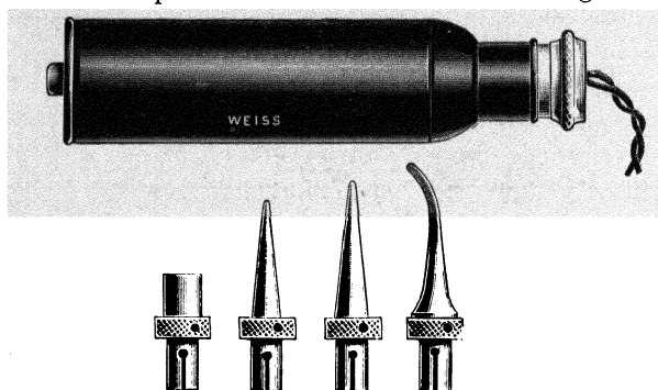
FIG. 202.—PORTABLE MAGNET.
