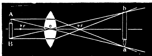
FIG. 264.—REAL, INVERTED, AND ENLARGED IMAGE FORMED BY A CONVEX LENS.
