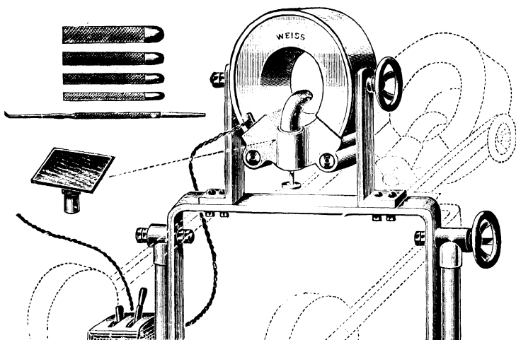
FIG. 203.—MELLINGER'S RING MAGNET.
