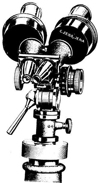
FIG. 53. — MICROSCOPE HEAD WITH DR. ULBRICH'S GRADUATED DRUM ATTACHED.
