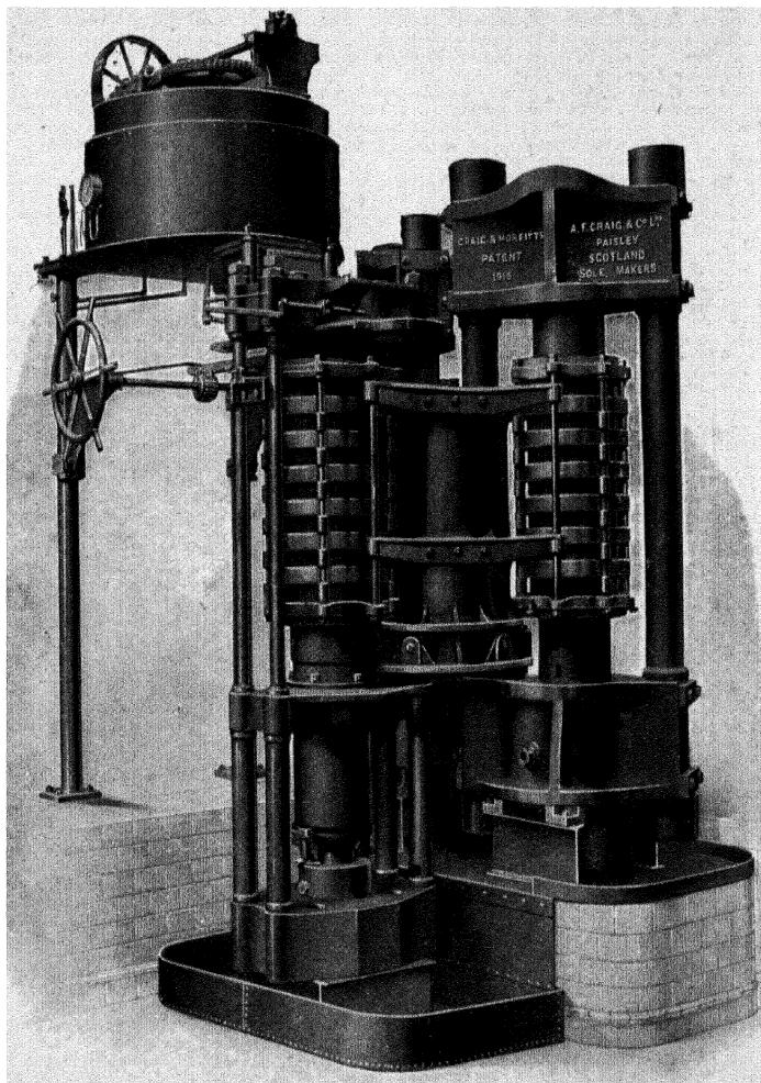
“Craig” Revolving Box Press for Copra, Palm Kernels, etc.
