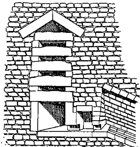
FIG. 30. Section of the relieving chambers above the King's Chamber in the Great Pyramid (after PERROT and CHIPIEZ, Histoire de VArt dans VAntiquite , p. 227).
