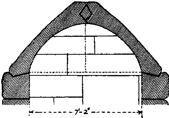
FIG. 31. Corbelled arch in the central sanctuary of the XVIIIth-Dynasty temple at El-Deir el-Bahari.
