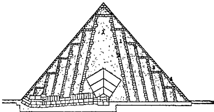
FIG. 29. Section of pyramid of King Sahure* at Abusir; Vth Dynasty (after BORCHARDT 5 Das Grabdenkmal des Konigs Sabure p. 29).
