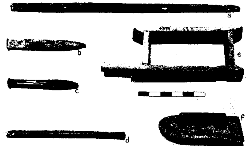
FIG 14. Ancient tools: *, Quarrymen's chisel; b , c , Mason's chisels; d , Mortise chisel; *. Wooden brickmaker's mould; /, Plasterer's tool. All New Kingdom. Cairo Museum. The scale is in inches
