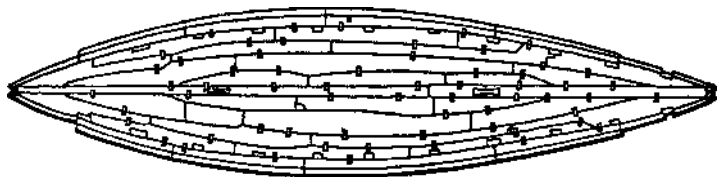
FIG. 16. Plan of a royal barge from El-Lisht showing its construction of small pieces of wood. XIIIth Dynasty; Cairo Museum.
