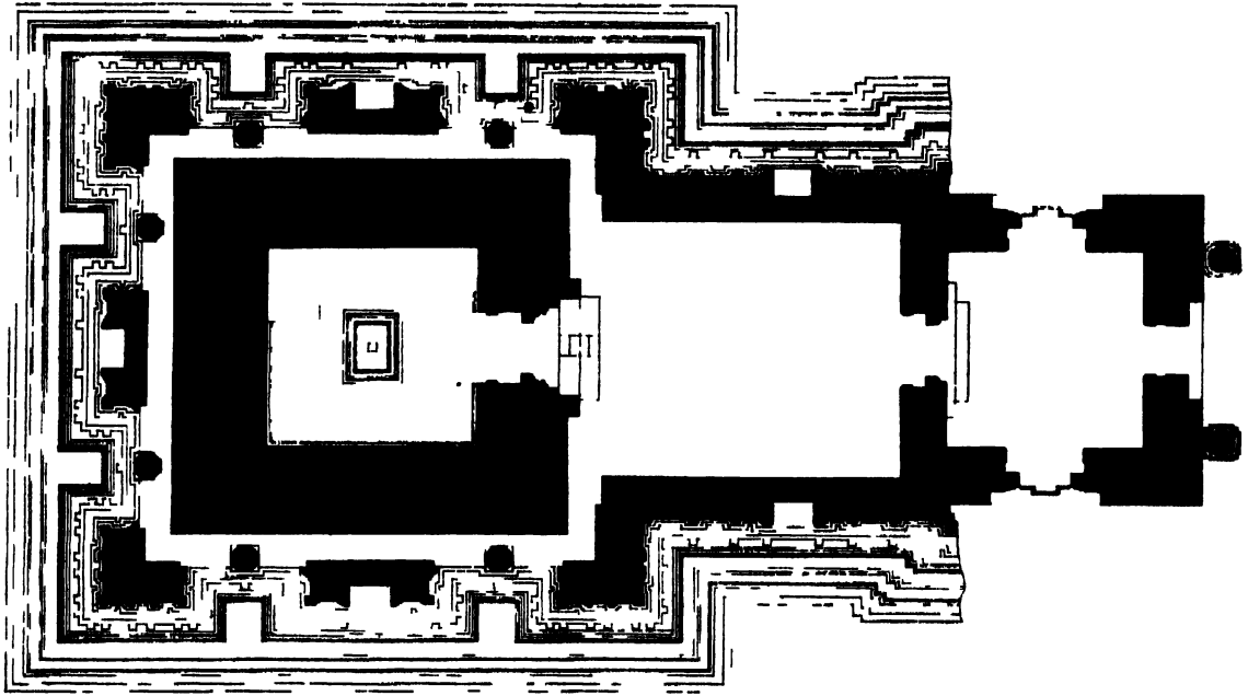
(b) PLAN OF THE TEMPLE AT DICHPALI (NIZAMABAD). SCALE 15' TO 1".
