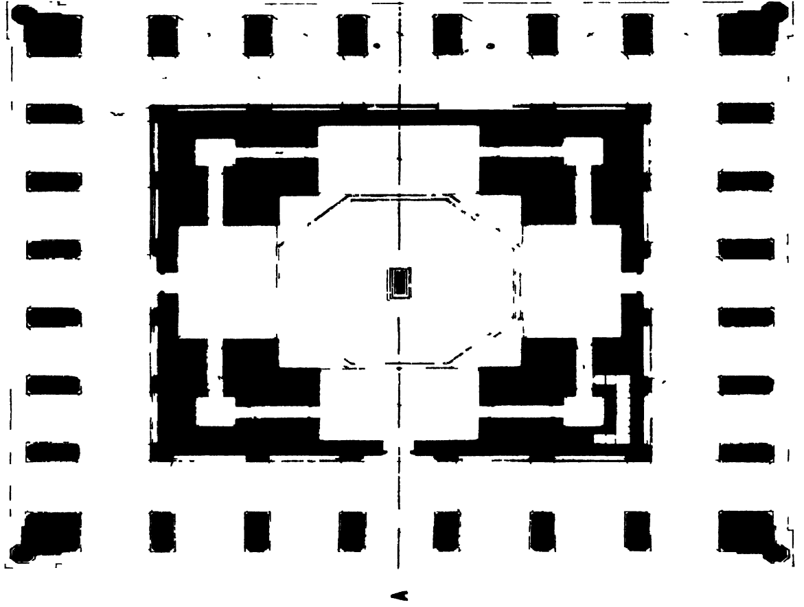
(b) PLAN OF ABDULLAH QUTB SHAH'S TOMB AT GOLCONDA. SCALE 24' TO 1'.
