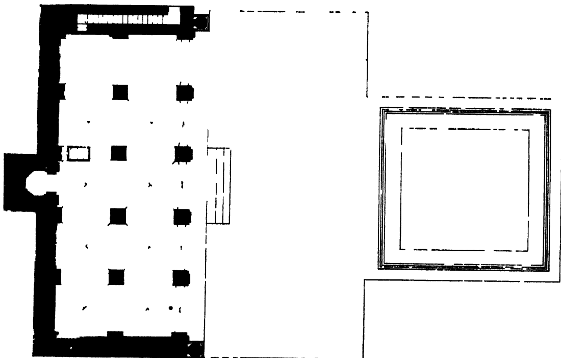
(c) PLAN OF THE JAMI MASJID AT BILOLI (NIZAMABAD). SCALE 15' TO 1".
