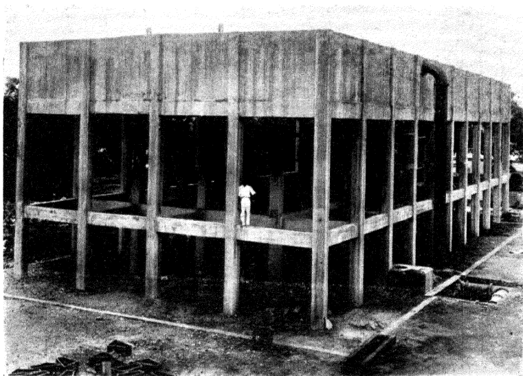
150,000 GALS. R. C. C. TANK FOR WATER WORKS Contractors : Hindustan Construction Co. Ltd.
