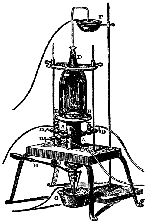
HARE'S APPARATUS FOR DEFLAGRATING CARBURETS.
