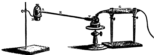
HARE'S DISTILLATORY APPARATUS.
