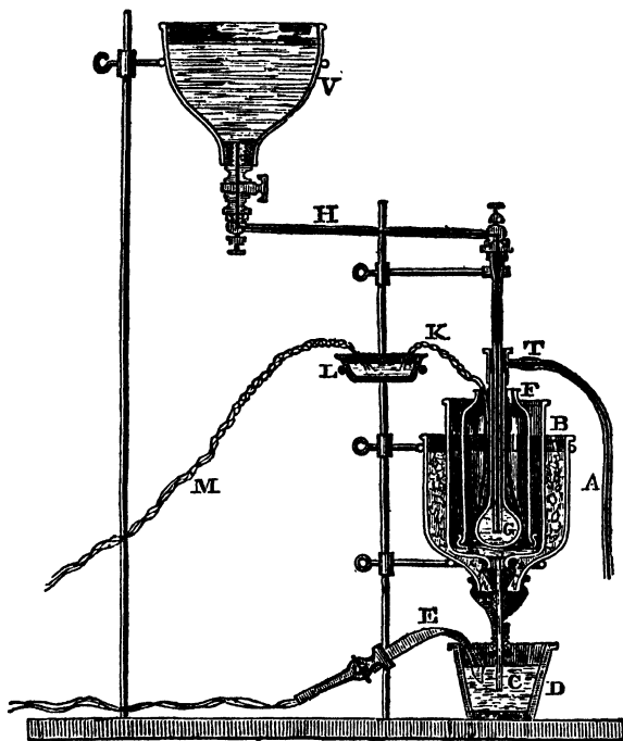
HARE'S APPARATUS FOR OBTAINING AMALGAMS, ETC.
