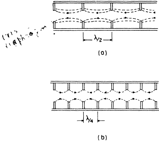
FIG. 5-7. Longitudinal cross section of circular wave guides for electron linear accelerators. (a) Iris-loaded wave guide for a standing wave accelerator; diaphragms are located at \frac{1}{2}\lambda intervals, the \pi -mode. (b) Traveling wave waveguide. Diaphragms are located at \frac{1}{4}\lambda intervals, the \pi/2 -mode.
