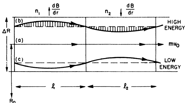
FIG. 7-5. Orbits for particles deviating from equilibrium energy.
