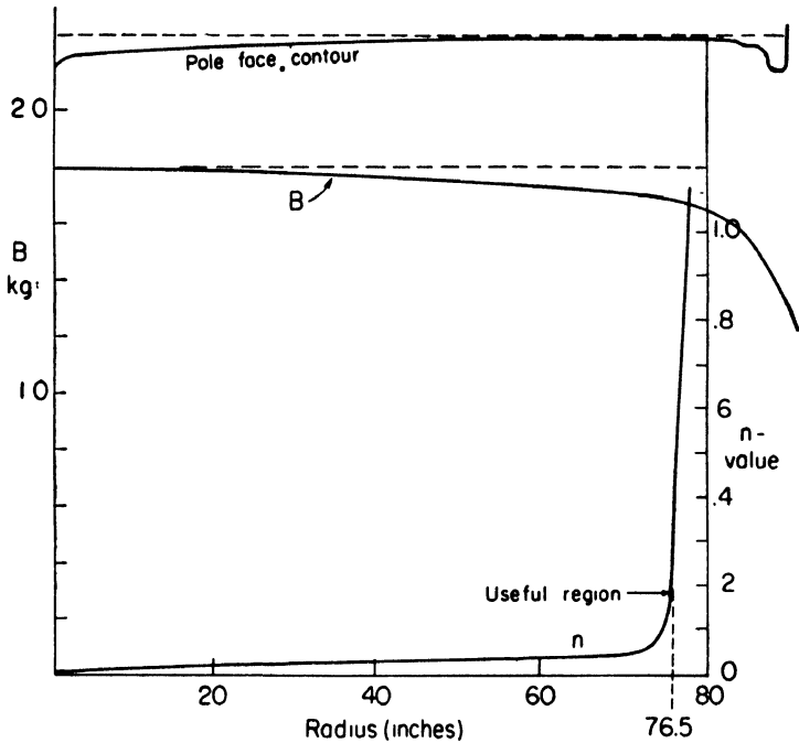
FIG. 4-5. Pole face contour of the Chicago magnet to provide the radially decreasing field needed for focusing, with a plot of flux density vs. radius at one value of excitation. The plot of n -value vs. radius illustrates the extent of the useful region of field.
