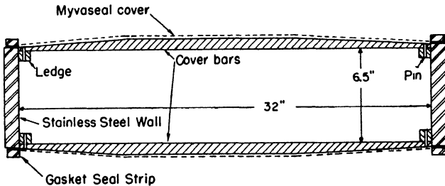
FIG. 6-5. Cross section of the cosmotron vacuum chamber.
