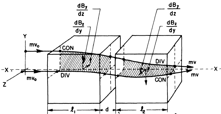
FIG. 7-2. Double focusing by a pair of matched magnetic lenses, in which the sense of the magnetic gradients is reversed.
