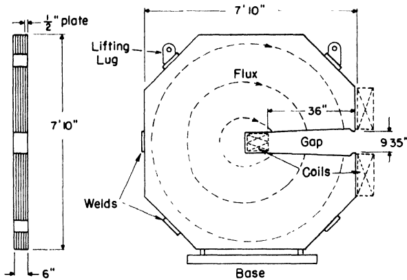
FIG. 6-2. Cross section of C-magnet and assembly of \frac{1}{2} -in. plates into blocks.
