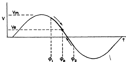
FIG. 2-5. Phase oscillation about equilibrium phase \phi_e between arbitrary limits \phi_1 and \phi_2 .
