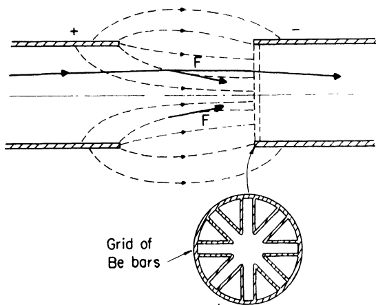
FIG. 5-6. Convergent forces on acceleration between a cylinder and a plane electrode or grid.
