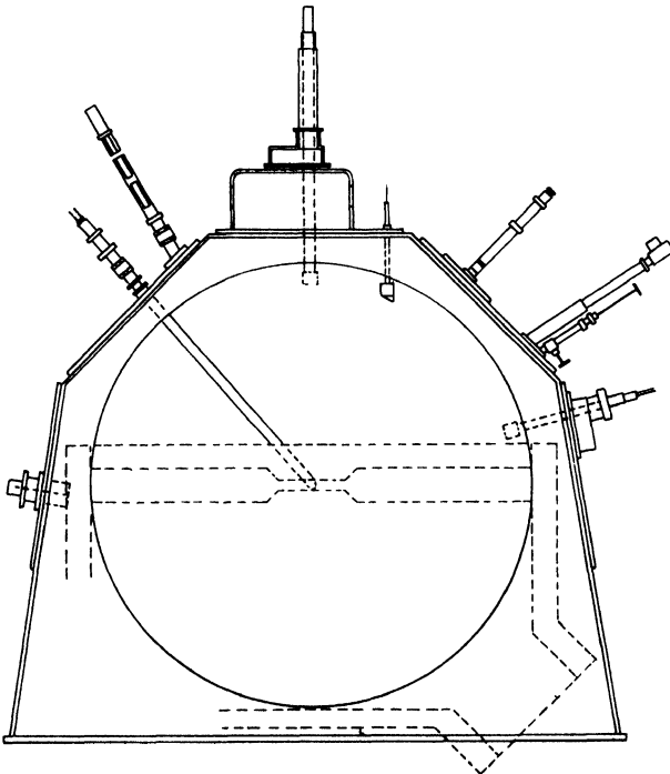
FIG. 4-7. Vacuum chamber for the Rochester synchrocyclotron.
