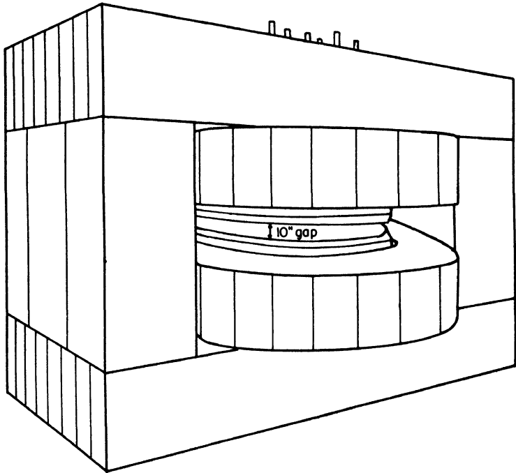
FIG. 4-4. Schematic diagram of the Chicago 170-in. diameter synchrocyclotron magnet, showing the assembly of slabs and disks. The magnet is excited by two current carrying coils located symmetrically about the gap.
