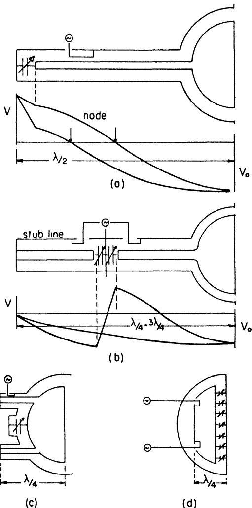
FIG. 4-6. Variable frequency rf systems for the synchrocyclotron. (a) Half-wave resonant D-line with variable capacitor at end of D-stem; (b) three-quarter wave system using variable capacitor and quarter-wave stub line; (c) quarter-wave D-stems with variable capacitor at back of the D; (d) quarter-wave D with variable capacitor on the diametral face of the D.
