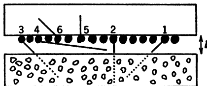
FIG. 21. Track registration from external thin sources. Showing powder film on glass backing separated from emulsion by a small air gap l . This clearance is provided by narrow cardboard or metal spacers 0.05 cm thick.
