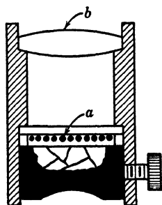
FIG. 4. Spinharscope for detecting alpha particles from polished sections.
