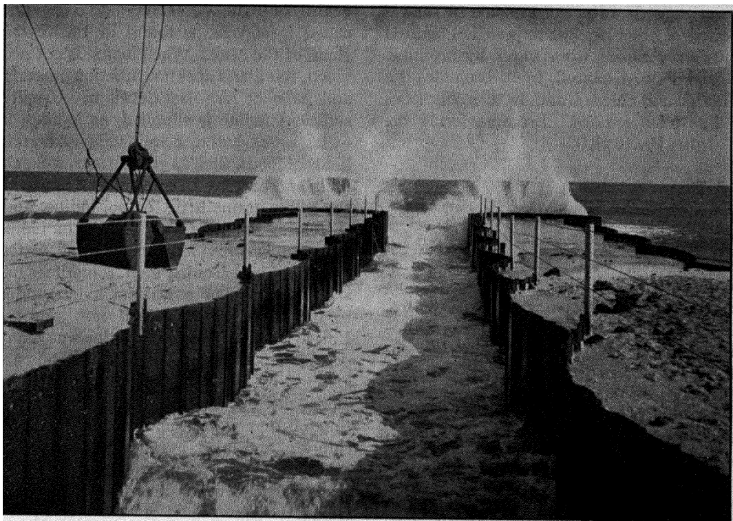
Figure 177. Intake through which Sea Water is Obtained for Use in the Extraction of Bromine and Magnesium
