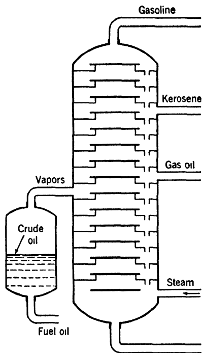
Figure 238. Bubble Tower
