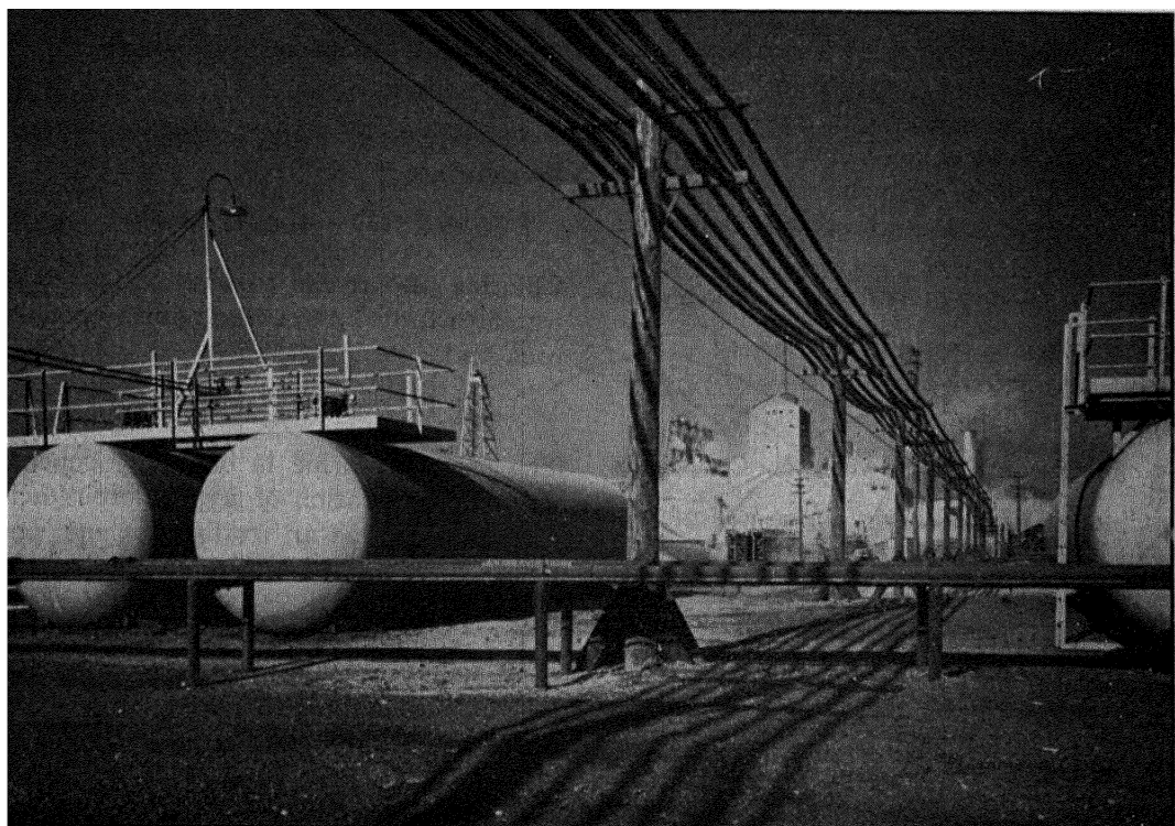
Figure 176. Storage Tanks for Liquid Chlorine (Courtesy of Columbia Chemical Division, Pittsburgh Plate Glass Company)
