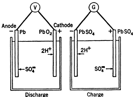
Figure 262. The Lead Storage Battery
