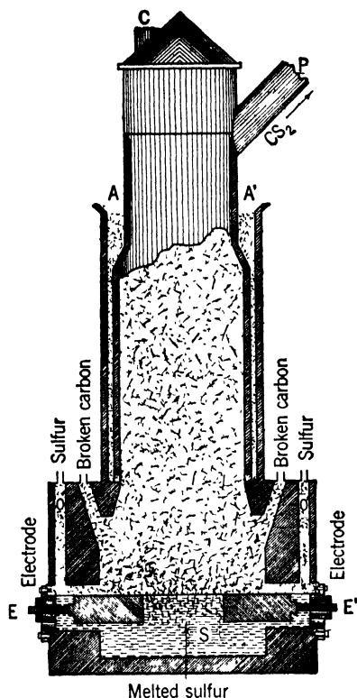
Figure 194. Production of Carbon Disulfide in the Electric Furnace
