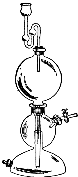
Figure 54. A Kipp Generator
