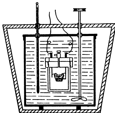
Figure 75. A Calorimeter
