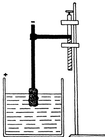
Figure 266. The Preparation of Metallic Calcium
