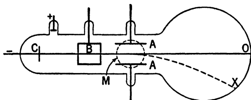
Figure 82. The Cathode-Ray Tube
