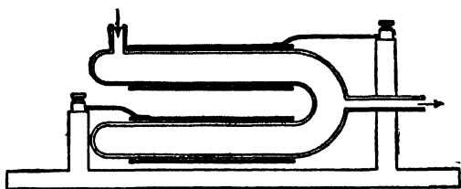
Figure 49. Apparatus Used to Produce Ozone by Means of an Electrical Discharge
