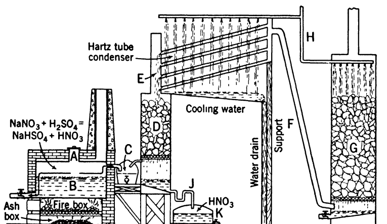
Figure 213. Nitric Acid Plant
