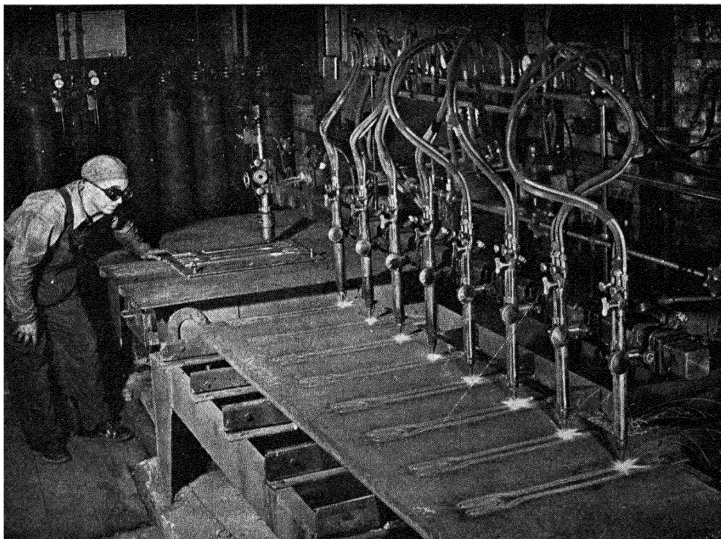
Figure 48 Eight Torches Mounted on a Bar for Cutting Purposes in a Multiflame Machine (Courtesy of Air Reduction Sales Company)
