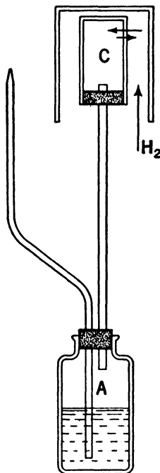
Figure 62. Apparatus Used to Show the Different Rates of Diffusion of Hydrogen and Air
