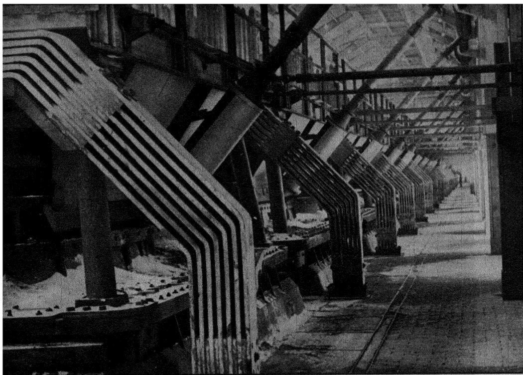
Figure 275. Line of Electrolytic Cells in Which Aluminum Oxide is Reduced in Making Aluminum (Courtesy of Aluminum Company of America)
