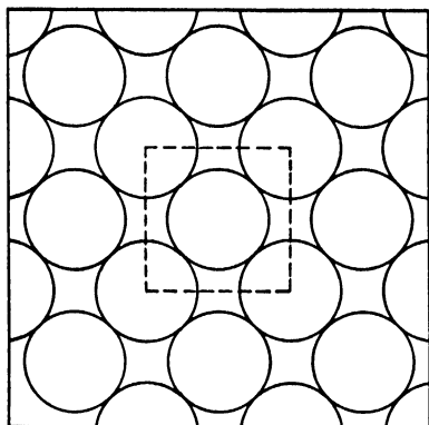
Figure 122. A Face of a Face-Centered Crystal Pattern, Showing the Packing of Atoms
