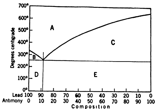
Figure 265. Lead-Antimony Alloy Diagram
