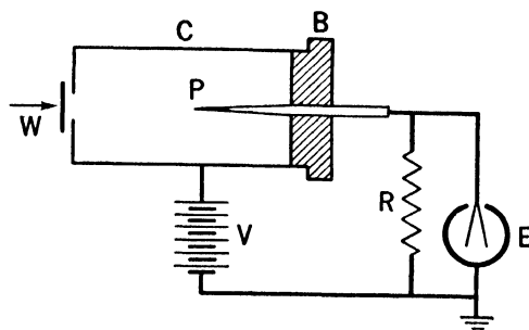
Figure 80. Geiger Point Counter
