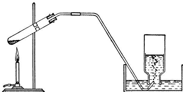
Figure 47. The Preparation of Oxygen from Potassium Chlorate
