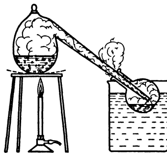
Figure 212. The Preparation of Nitric Acid in the Laboratory
