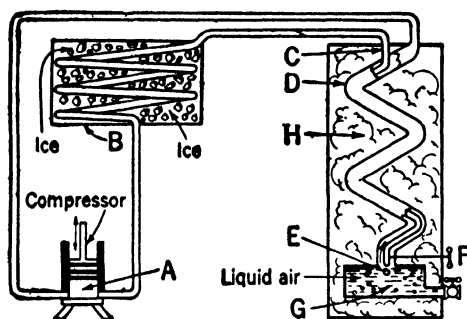
Figure 45. The Liquefaction of Air
