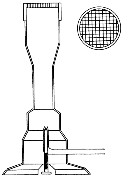
Figure 243. Meker Burner
