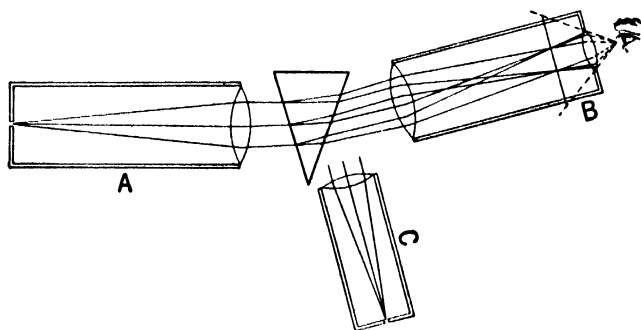
Figure 99. The Essential Parts of a Spectroscope
