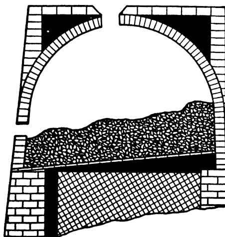
Figure 187. Beehive Coke Oven
