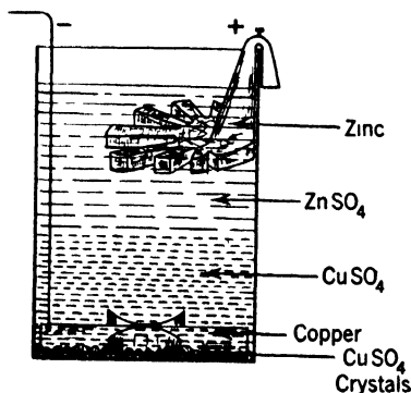
Figure 260. The Gravity Cell
