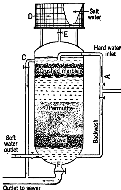
Figure 269. The Permutite Water Softener
