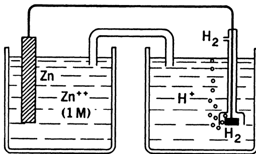
Figure 259. The Measurement of Electrode Potentials
