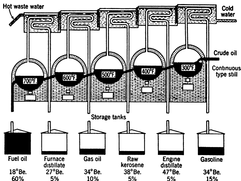
Figure 237. Diagram Showing the Fractional Distillation of Petroleum
