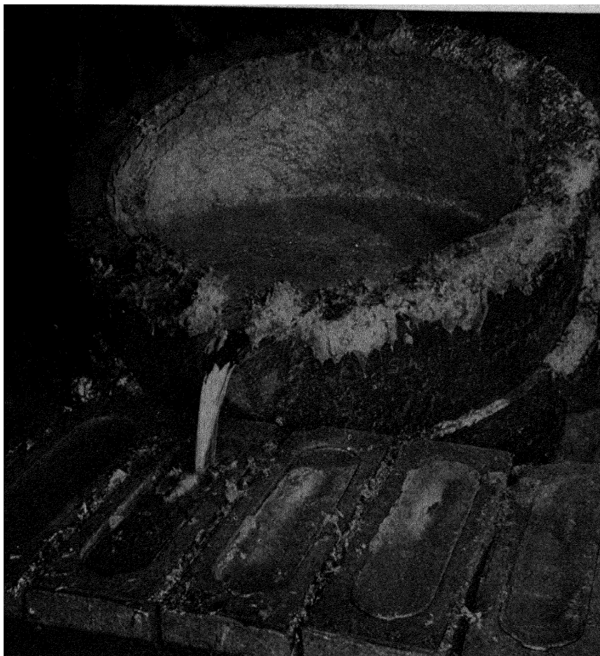
Figure 274. Pouring Molten Aluminum from Ladle into Pig Molds (Courtesy of Aluminum Company of America)
