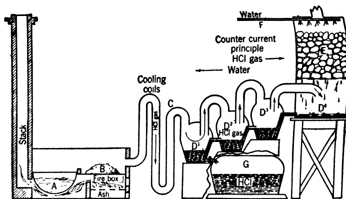
Figure 181. Diagram of a Plant Producing Hydrochloric Acid
