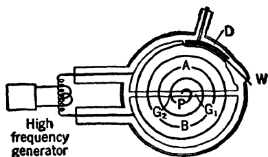
Figure 92. The Cyclotron
