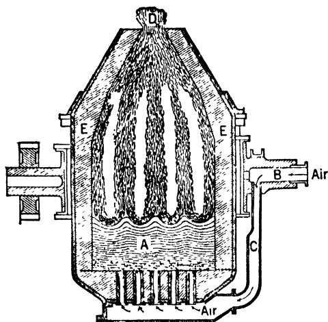
Figure 282. The Bessemer Converter
