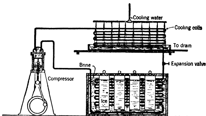
Figure 211. The Production of Ice by Means of Ammonia
