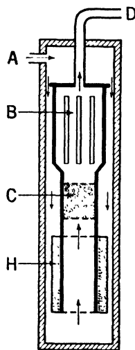
Figure 209. The Reaction Chamber of the Haber Synthetic Ammonic Process
