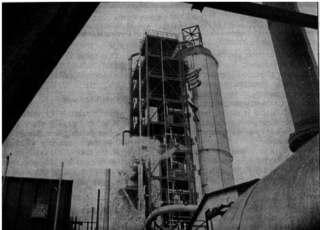
Figure 240. Pipe Still and Bubble Tower Used in Refining Lubricating Oils (Courtesy of Standard Oil Company)
