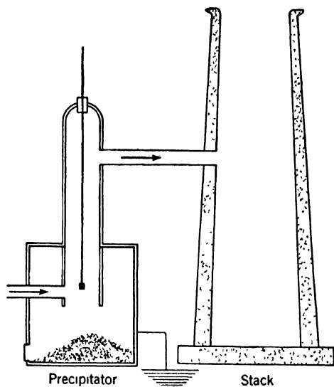
Figure 163. Cottrell Electrical Precipitator
