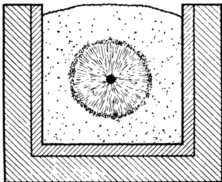
Figure 196. Cross Section of a Silicon Carbide Furnace
