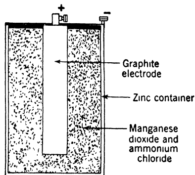
Figure 261. The Dry Cell
