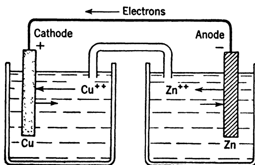
Figure 258. The Zinc-Copper Cell
