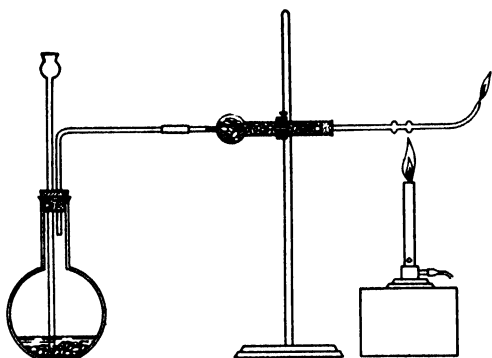
Figure 229. Diagram of Apparatus Used in the Marsh Test for Arsenic
