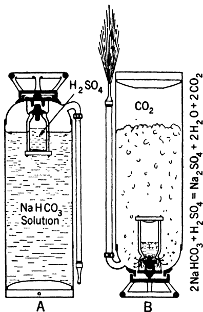
Figure 192. Fire Extinguisher
