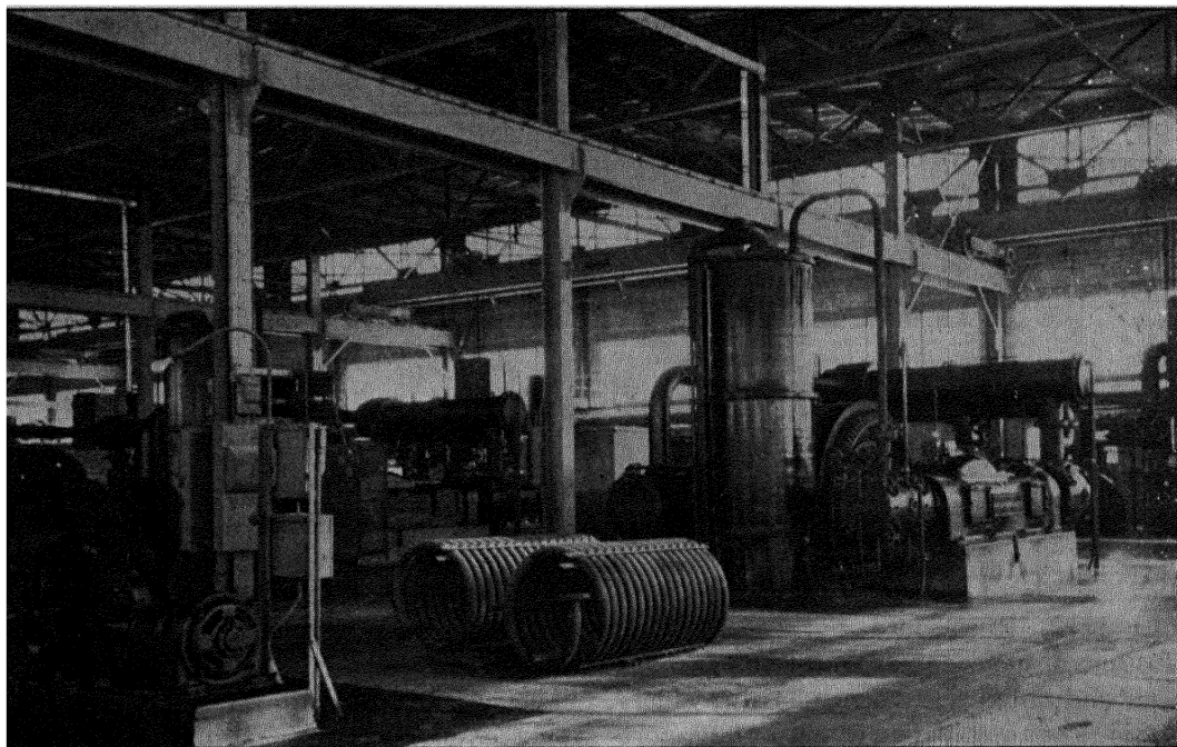
Figure 205. Plant in Which Nitrogen Gas is Distilled from Liquid Air (Courtesy of American Cyanamid Company)
