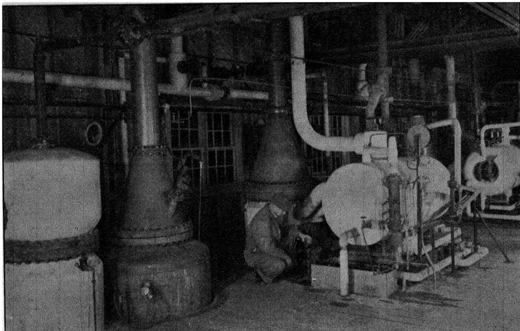
Figure 215. Ammonia Burners and Waste Heat Boilers in Plant Producing Nitric Acid from Ammonia (Courtesy of Chemical Construction Company)
