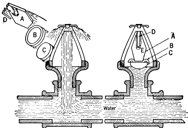
Figure 230. Automatic Sprinkler
