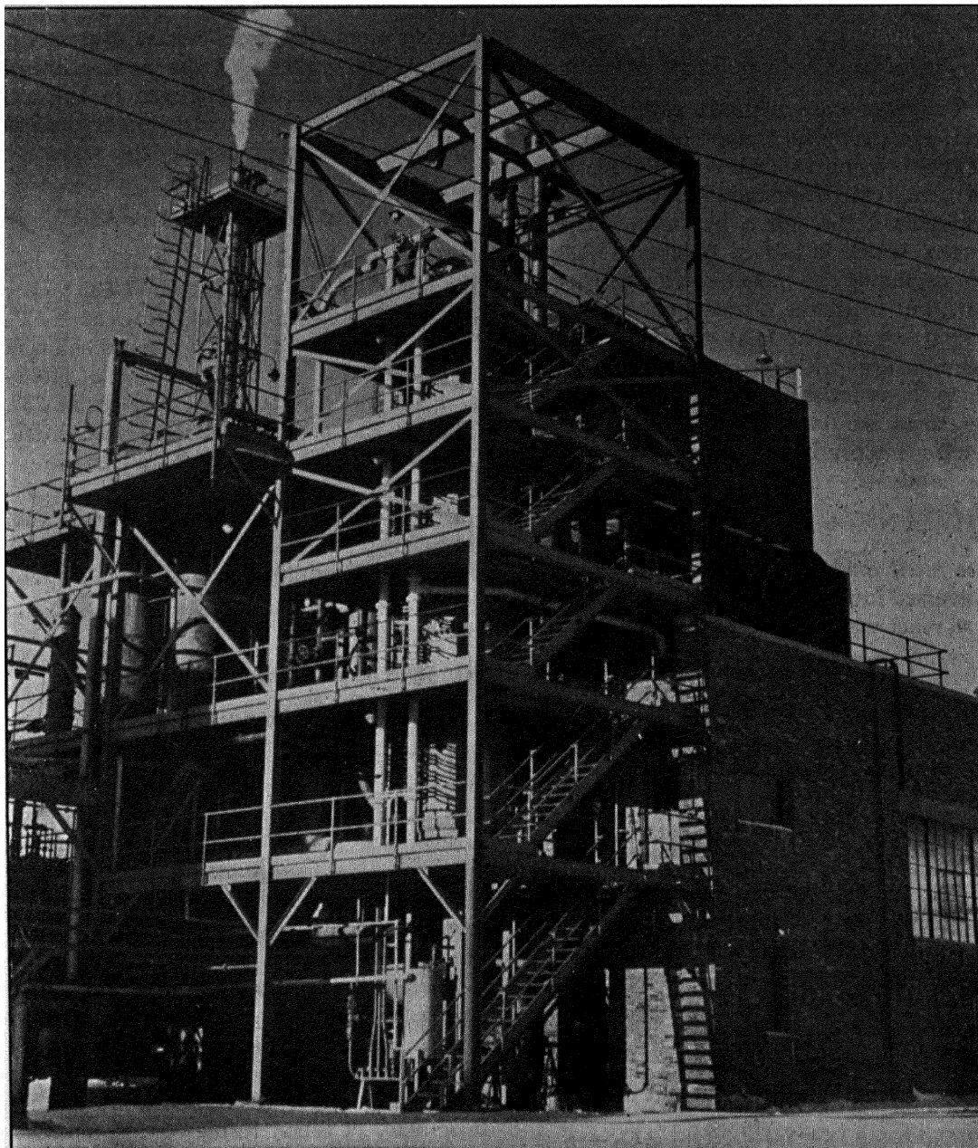
Figure 214. Synthetic Nitric Acid Plant (Courtesy of Monsanto Chemical Company)
