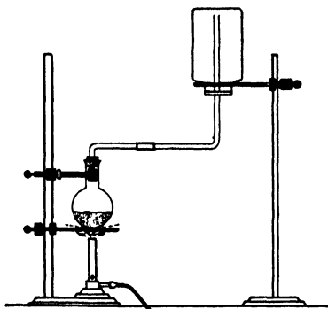
Figure 208. The Preparation of Ammonia and Its Collection by the Downward Displacement of Air
