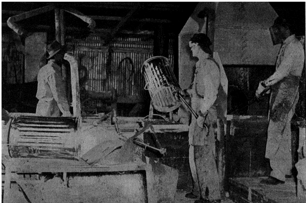
Figure 272. Galvanizing Garbage Cans
