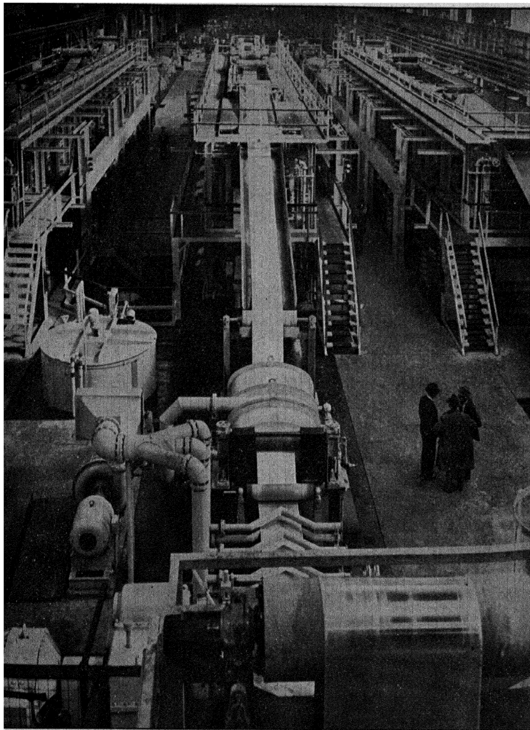
Figure 277. Electrofinning Steel Sheets
