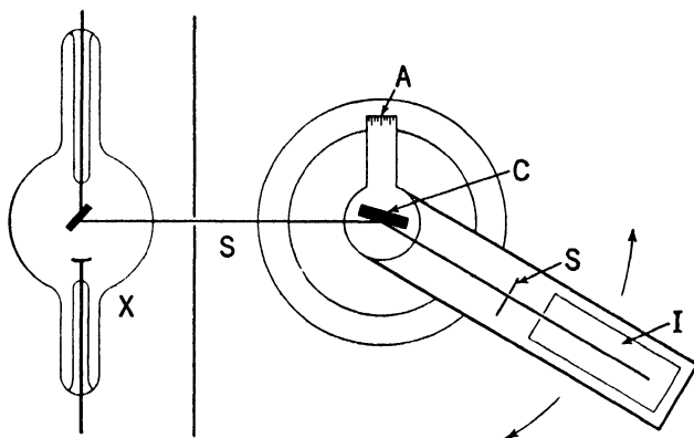
Figure 106. Apparatus Used to Study the Structures of Crystals by Means of X-Rays
