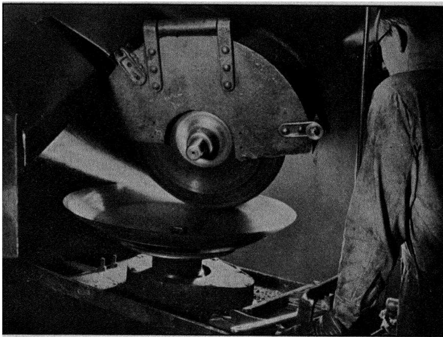
Figure 276. Polishing Cultivator Disks with a Wheel Coated with an Aluminum Oxide Abrasive, Alundum (Courtesy of Norton Company)
