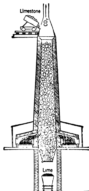
Figure 267. Lime Kiln
