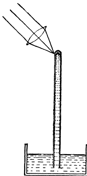
Figure 43. The Apparatus Used by Priestley in the Experiments by Which He Discovered Oxygen
