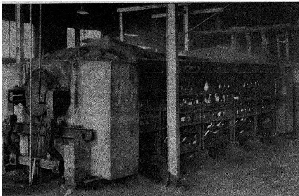
Figure 195. Resistance Type of Electric Furnace in Which Sand and Coke Are Converted into Silicon Carbide
