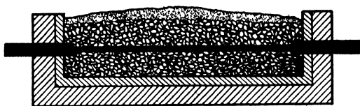
Figure 185. The Production of Graphite in the Electric Furnace
