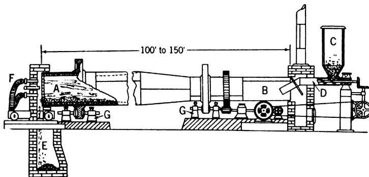
Figure 270. Cement Kiln
