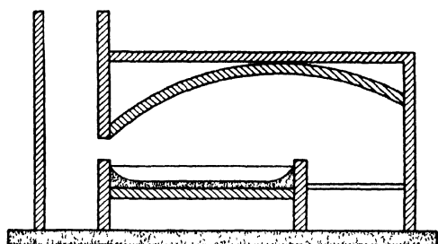
Figure 281. Puddling Furnace
