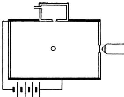
Figure 84. Millikan's Apparatus
