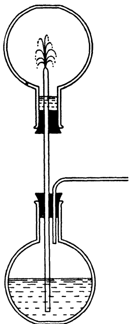
Figure 182. A Method by Which the Solubility of Hydrogen Chloride in Water can be Demonstrated
