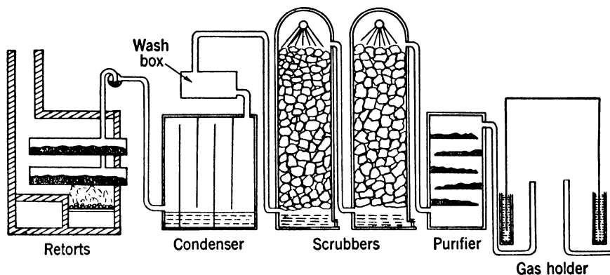
Figure 244. Coal Gas Plant
