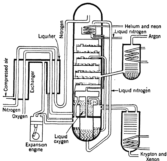
Figure 168. Diagram Showing the Parts of a Plant Designed to Separate the Different Constituents of Air
