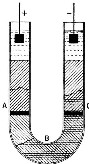
Figure 156. An Experiment to Demonstrate Differences in the Migration Velocities of Ions
