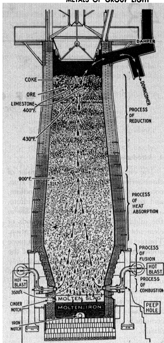
Figure 279. Cross Section Diagram of a Blast Furnace
