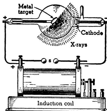
Figure 105. X-Ray Tube
