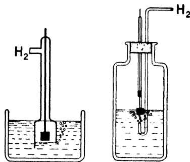
Figure 201. Hydrogen Electrodes
