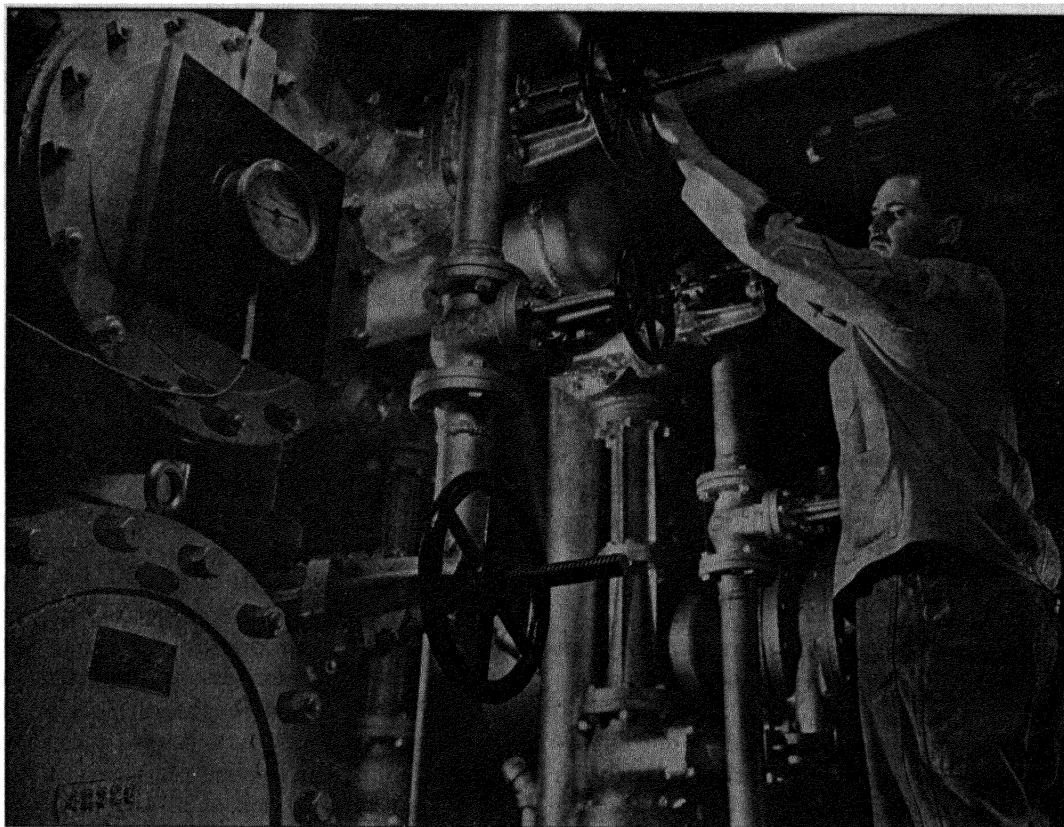
Figure 55. A Section of a Plant in Which Liquid Fats Are Converted into Solid Fats by Hydrogenation (Courtesy of Lever Brothers)
