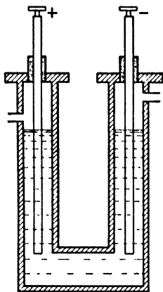
Figure 178. Electrolytic Cell for the Production of Fluorine
