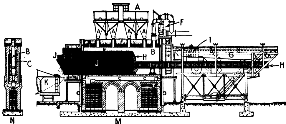
Figure 188. Cross-Section of a By-Product Coke Plant
