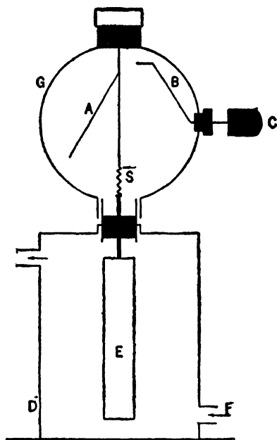
Figure 77. An Electroscope
