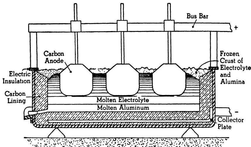
Figure 273. The Electrolytic Preparation of Aluminum (Courtesy of Aluminum Company of America)
