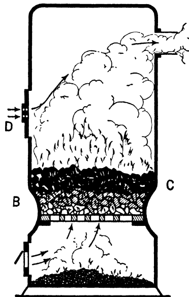
Figure 190. The Combustion of Coal At B, carbon burns to form \text{CO}_2 ; at C, carbon dioxide is reduced by hot carbon to \text{CO} .
