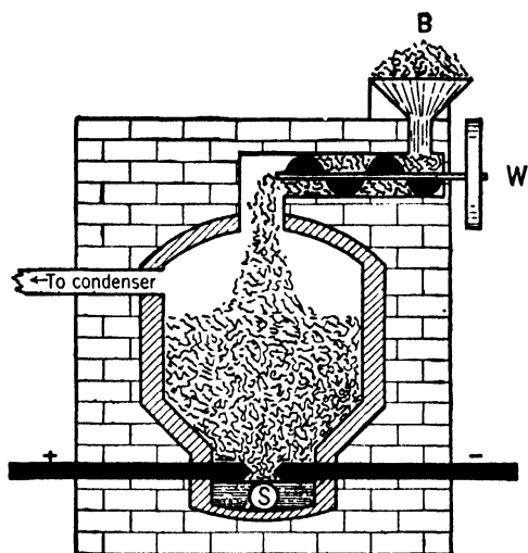
Figure 227. An Electric Furnace in Which Phosphorus is Produced
