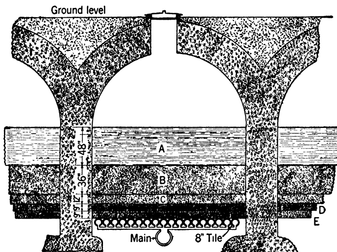
Figure 140. The Construction of a Filtration Bed A, water; B, fine sand; C, D, E, coarse sand and gravel.
