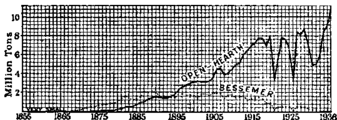
FIG. 184.—Production of steel. (1937, O.H., 119; B, 0·7; 1938, O.H., 94; B, 0·6.)
