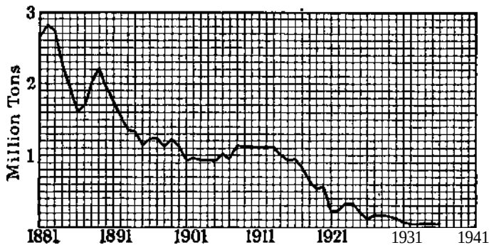
FIG. 182.—Production of wrought-iron. (1937, 0.08 mn. tons; 1938, 0.05 mn. tons.)
