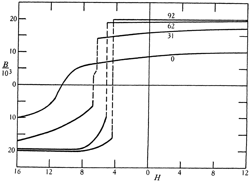
Fig. 7. Effect of tension on the hysteresis curves of material with positive magnetostriction. Ferronickel alloy, 15 per cent iron. The numbers on the curves give the tension in kg. per sq. mm. (Sixtus and Tonks, 1931.)
