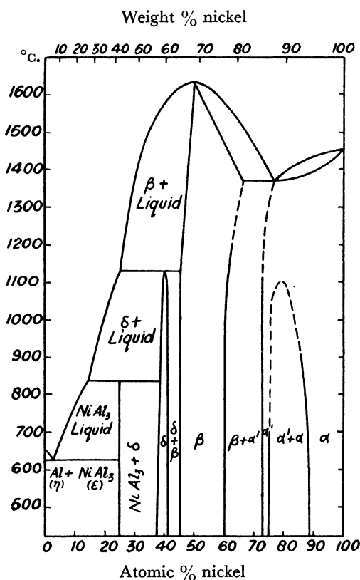
Fig. 1. The nickel-aluminium system. Reproduced by permission from the Proceedings of the Royal Society.
