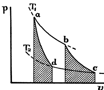
FIG. 19.—WORK UNDER THE ADIABATICS.
