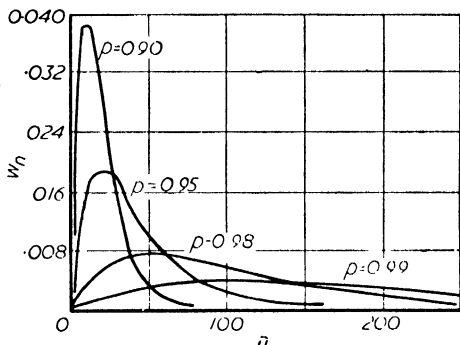
Figure 6. Molecular weight distribution for linear condensation polymers on a weight basis for several extents of reaction p (Reference : 17)
