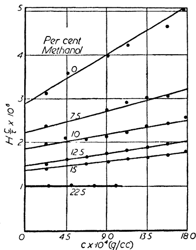
Figure 30. Reciprocal specific turbidity of polystyrene in benzene/methanol mixtures
