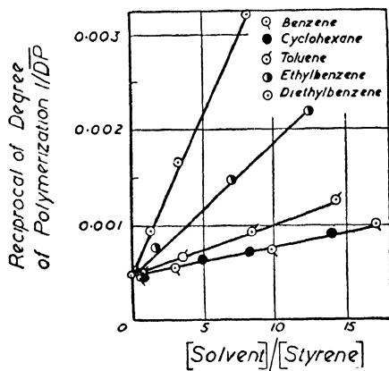
Figure 10. Effect of solvents on the degree of polymerization of styrene at 100°C (Reference : 38)
