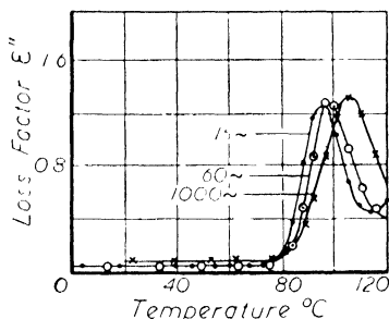
Figure 72. Effect of temperature on the loss factor of polyvinyl chloride at frequencies 15, 60, and 1,000 cycles/sec
