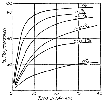
Figure 18. Effect of varying emulsifying agent concentration on the polymerization of 0.1 M aqueous solution of methyl methacrylate at 25°C
