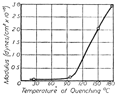
Figure 58. Hardness of polyamide quenched at various temperatures (Reference : 31)
