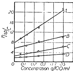
Figure 37. Plot of viscosity data for polystyrene fraction in several solvents: A toluene, B ethylene dichloride, C methyl ethyl ketone, D methyl ethyl ketone/isopropanol
