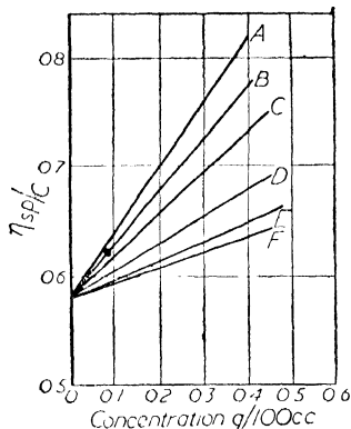
Figure 39. Effect of solvent composition on the viscosity of dilute solutions of polyvinyl acetate in ethyl acetate/dimethyl phthalate mixtures at 25°C: A 90% D.M.P., B 7% D.M.P., C 50% D.M.P., D 30% D.M.P., E 10% D.M.P., F 100% E.A.
