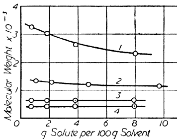
Figure 35. Effect of concentration on cryoscopic molecular weight of polystyrene fractions in benzene (Reference : 26)
