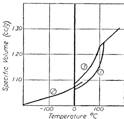
Figure 55. Specific volume of polyethylene. The curves refer to samples of different average molecular weights (Reference : 27)
