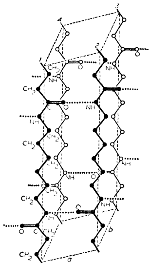
Figure 53. Molecular structure of polyhexamethylene diamine (Nylon 66) (Reference : 26)
