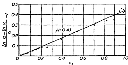
Figure 22. Determination of \mu for rubber/benzene system at 25°C from data of Gee and Treloar (Reference : 4d)
