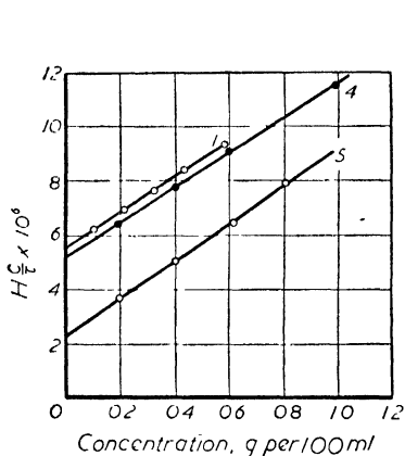
Figure 29. Turbidity data for polystyrene fractions in methyl ethyl ketone. Molecular weight by light scattering 1. 178,000, 4. 190,000, 5. 445,000 (molecular weight by osmotic pressure of fraction 1: 172,000)
