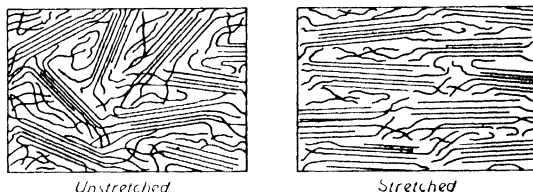
Figure 59. Two-dimensional representation of structure of crystalline polymer
