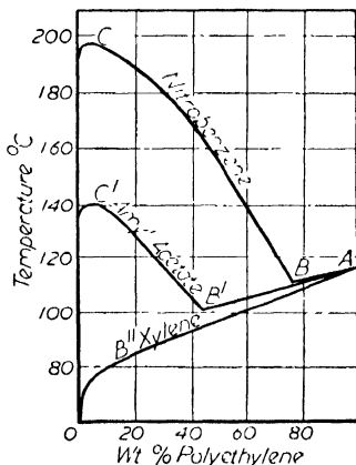
Figure 24. Solubility curves for polyethylene in nitrobenzene, amyl acetate, xylene (Reference : 11)
