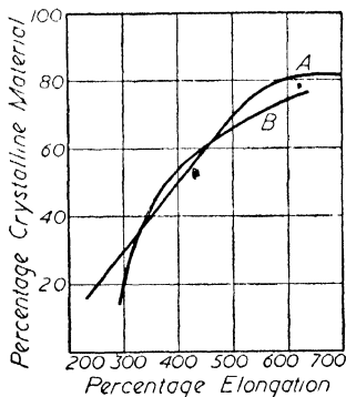
Figure 57. X-Ray determination of crystalline material: A unvulcanized, B vulcanized, rubber (Reference : 29)
