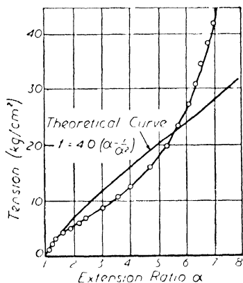
Figure 66. Extension in one direction for rubber (8% sulphur) at 20°C (Reference : 20b)
