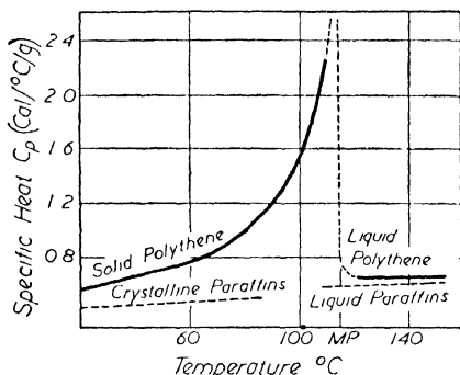
Figure 56. Specific heat of Polythene (Reference : 27)
