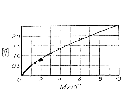
Figure 41. Dependence of intrinsic viscosity on molecular weight for polyisobutylene fractions in diisobutylene at 20°C. [\eta]_\infty = 3.60 \times 10^{-4} and \beta = 0.64 .
