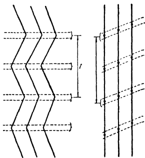
Figure 63. Possible scheme of chain unkinking accompanying elongation of substituted polyamides and other rubber-like materials
