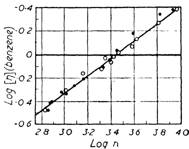
Figure 42. Relation between chain length (determined by osmotic pressure measurements) and intrinsic viscosity for sharp fractions of polymethyl methacrylate
