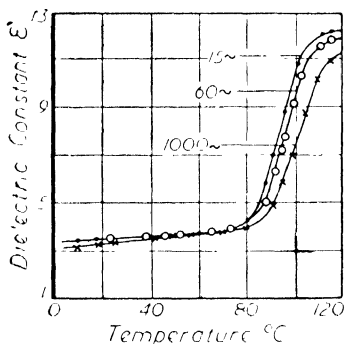
Figure 71. Effect of temperature on the dielectric constant of polyvinyl chloride at frequencies 15, 60, and 1,000 cycles/sec
