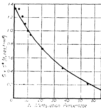
Figure 60. Dependence of Young's modulus G on the molar proportions of N-methylation for polydecamethylene sebacamides
