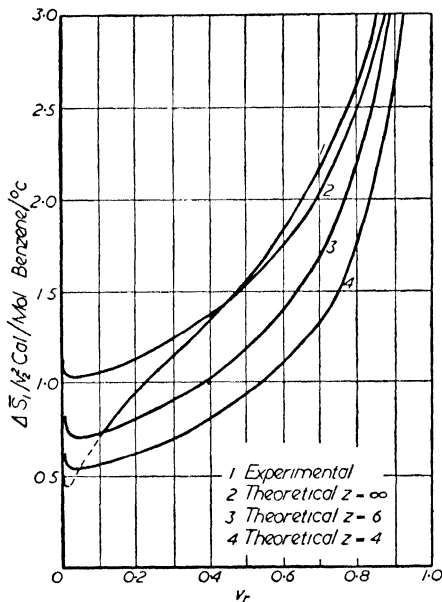
Figure 21. Entropy of dilution of rubber by benzene
