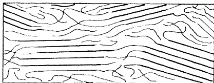
Figure 54. Arrangement of chain molecules in 'crystalline' polymer. Heavy lines represent crystalline regions. Chains pass through crystalline and amorphous regions
