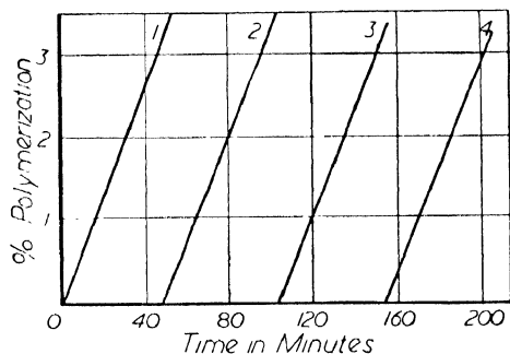
Figure 9. Inhibition of photopolymerization of vinyl acetate by benzoquinone
