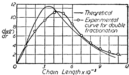
Figure 14. Comparison of theoretical and experimental differential weight distributions for polymethyl methacrylate (Reference : 46)
