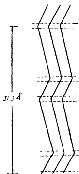
Figure 52. Possible diagrammatic form of chain folding along fibre axis of polytrimethylene sebacate (Reference : 22b)
