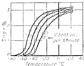
Figure 70. Deformation/temperature curves of natural rubber (3% sulphur) at various frequencies (Reference : 26)
