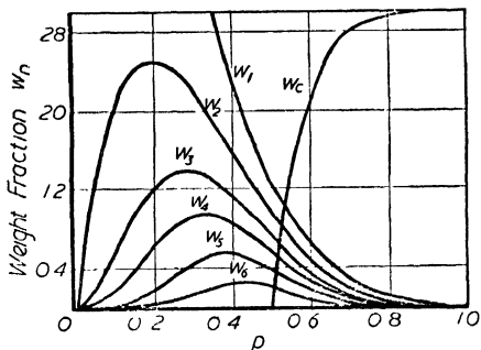
Figure 8. Weight fractions of various species in a trifunctional condensation as a function of \alpha , which in this case equals the extent of reaction p . w_c is the weight fraction of the gel. (Reference : 2)
