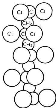
Figure 47. Suggested chain configuration for polyvinylidene chloride (Reference : 15)
