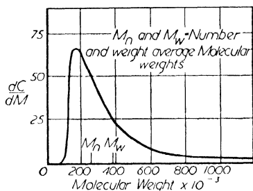
Figure 32. Frequency distribution dC/dm in relative coordinates of nitrocellulose fraction calculated directly from sedimentation measurements (Reference : 18)
