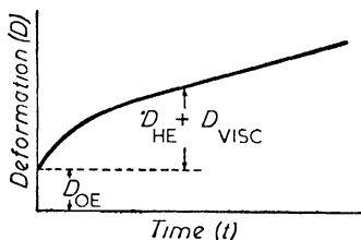
Figure 68. Deformation/time curve for constant stress
