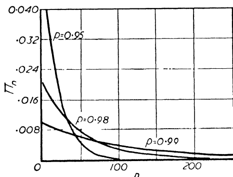
Figure 5. Molecular weight distribution for linear condensation polymers on a number basis for several extents of reaction p . Mol fractions \Pi_n versus number of structural units n (Reference : 17)
