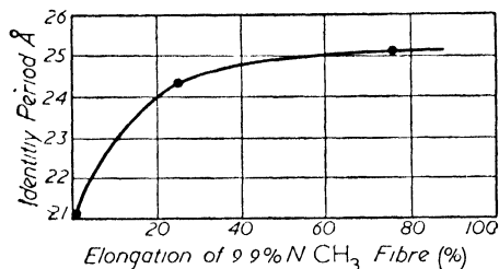
Figure 62. Change in identity period caused by stretching fibre of 9.9% N CH 3 polydeca-methylene sebacamide
