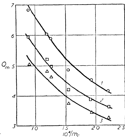
Figure 26. Effect of cross linking of rubber on swelling capacity in good solvents
