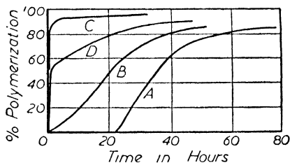
Figure 16. Polymerization of acrylonitrile in aqueous solution at 20°C
