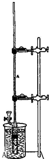
FIG. 20. Osmotic pressure cell
