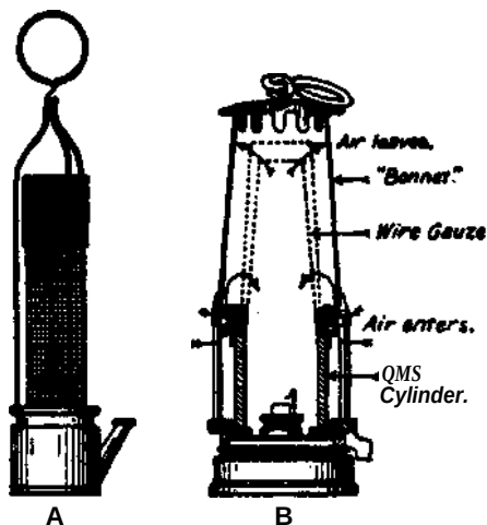
FIG. 2. Safety-lamps, old and new
