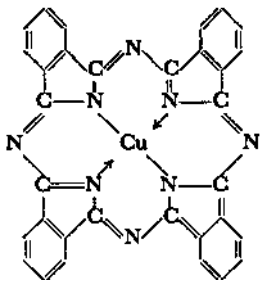
FIG. 16. Graphic formula of Monastrol Blue
