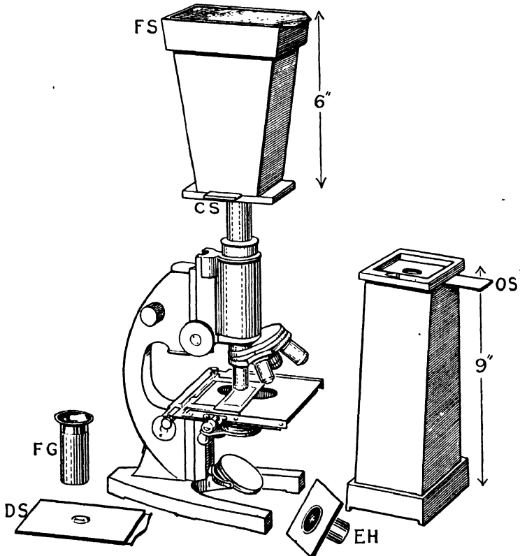
FIG. 3.—Home made box cameras, 9 in. model unmounted, 6 in. model mounted on microscope. FS, focussing screen. CS, closed shutter. OS, open shutter. FG, focussing glass. DS, dark slide. EH, eyepiece holder to be inserted in top of unmounted camera before mounting.
