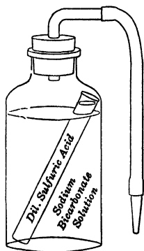
Fig. 33. Simple form of chemical fire extinguisher.
