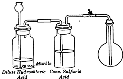
Fig. 45. Filling a flask with dry carbon dioxide.
