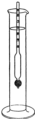
Fig. 77. Finding the density of gasolene.
