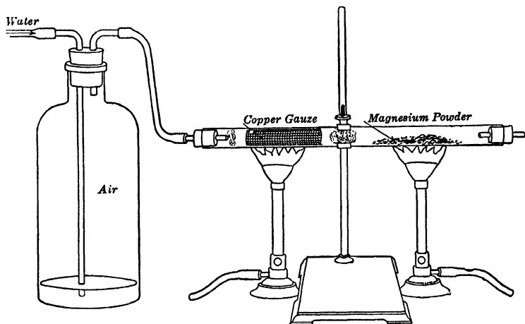
Fig. 37. Passing air over hot copper and magnesium.
