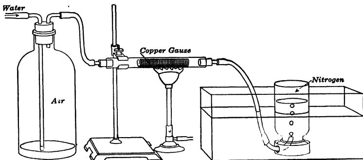
Fig. 36. Passing air over hot copper.
