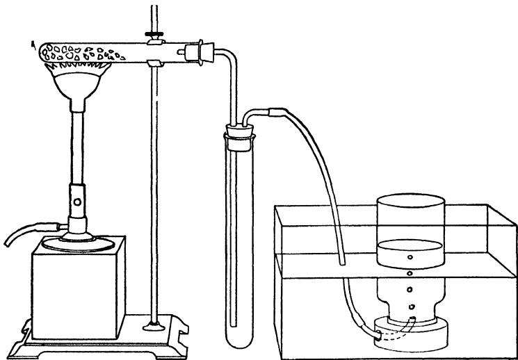
Fig. 72. Destructive distillation of coal.
