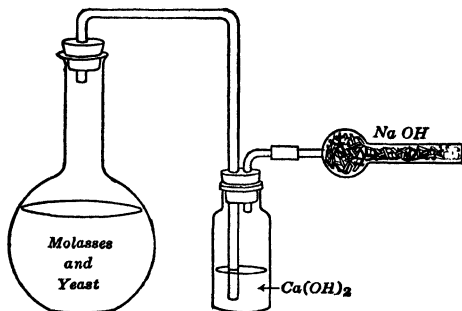
Fig. 80. Fermentation of molasses in the laboratory.
