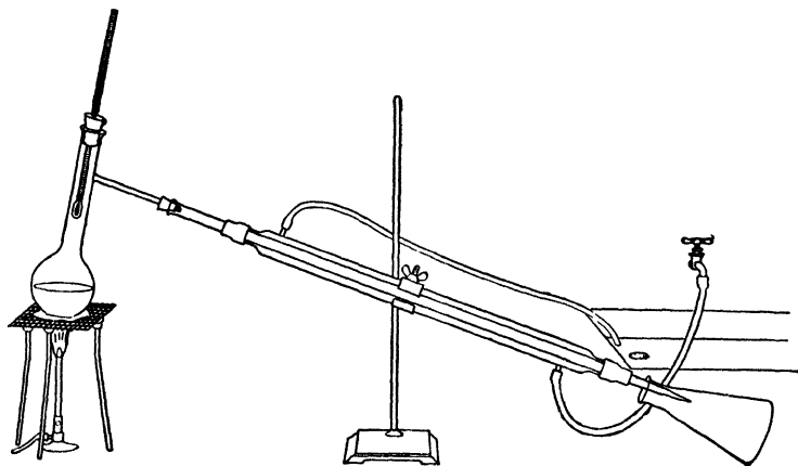
Fig. 81. Fractional distillation of alcohol.
