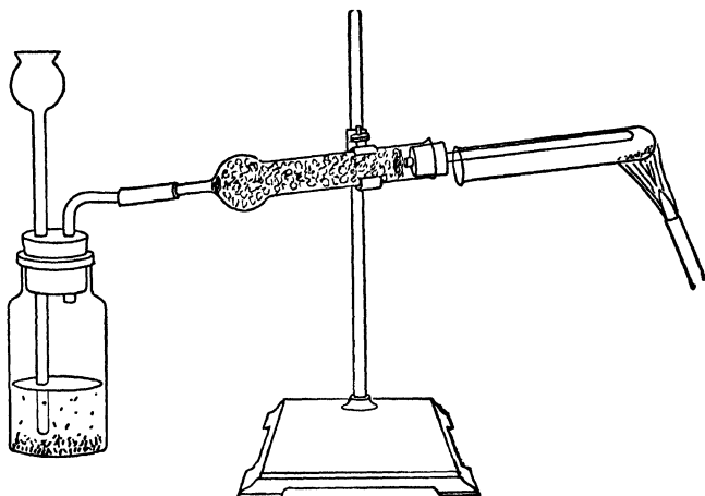
Fig. 26. Reducing copper oxide with dry hydrogen.
