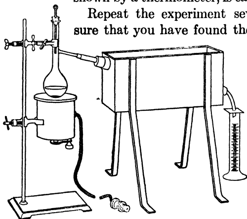
Fig. 79. Finding the boiling point and dry point of gasoline.
