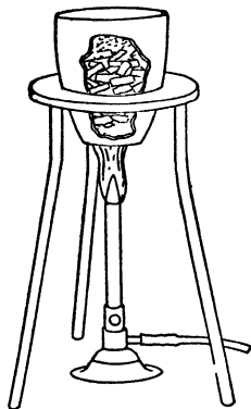
Fig. 75. Preparation of charcoal in a sand crucible.
