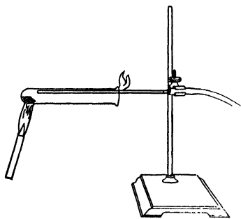
Fig. 46. Reducing copper oxide to copper with illuminating gas.
