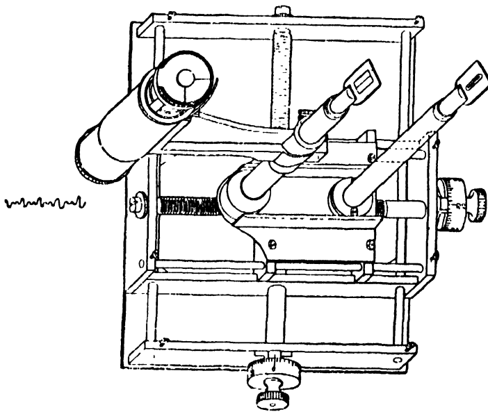
FIG. 45.—Coordinate measurer.
