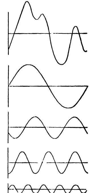
FIG. 71.—Curve with its sinusoid components.
