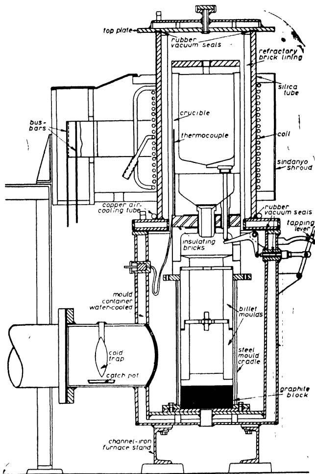
Fig. 5—High Frequency Vacuum Furnace
