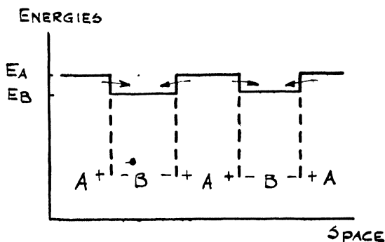
Figure 8.—Electronic rearrangement, due to a difference in electronegativity, in an intermetallic compound
