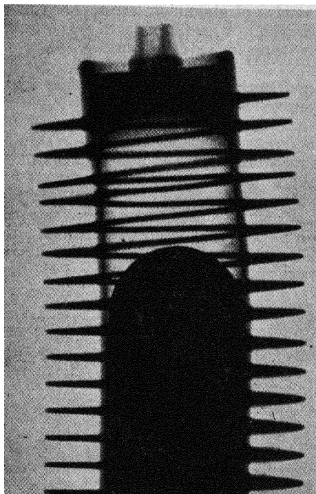
Fig 20. —Effect of ratchetting in experimental Calder Hall can.
