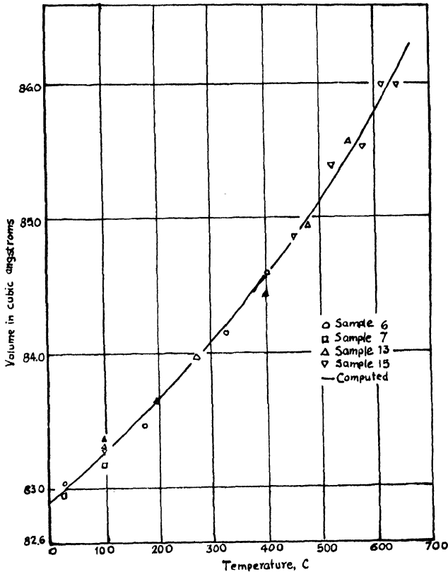
Fig. 17—Volume of \alpha uranium as a function of temperature.
