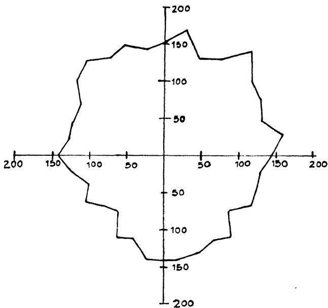
Fig. 8—Radial intensity of the (002) reflection from a 3/4" round uranium rod rolled with hand round pass rolls. (Cu K \alpha radiation, using 0.2° geiger tube slit and 0.4° x-ray tube slit.)
