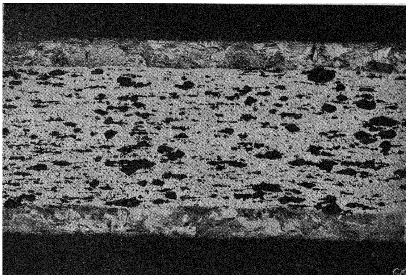
Figure 9. —Cross section of a fuel plate fabricated by the “picture frame” technique. Core : \text{UO}_2 in stainless steel. Cladding : stainless steel. (Mag. 100x). (Courtesy : Nuclear Development Corporation)
