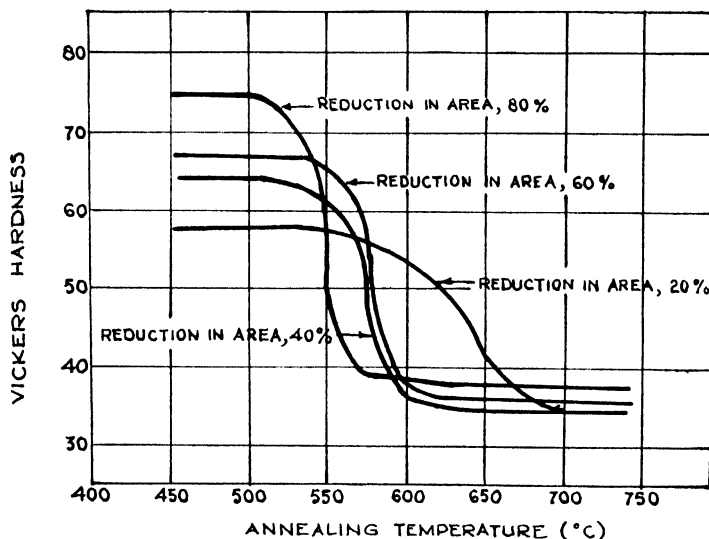
Fig. 5.—Effect of cold work on recrystallisation of iodide thorium (7). (Soaking time—1 hour)
