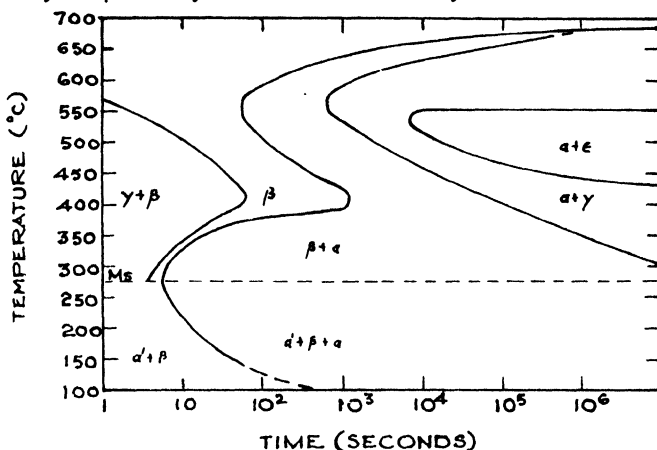
Fig. 29—Isothermal transformation diagram, of 0.5 w/o Mo-U.
