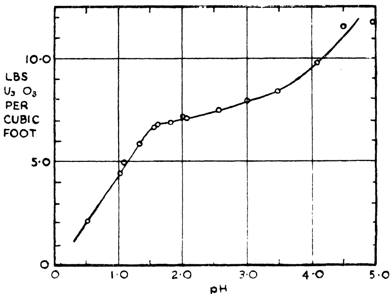
Figure 2.—The absorption of uranium from pure solution by de-acidite FF
