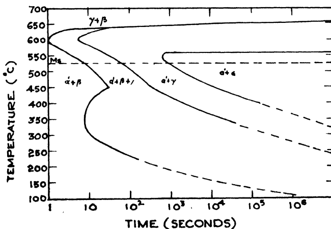
Fig. 30—Isothermal Transformation diagram of 1.0 w/o Mo-U.
