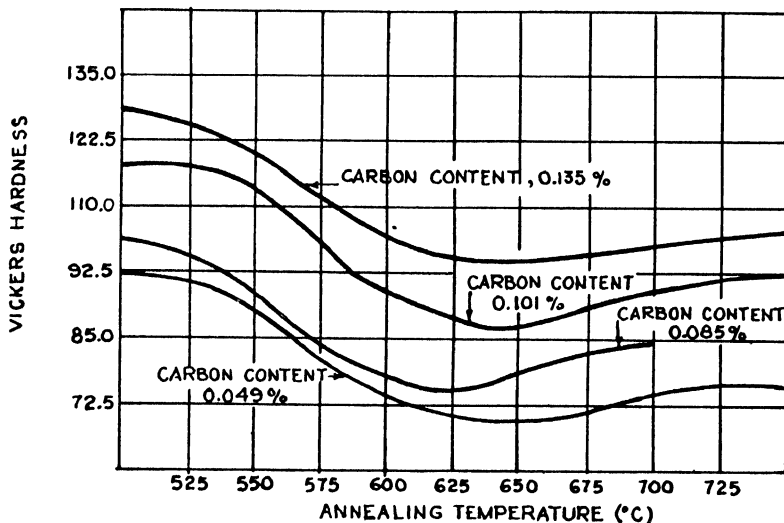
Fig. 8.—Effect of carbon on recrystallisation of thorium (10) Annealing time one hour. The specimens were made from ingots reduced 35% in area and homogenised for 12 hours at 1275°C
