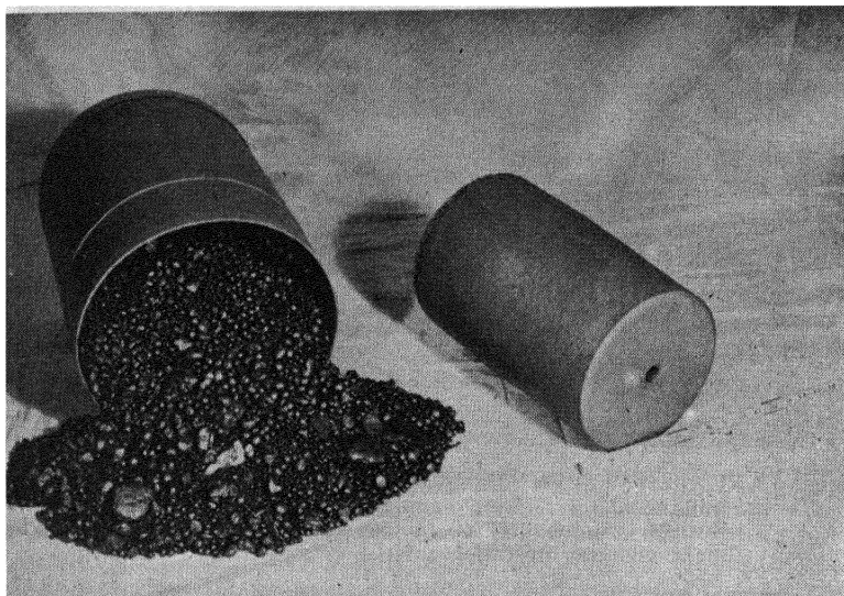
Fig. 14 —Pure Beryllium Pebbles, left, and Nuclear Grade Vacuum Cast Ingot.
