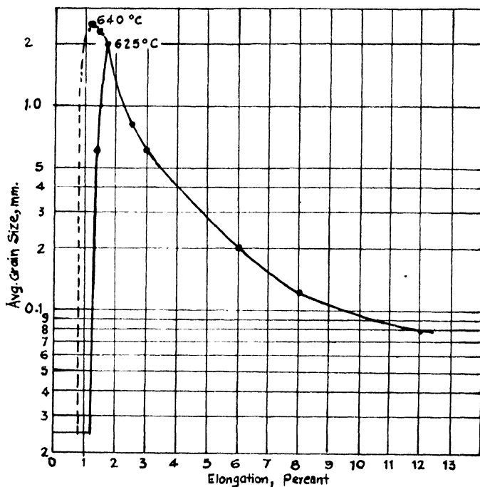
Fig. 15—Grain Size Vs. Strain in Impure Uranium. Increase of grain size with decreasing strain in elongated, tapered tensile bar annealed by heating at 5°C per hour to 625°C (solid line), and subsequently heated at 640°C for 45 hours (dotted line).
