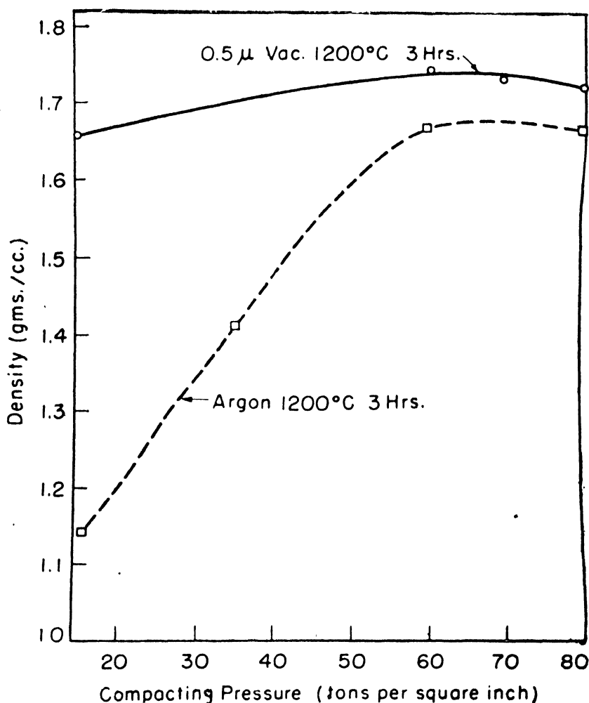
Figure 12. —Density of -200 mesh beryllium powder vs. compacting pressure, as compacted, as sintered in argon and in vacuo
