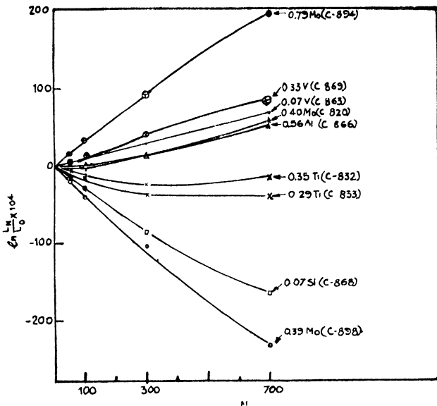
Fig. 19—Growth of specimens quenched from 710°-725°C.
