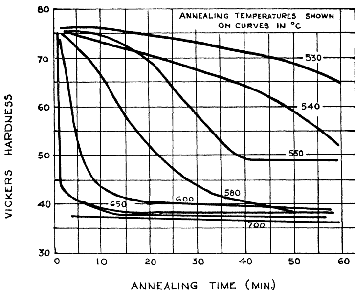
Fig. 4.—Isothermal recrystallization curves for iodide thorium* (Specimens cold worked to 80% R. A.)
