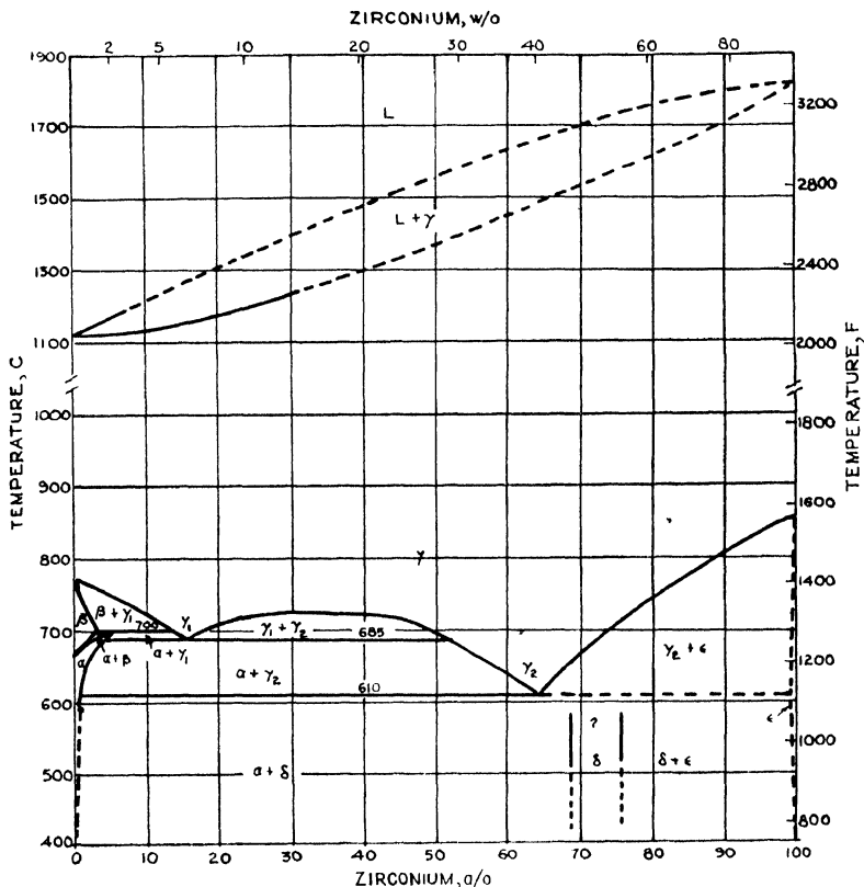
Fig. 23—Uranium-zirconium system
