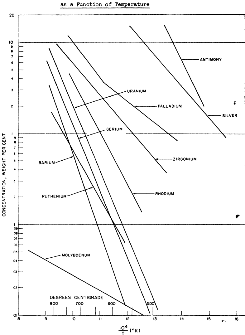
Fig. 1 —Individual Solubilities of Uranium, Cerium, Barium and Noble Metal Fission Product Elements in Zinc as a Function of Temperature
