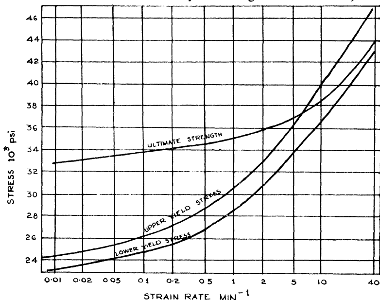
Fig.2.—Variation of strength properties of thorium sheet, parallel to rolling direction, with strain rate (8).
