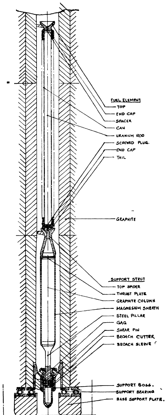
Fig. 12.—Graphite and fuel element support.
