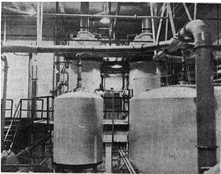
Fig. 10—Continuous Salting Evaporators. Automatic controls visible between evaporators. Continuous centrifuge at lower left corner. Evaporators operate at 2" Hg absolute pressure, with 6,000 lb. per hour evaporation rate each.
