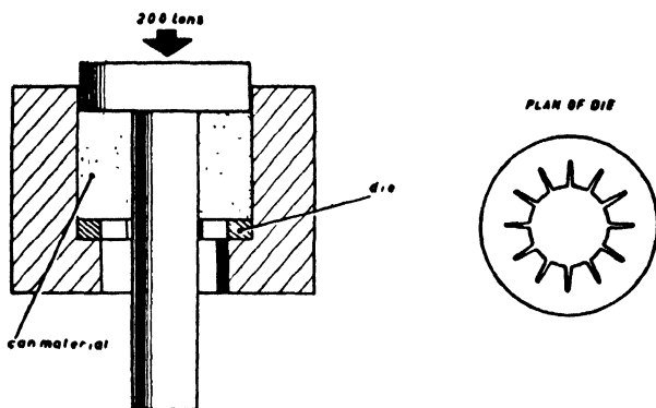
Fig. 16—Bepo type finned cans are made by impact extrusion. The Helical Twist in the fins is usually done later in a lathe.
