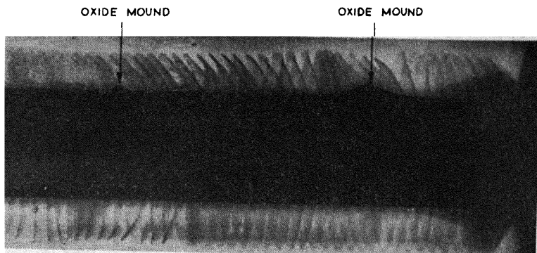
Fig. 24—Radiograph of Failed Calder Hall Cartridge.
