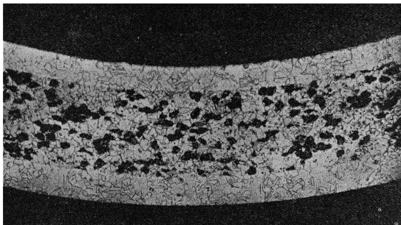
Figure 11. —Tubular fuel element. Core: Approx. 20 w/o UO 2 in stainless steel. Cladding: stainless steel. (Mag. 100x) (Courtesy: Martin Company)
