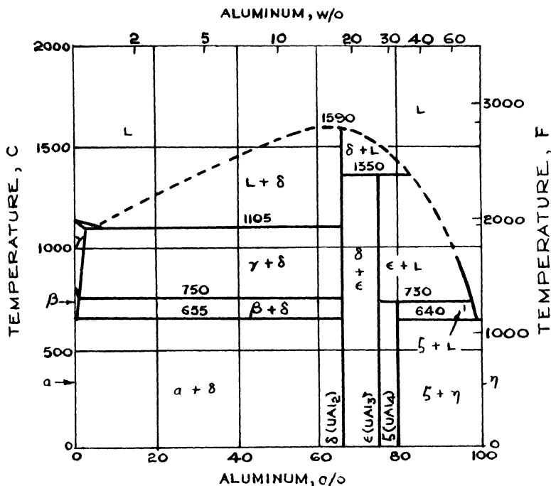
Fig. 27—Uranium-aluminum system
