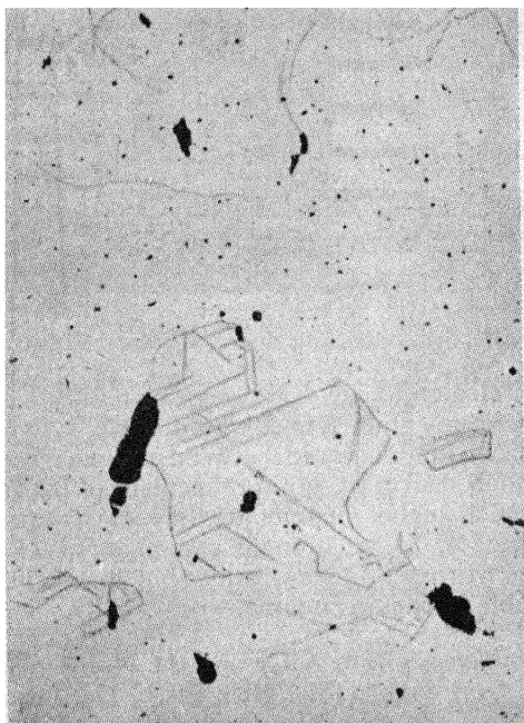
Fig. 21—Cavitation produced by creep strain in Magnesium Alloy.
