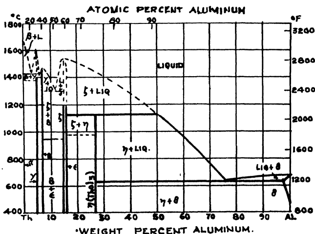
Fig. 9. —Thorium-Aluminium System
