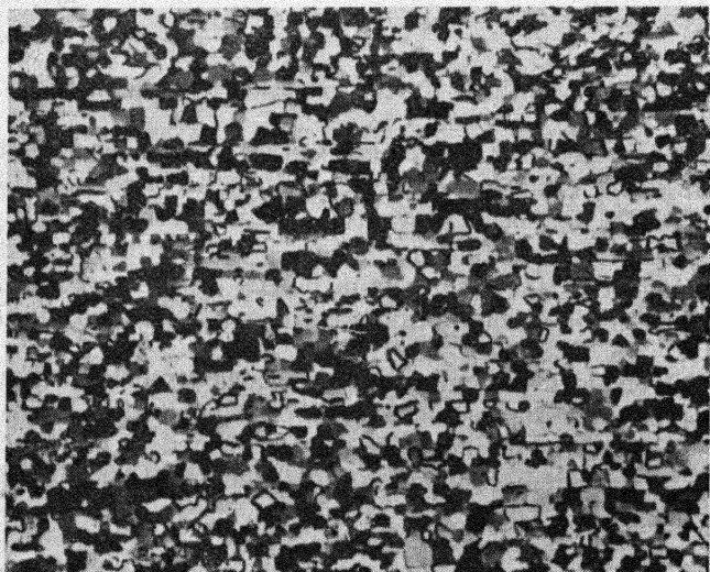
Figure 2. Specimen 3. Extrusion (6855) x 150
