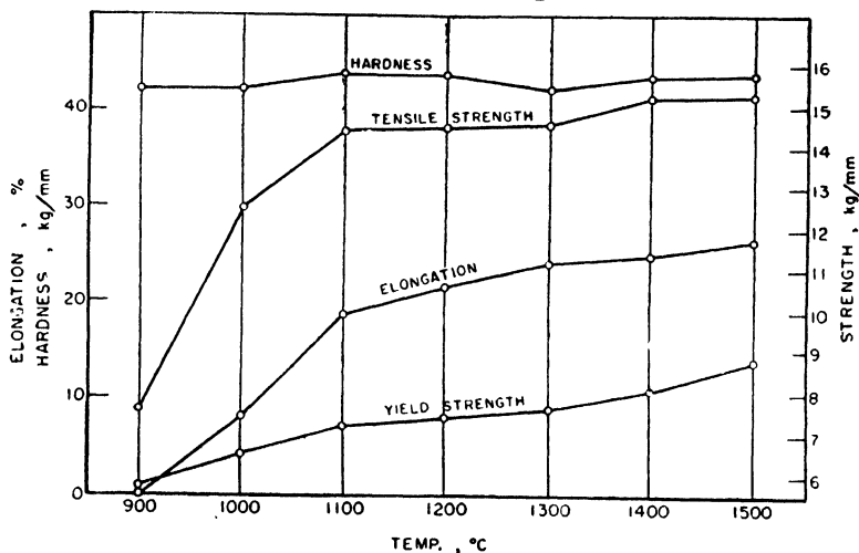
Figure 5.—Effect of sintering temperature on the mechanical properties of electrolytic thorium powder compacts, sintered at various temperatures. (According to G. A. Meerson)
