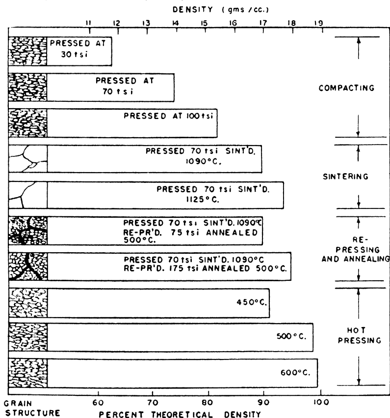
Figure 3.—Density and grain structure of uranium produced by various powder metallurgical treatments
