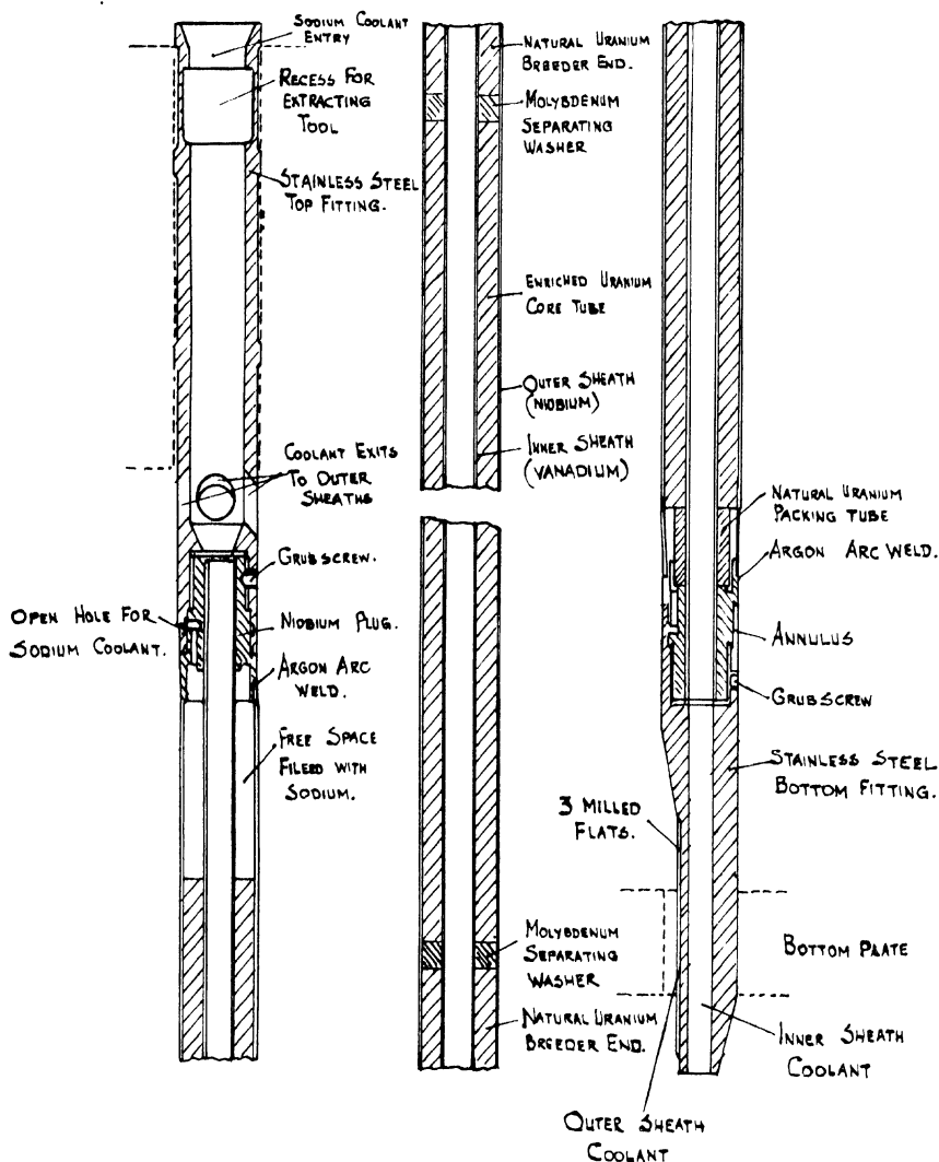
Fig. 25—The Dfr fuel element.
