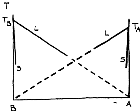
Figure 11.—Liquidus L and solidus S for large size factors
