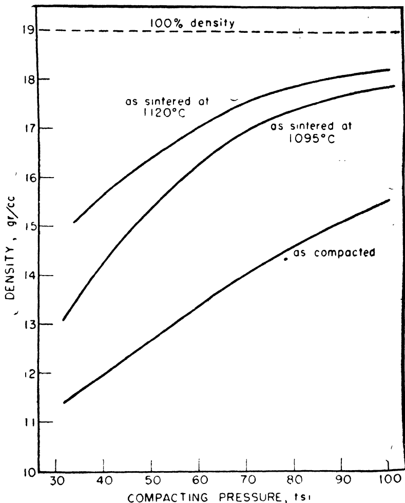
Figure 2. —Effect of compacting pressure on the density of a "green" and sintered uranium powder compact
