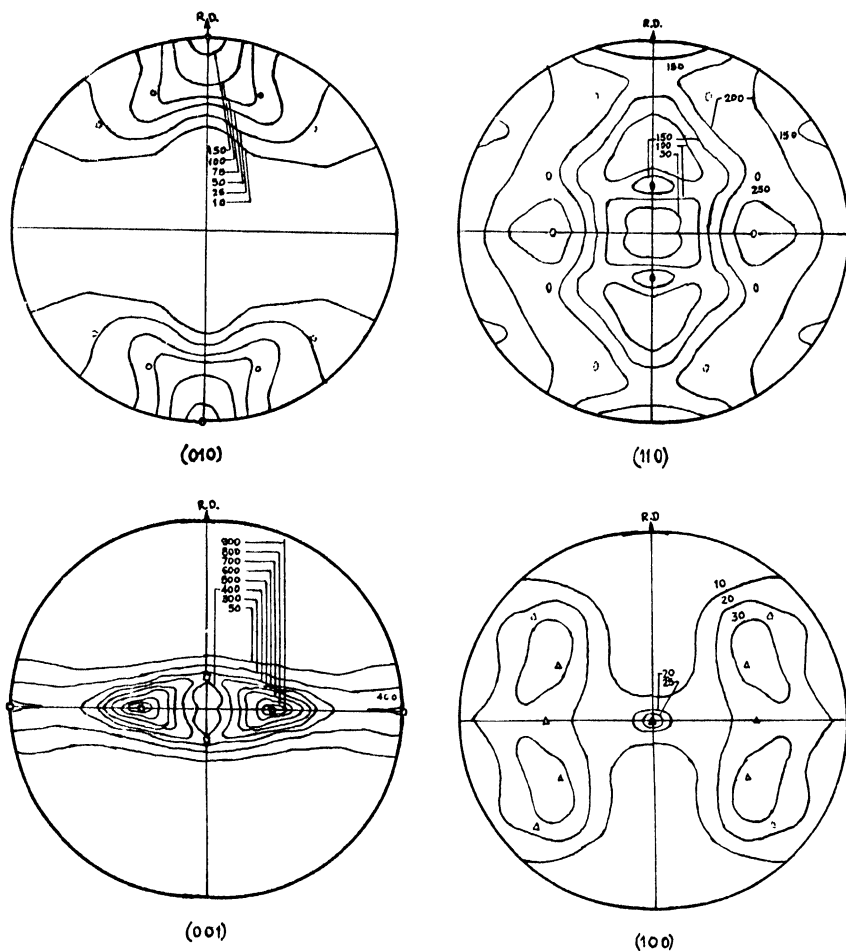
Fig. 11—Pole figures for Uranium Sheet 300°C rolled and recrystallized.
