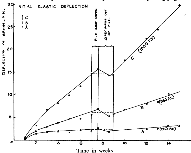
Fig. 11—Creep of uranium springs during irradiation ( 13 \times 10^{12} thermal neutrons per sq. cm. per sec.) at 100^\circ\text{C} . The stress valves refer to mean skin stresses.
