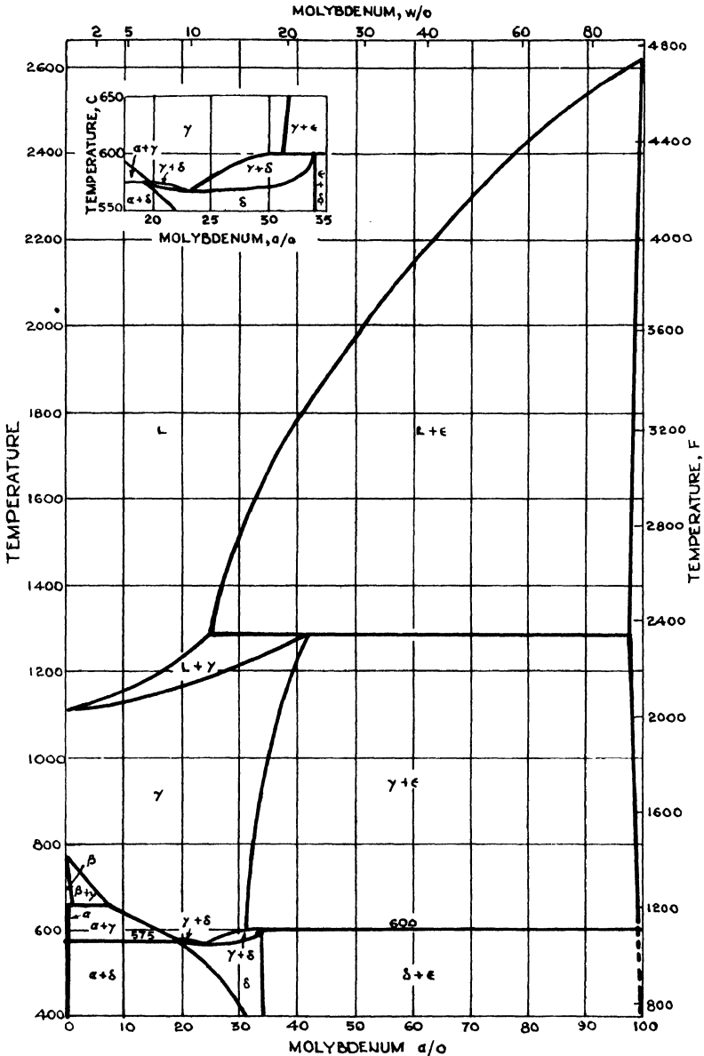
Fig. 26—Uranium-Molybdenum system
