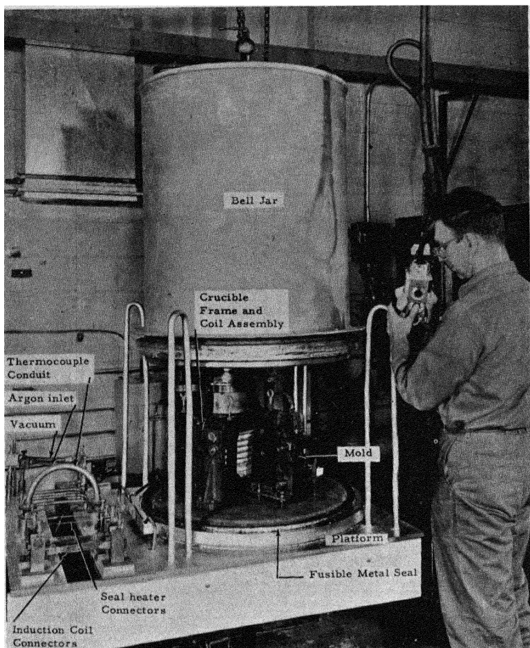
Fig. 8—Uranium Melting Furnace—Bell Jar Partially Removed.
