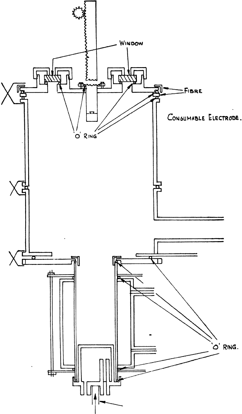
Fig. 4 —Consumable electrode vacuum arc melting furnace.
