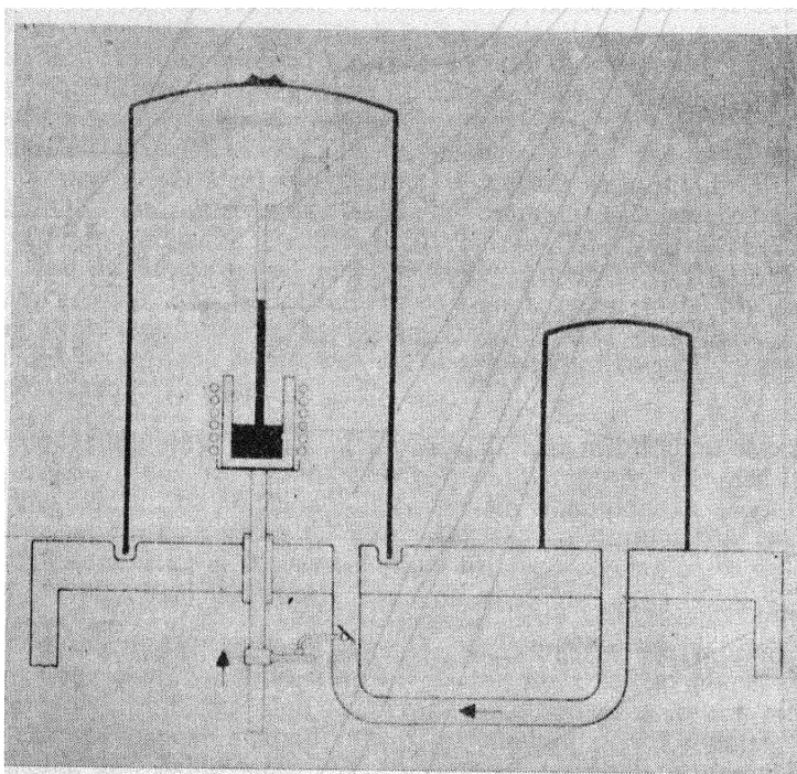
Fig. 2—Injection Casting Furnace
