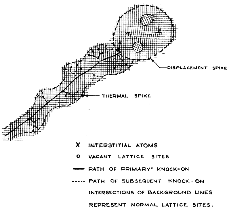
Fig. 20—Schematic diagram of situation resulting from passage of energetic knock-on atom through a solid.
