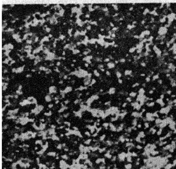
Fig. 14e. —100X. 90% total reduction in area at 300°C in five steps (15%, 30%, 30%, 48% and 48%) with intermediate recrystallization. Final anneal one hour at 475°C
