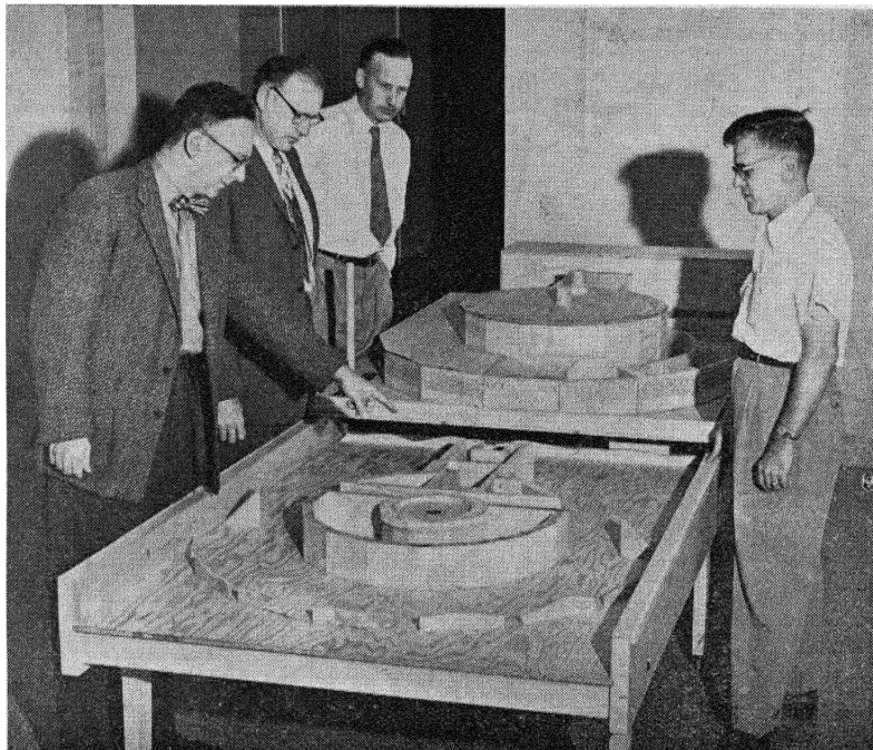
Fig. 6—EBR—II Process Building Model
