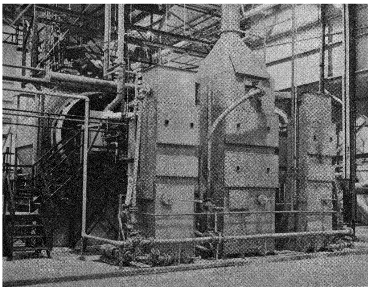
Fig. 4 —Sulphating Mill at left. Sodium Carbonate Scrubbing Towers in foreground.
