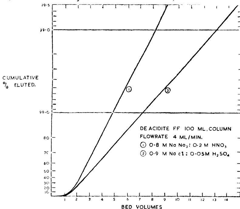
Figure 11.—Elution rate.
