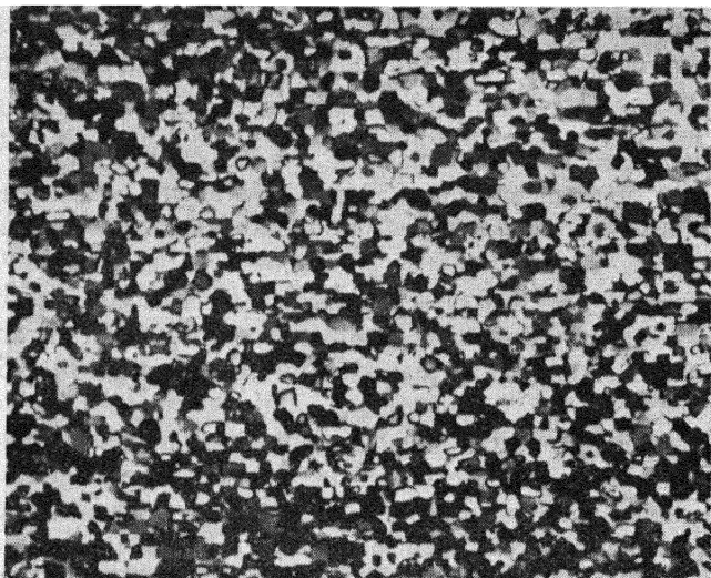
Figure 2. Specimen 1. Extrusion of Zr tube M 919 (6854) x 150
