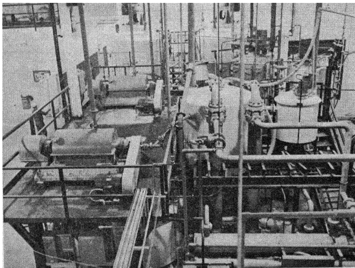
Fig. 7 —Alum Crystallizer and Continuous Centrifuge in foreground. Beryllation kettle and hydrolizer behind crystallizer, with beryllium hydroxide centrifuge at left. Production capacity of this equipment is approximately 1,000 lb. of beryllium per day. Large tanks in background are ammonium beryllium fluoride solution storage tanks.
