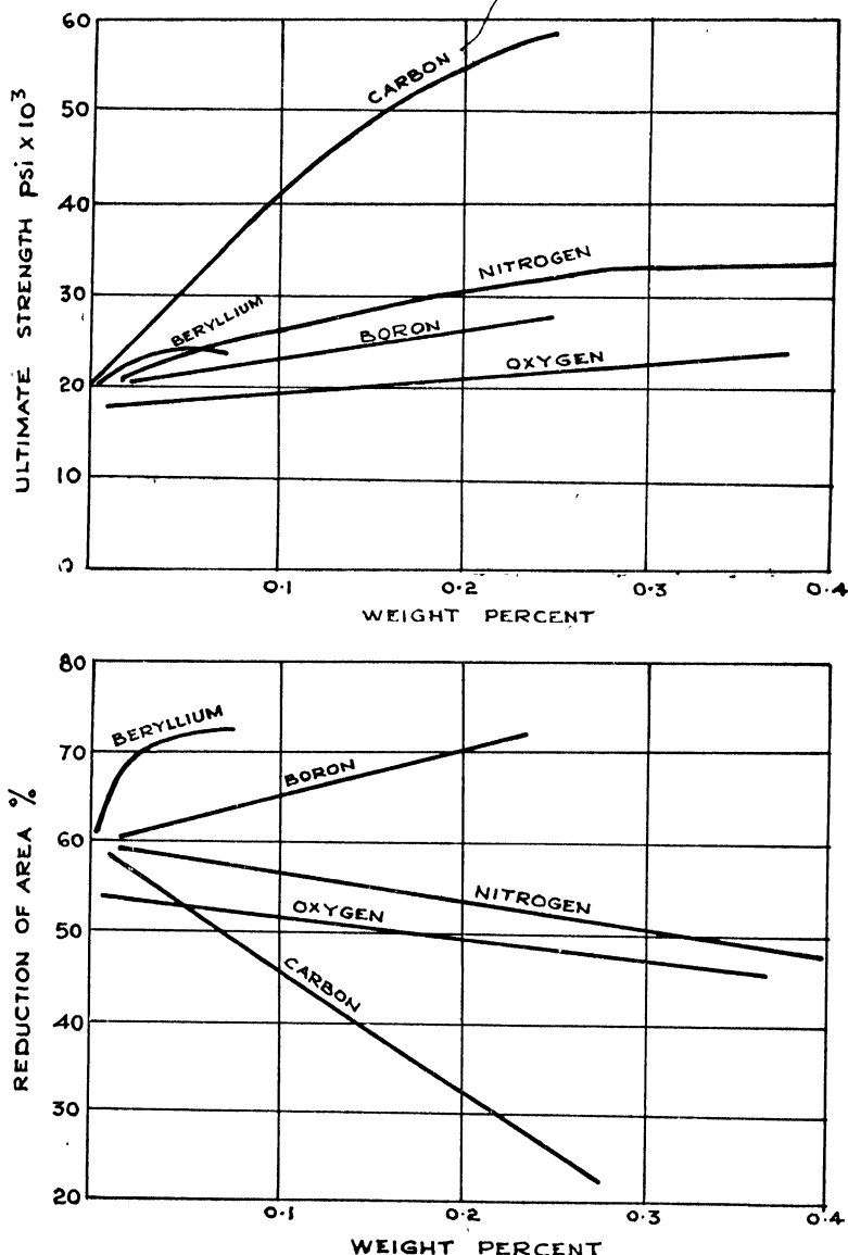
Fig. 7.—Effect of carbon, oxygen, nitrogen, beryllium and boron on the strength and ductility of iodide thorium a
