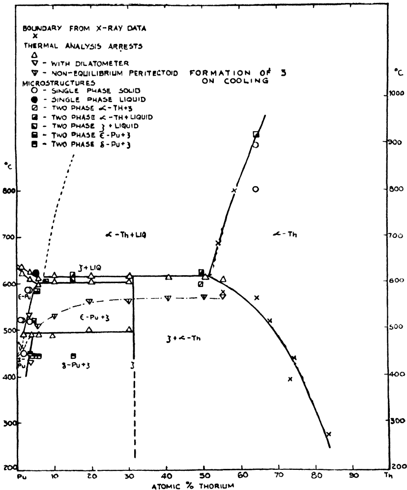
Fig. 7.—The plutonium—thorium equilibrium diagram
