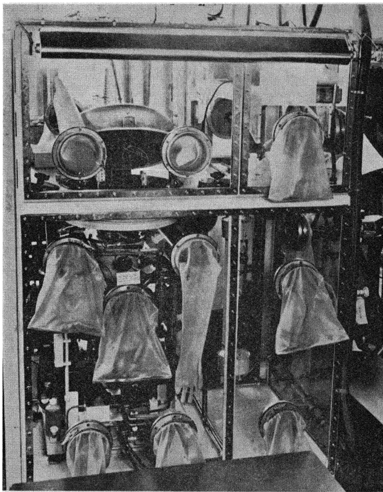
Fig. 1.—Typical glove box at Harwell; note upper working space and lower compartment for pumping equipment
