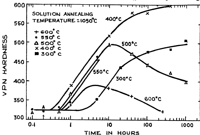
Fig. 32—Hardness data for an isothermally transformed U-10 wt % Nb Alloy.
