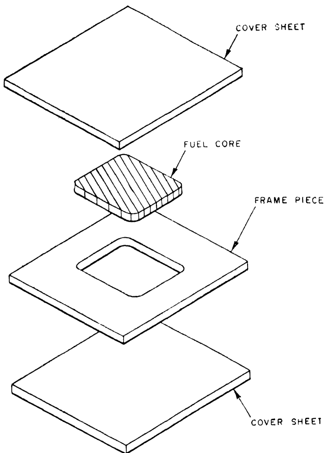
Figure 8. —Exploded view showing make up of composite fuel plate prior to rolling
