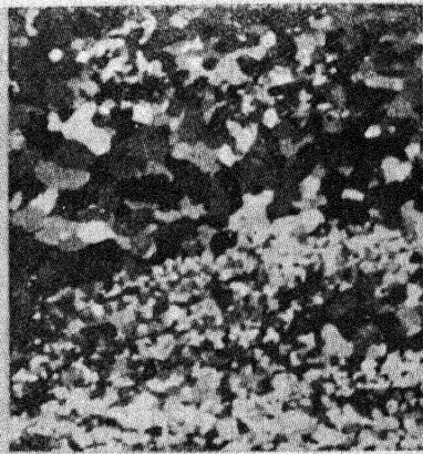
Fig. 14d. —100X. High purity rod, 90% reduction in area at 300°C, annealed two hours at 525°C
