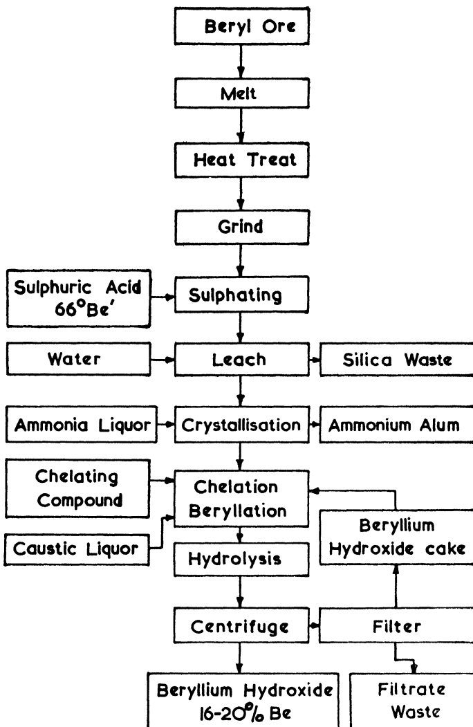
Fig. No. II—Beryllium Hydroxide Production Brush Process.
