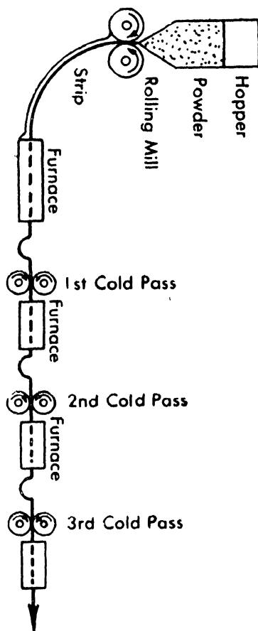
Figure 20. —Flow diagram for production of strip from metal powder
