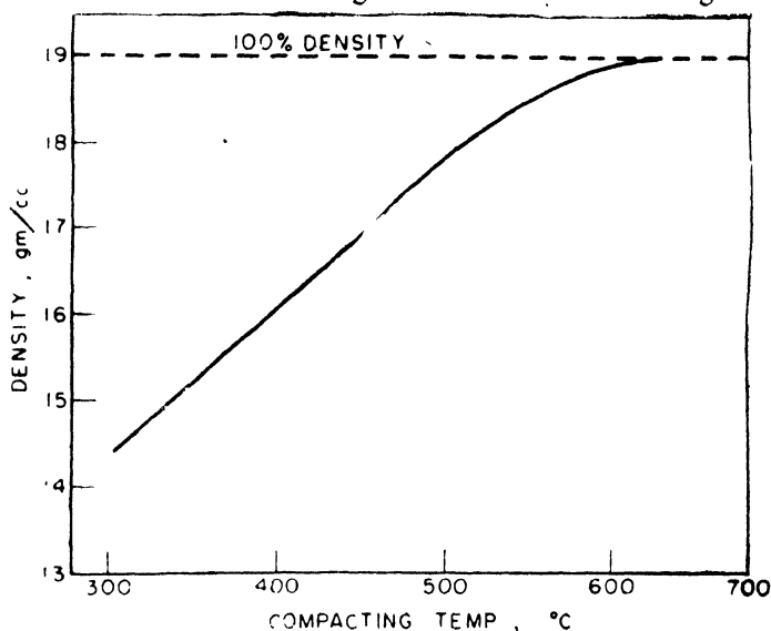
Figure 4. —Density of hot compacted uranium powder vs. compacting temperature (20 tsi)
