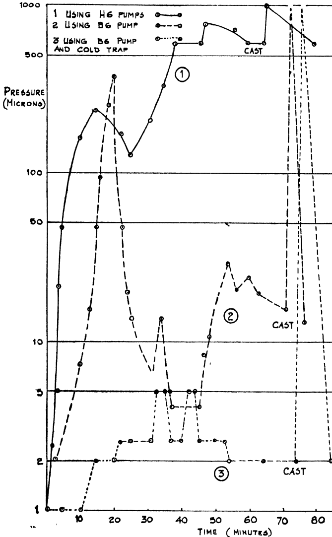
Fig. 6—Time pressure relationship of bar casting furnace. (AERG M[R 697)
