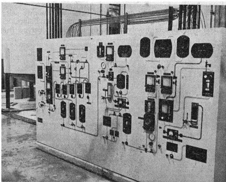
Fig. 6 —Hydroxide Plant Control Panel. All chemical operations in manufacture of beryllium hydroxide are controlled from this panel.
