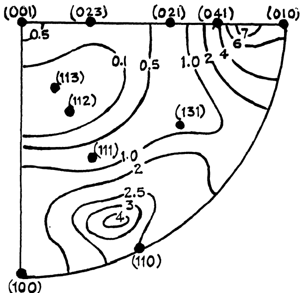
Fig. 5—Preferred Orientation plot for alpha extruded Uranium Rod, as extruded.
