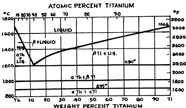
Fig. 14.—Thorium-titanium system
