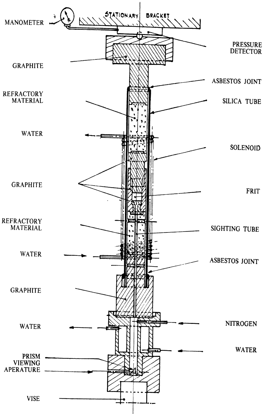
Figure 1.—Sintering Equipment
