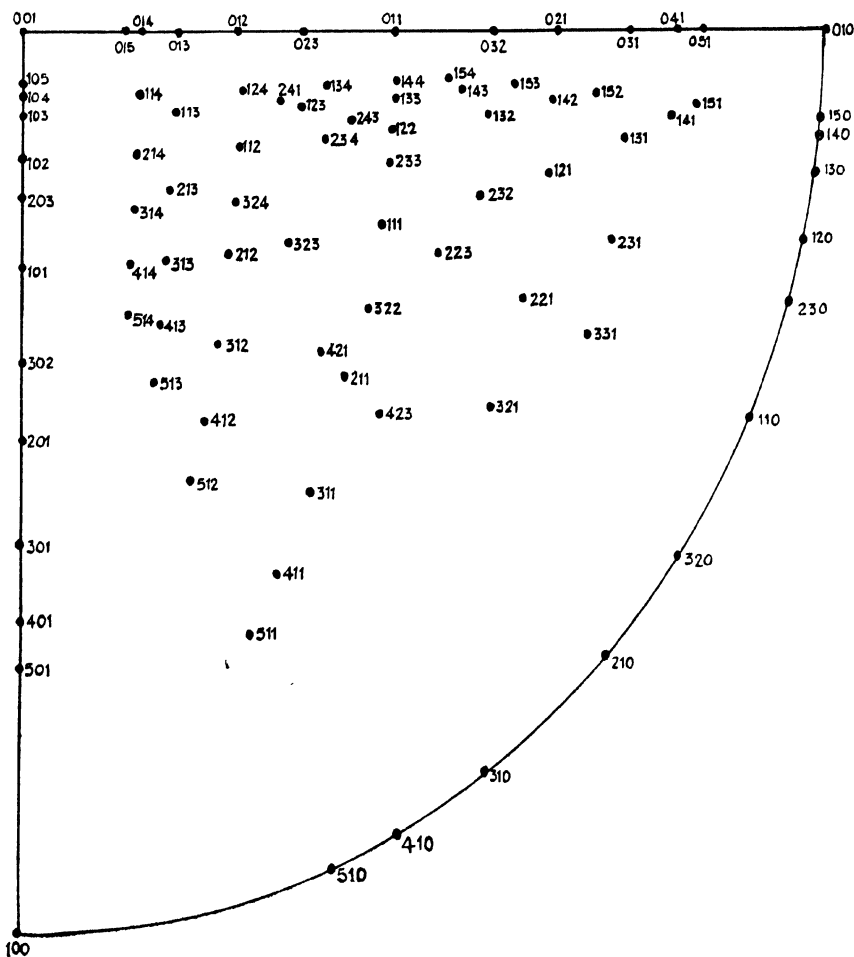
Fig. 6b—(001) standard projection of Alpha-uranium lattice directions.
