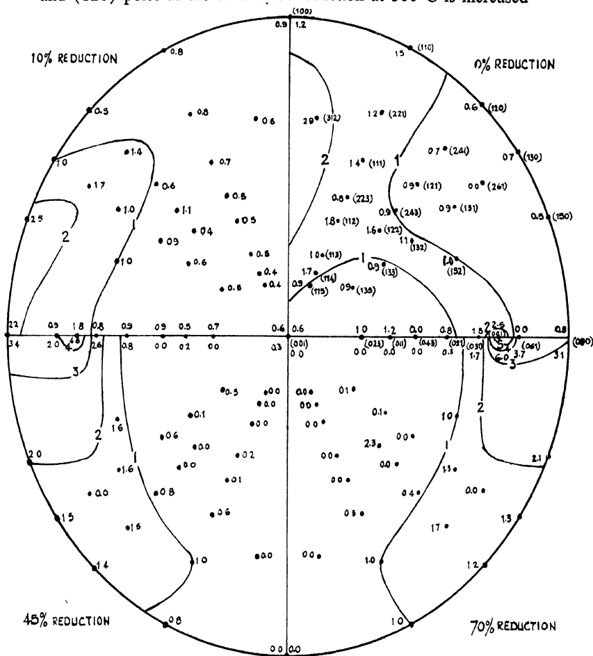
Fig. 4—Inverse pole figure of uranium rods rolled at 300°C. (0,10,45 and 70% reductions) Initial condition—water quenched from the beta phase.
