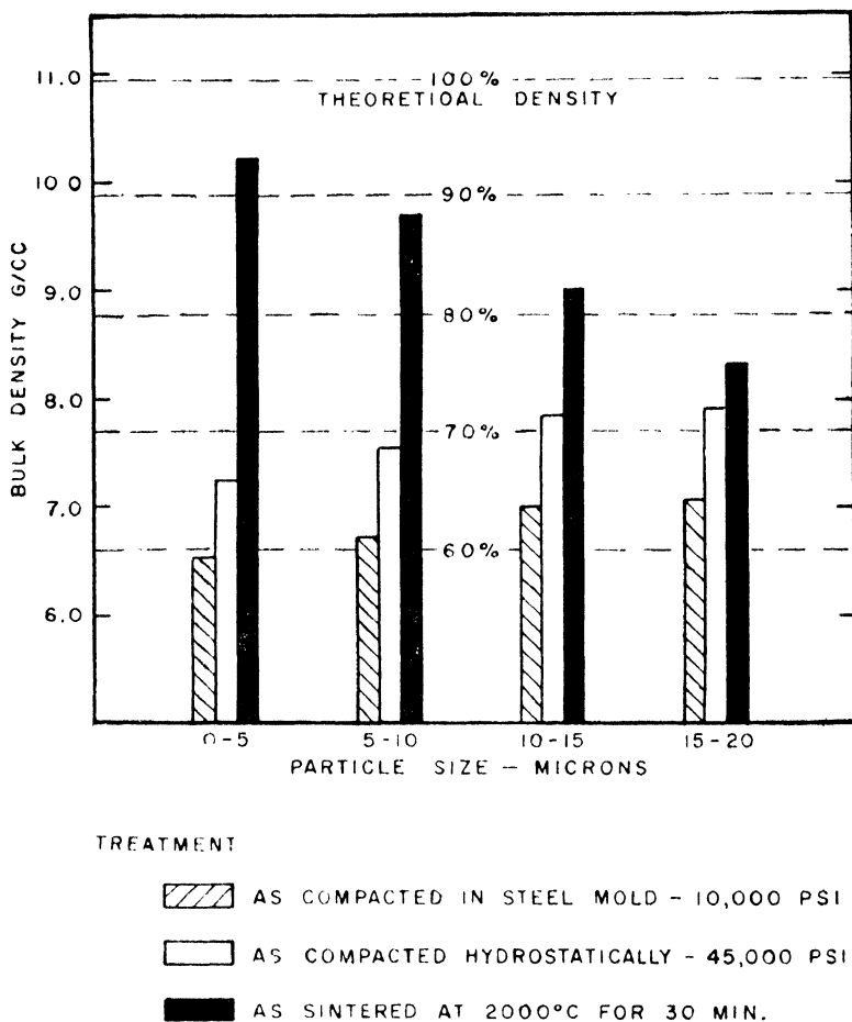
Figure 6. —Density of green compact (unsintered) ranges between 6 and 8.6 g/cc, depending on powder particle size—finer powders compact to lower densities than coarser ones.
