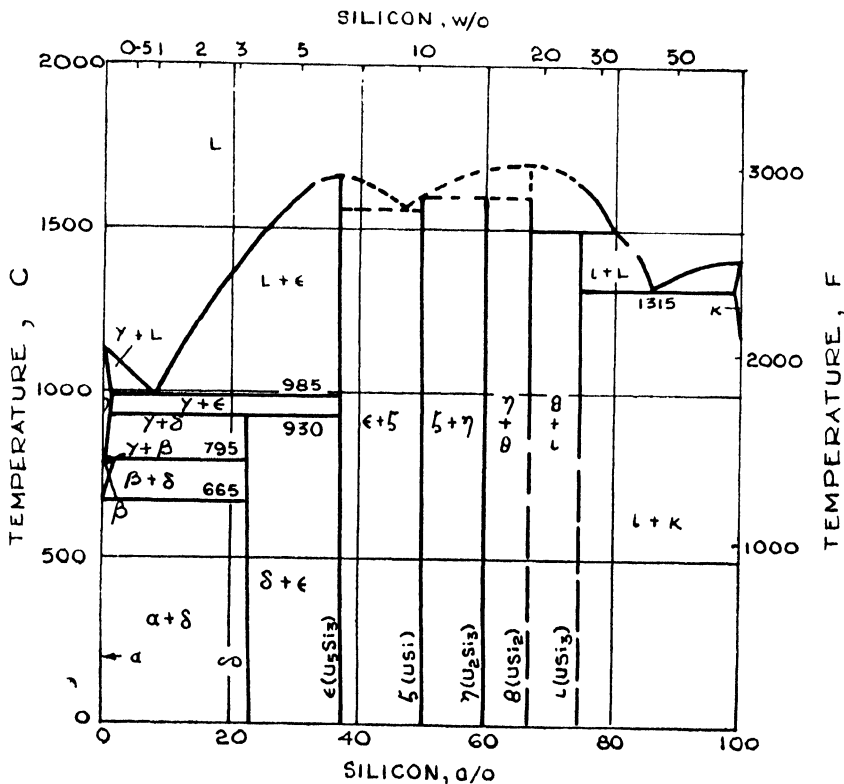
Fig. 28—Uranium-silicon system.
