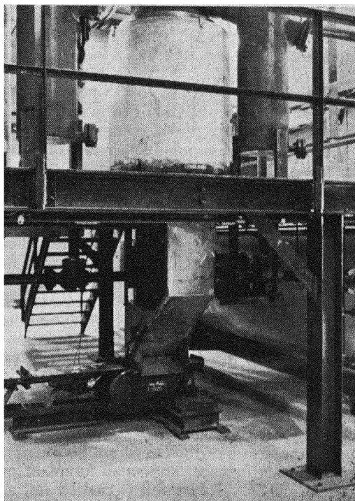
Fig. 11 —Continuous Beryllium Fluoride Furnace on Platform. Casting wheel and \text{BeF}_2 conveyor below platform. Furnaces are 125 KW, 800 volt, 3,000 cycle units, with 50 lb. per hour \text{BeF}_2 production capacity.
