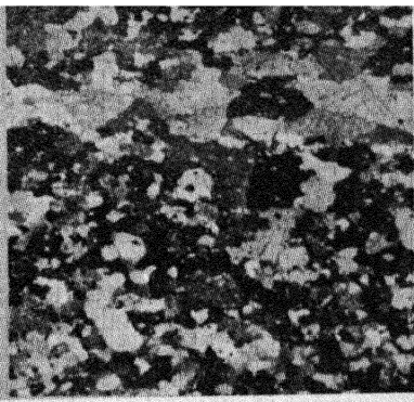
Fig. 14b. —50X. Same as (a) recrystallized 600°C—one hour.
