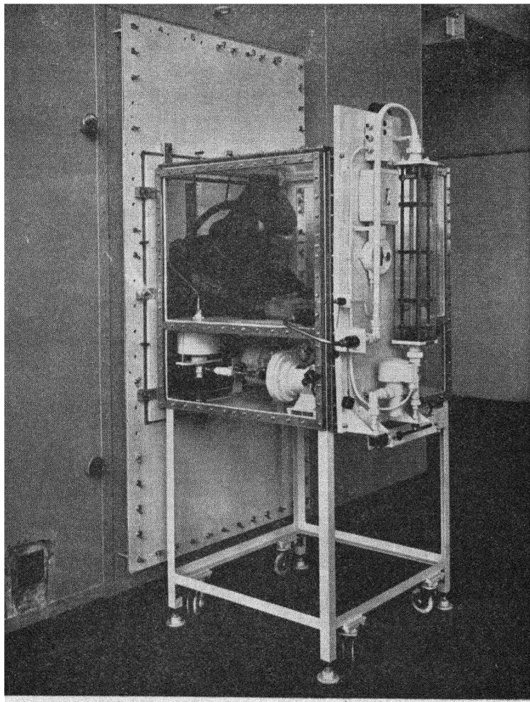
Fig. 2. —Glove box sealed to wall of active workshop and being serviced by pressurized suit operative
