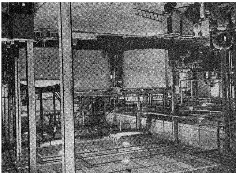
Fig. 5 —General view of ore leaching and beryllium hydroxide production equipment—Dorr thickeners at center, hydroxide equipment, left edge.
