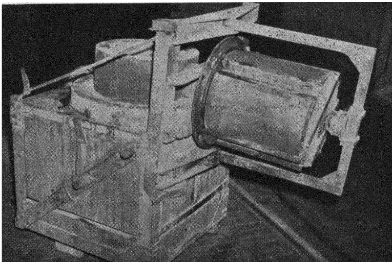
Fig. 12 —100 KW, 800 volt, 3,000 cycle Reduction Furnace. Slag and metal receiving pot are tightly attached to furnace to eliminate fume generation during pouring.
