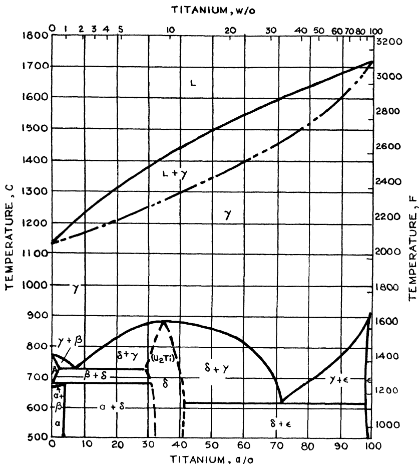
Fig. 24—Uranium-titanium system
