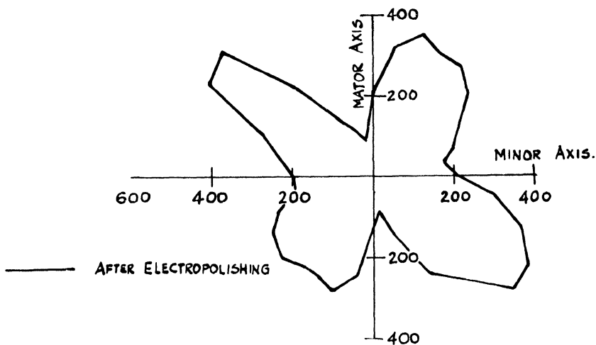
Fig. 7—Radial intensity of the (002) reflection from a 1" round uranium rod rolled in an oval, edge-oval pass sequence (Cu K radiation, using 0.2° geiger tube slit and 1° x-ray tube slit.)
