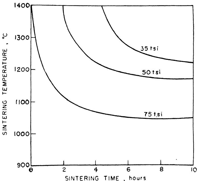
Figure 19.—Isodense lines representing 6.59 g/cc (complete densification) for three compacting pressures. Data for -325 mesh \text{ZrH}_2 powder, vacuum sintered
