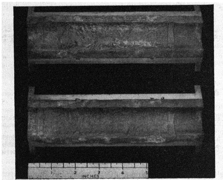
Fig. 10 —Wrinkles on an irradiated cast Uranium bar are reproduced by pressing on to lead.
