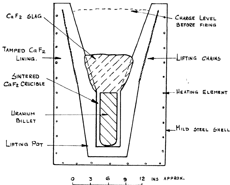
Fig. 3—Calcium— \text{UF}_6 reduction vessel after reaction (40 lb uranium approx.)
