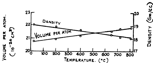
Fig. 2—Some physical constants of Uranium metal.
