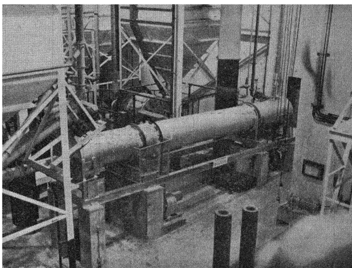
Fig. 3—Ore Heat Treating Kiln. Fine Grinding Mill in background.
