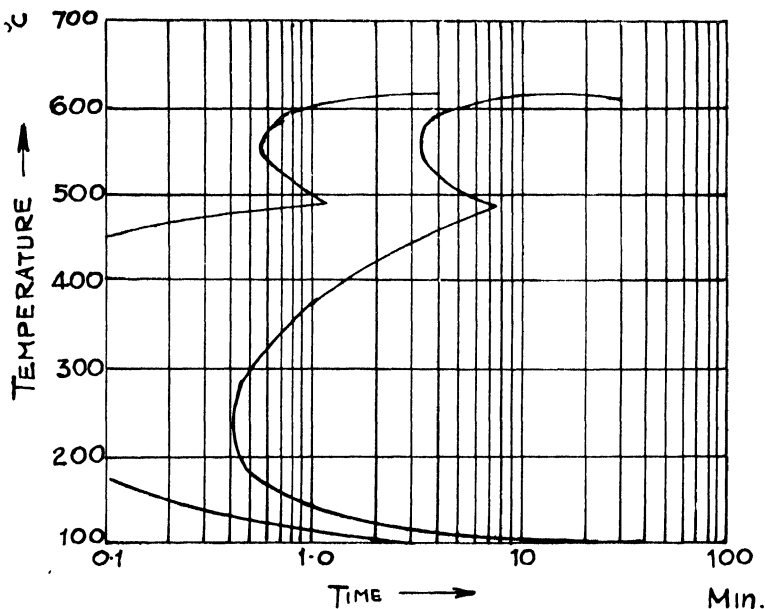
Fig. 14—TTT curve for uranium. 0.3 at % Chromium Alloy.
