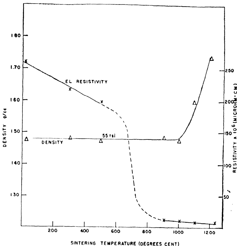
Figure 13. —Effect of sintering temperature on density and electrical resistivity of beryllium. Specimens sintered 3 hrs. in vacuo; measurements at room temperature
