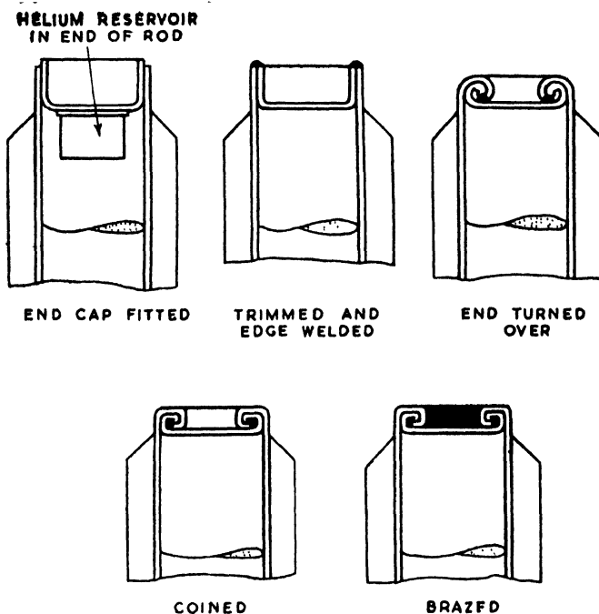
Fig. 17—Method of sealing uranium fuel containers.
