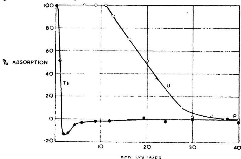
Figure 7.—Uranium and thorium absorption.
