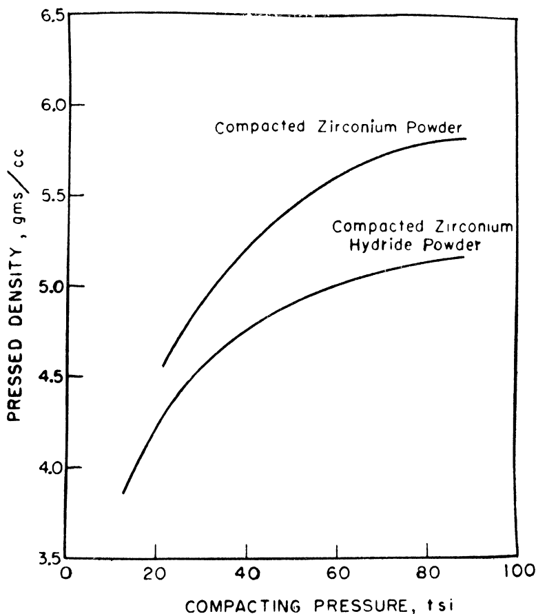
Figure 16.—Effect of compacting pressure on the “green” density of compacted zirconium and zirconium-hydride powder, respectively
