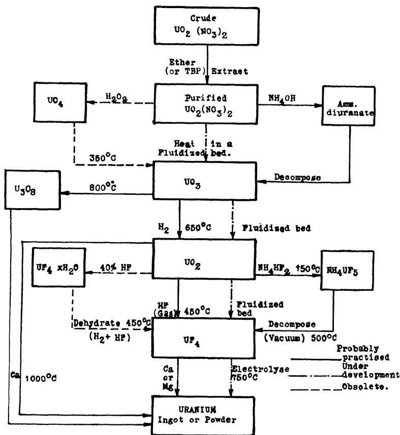
Fig. 1—Flow sheet for the production of Uranium
