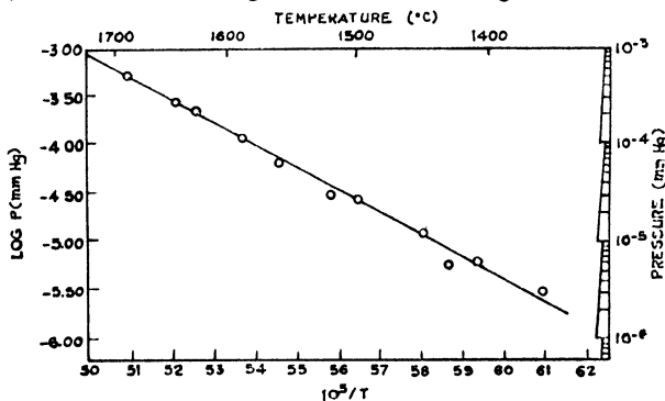
Fig. 1—Vapour pressure of uranium.
