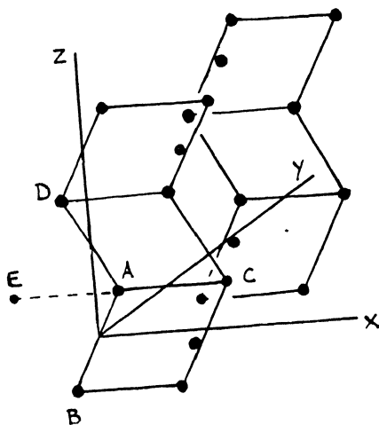
Figure 4.—Atomic structure of \alpha -uranium
