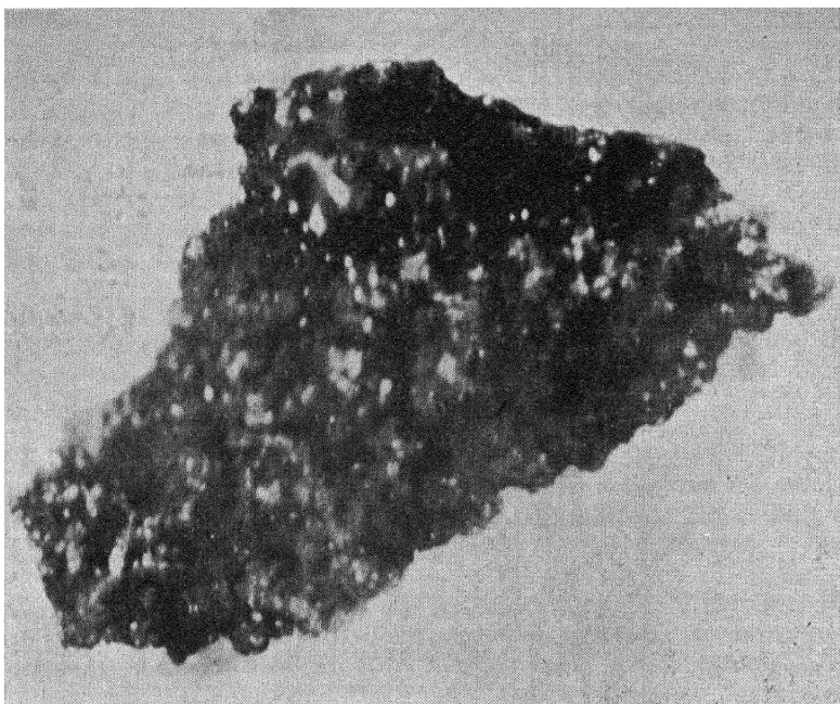
Fig. 13 —Disruption of uranium by fission product gas at high burnup.
