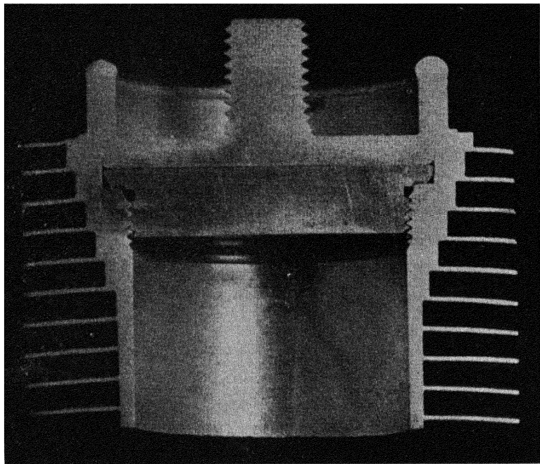
Fig. 23—Magnesium alloy fuel element with circumferential fins. These fuel elements have an edge-welded cap
