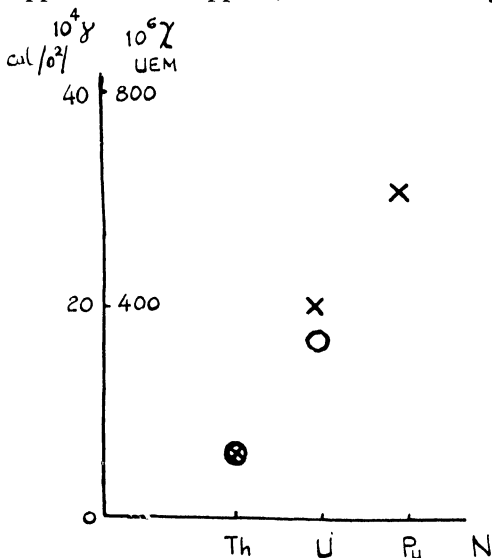
Figure 5.—Density of states at the Fermi level, deduced from the electronic specific heat \Delta C_v = \gamma T and from the magnetic susceptibility \chi . Crosses: \chi in 10^6 \text{UEu Cm}^{-3} circles: \gamma in 10^4 \text{ cal deg}^{-2} \text{ mole}^{-1} < 1 .
