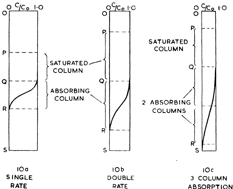
Figure 10.— Effect of flowrate.
