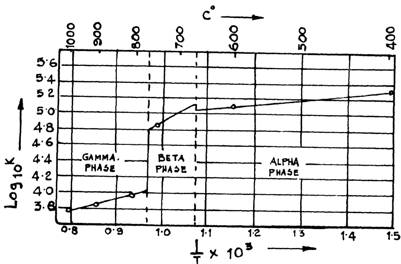
Fig. 8—The variation of the extrusion constant of uranium with temperature.
