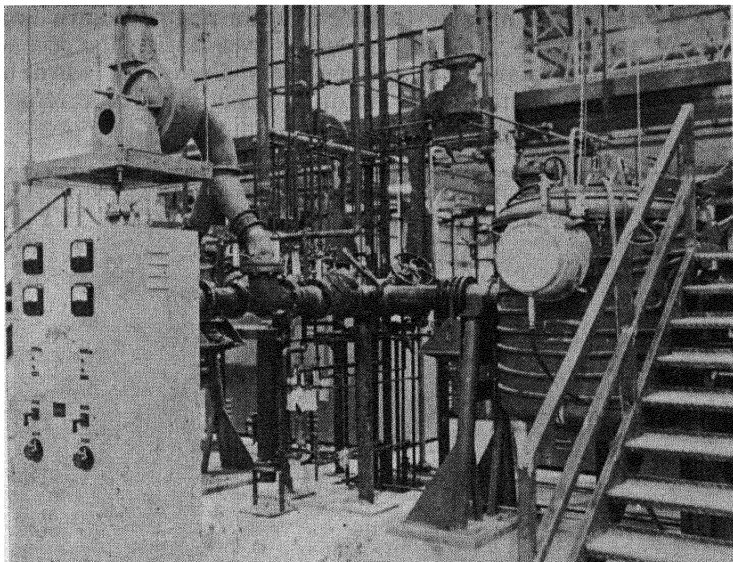
Fig. 13—Vacuum Casting Equipment. Light coloured attachment is mold container. Note ventilation system connection to furnace through trunion. This provides ventilation on furnace shell to make charging operation safe.
