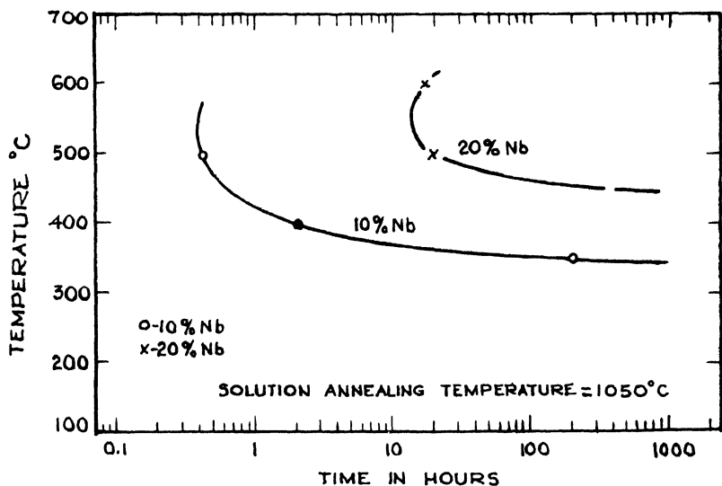
Fig. 31—TTT diagrams illustrating initial resistivity decrease for U-Nb Alloys.
