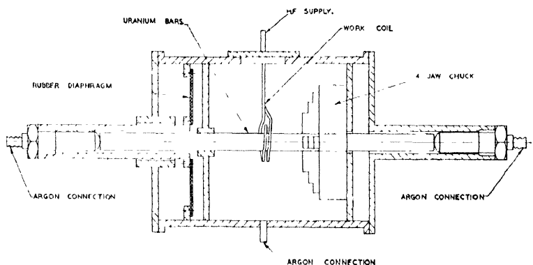
Fig. 7—Chamber developed for the pressure welding of uranium bars.
