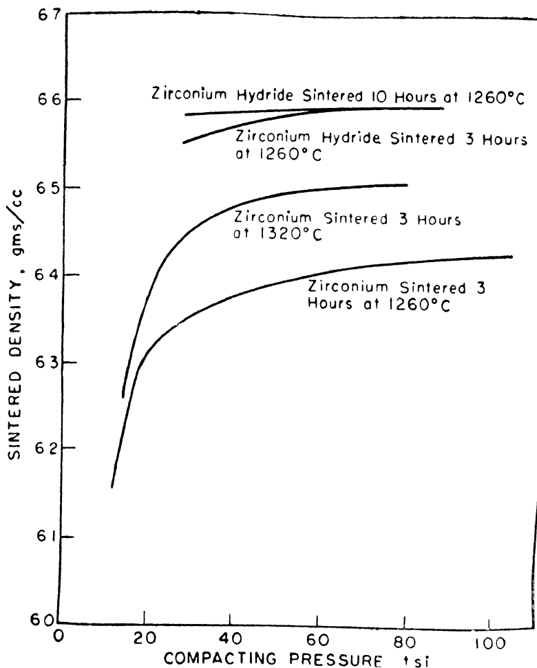
Figure 17.—Effect of compacting pressure on the sintered density of compacted and sintered zirconium-hydride powders (sintered in high vacuum)
