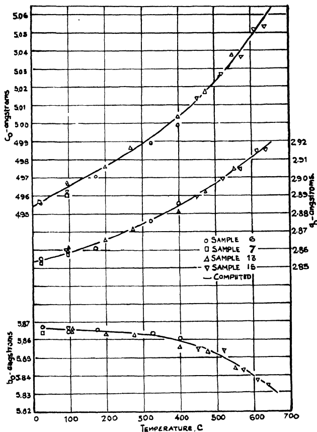
Fig. 16—Unit cell dimensions of \alpha Uranium as a function of temperature.
