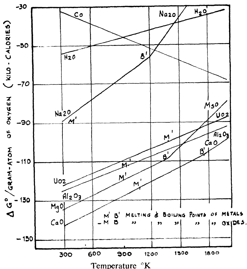
Fig. 2—Free energies of formation of oxides as a function of temperature.
