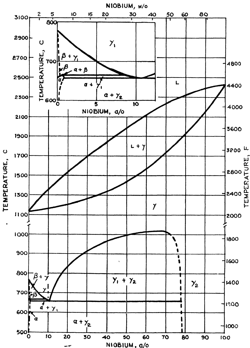
Fig. 25—Uranium-niobium system
