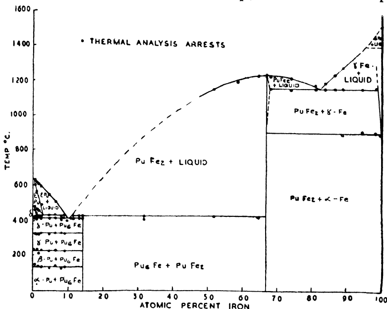
Fig. 8.—The plutonium—iron system
