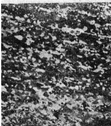
Fig. 14c. —50X. 87% reduction in area at 300°C, annealed one hour at 475°C.
