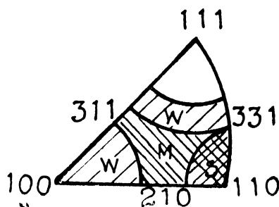
Figure 6—Compression rolling texture for thorium W = Weak, M = Medium, S = Strong
