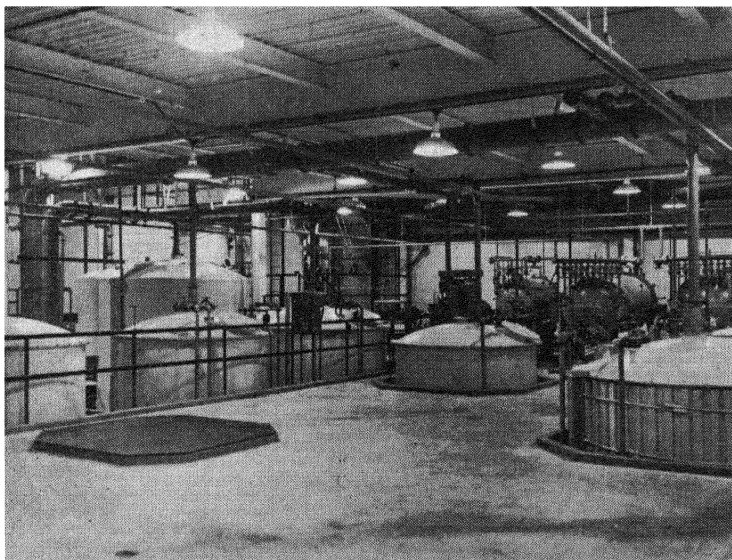
Fig. 9 —Ammonium Beryllium Fluoride Solution Purification Area. Self-cleaning filters used for impurity separation in right background.
