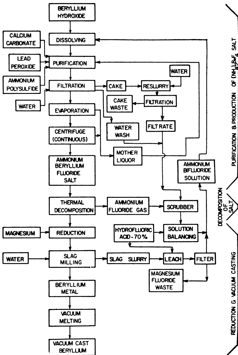
Fig. 8—Flow Sheet.
