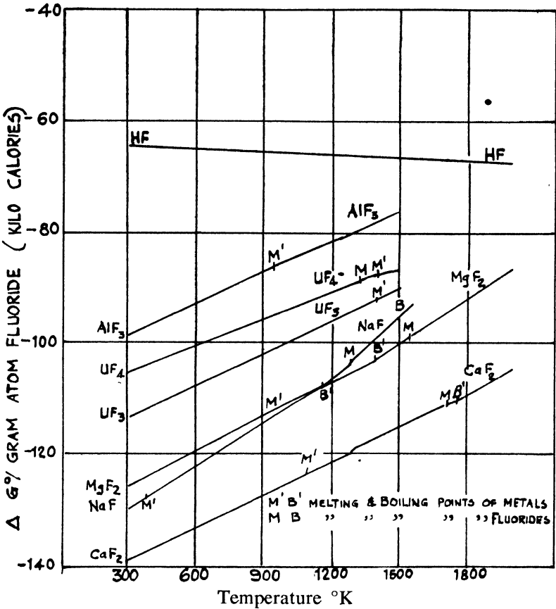
Fig. 1—Free energies of formation of fluorides as function of temperature.
