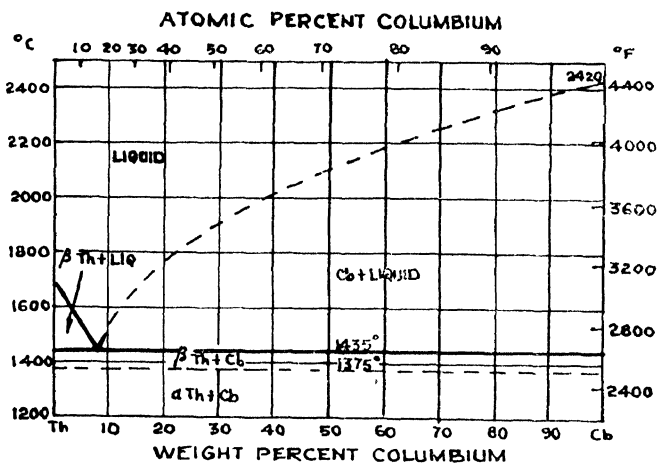
Fig. 18.—Thorium-niobium system
