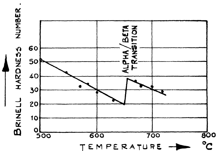
Fig. 12—The variation in hardness of Uranium with temperature. (Munro.)
