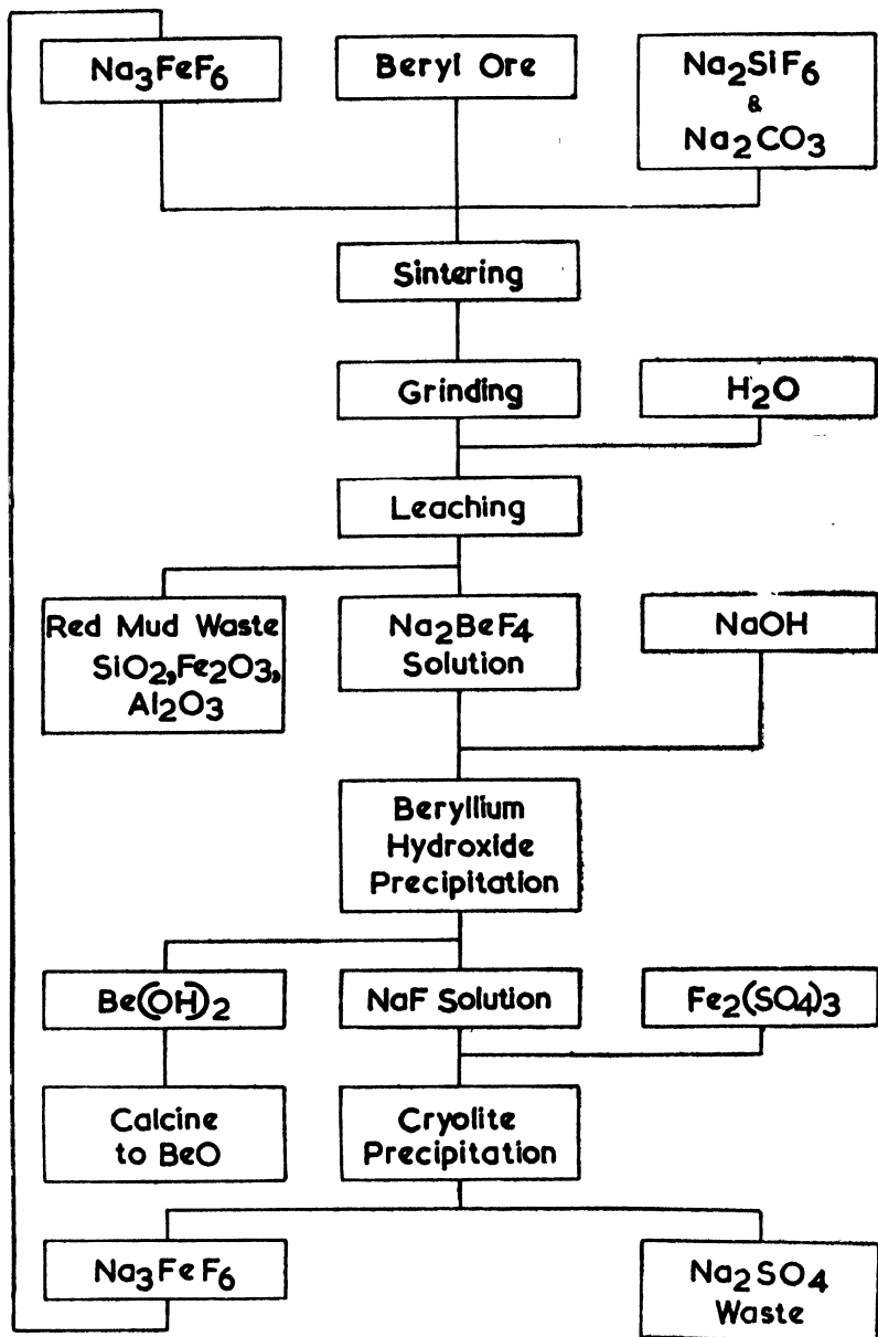
Fig. No. I—Flow Sheet of Fluoride Process for Reduction of Beryl.
