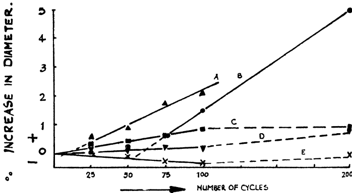
Fig. 18—Effect of alloy additions on the dimensional stability of uranium, Thermally cycled through the \alpha - \beta phase transformation temperature 9
