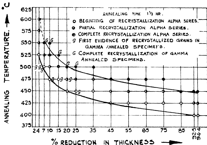
Fig. 13—Recrystallization temperatures are function of per cent reduction of uranium plate at room temperature. (Hayes, 1949).
