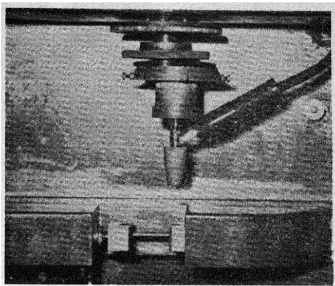
Fig. 22 —Automatic Argon-Arc Welding equipment developed for assembling fuel can elements.
