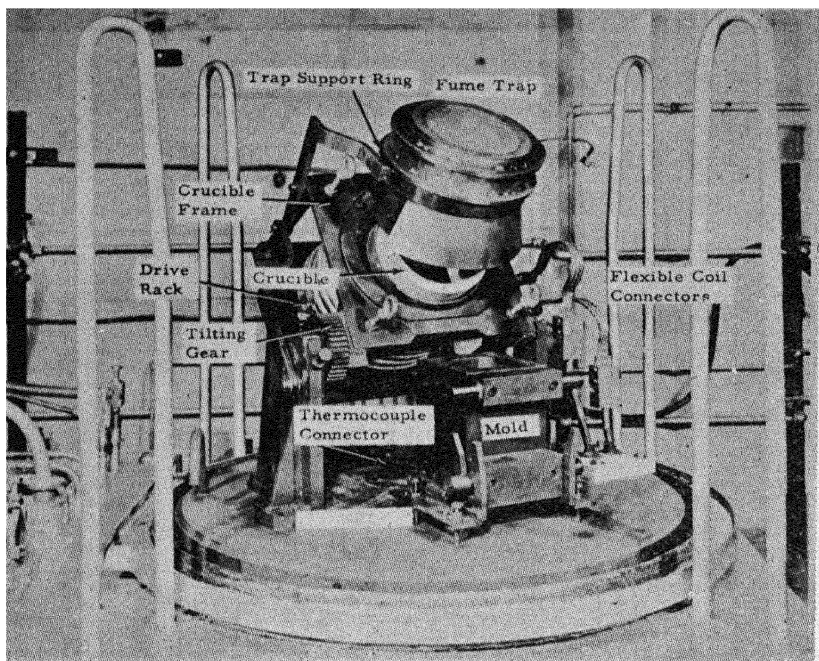
Fig. 10—Crucible Assembly in Partially Tilted Position . . .
