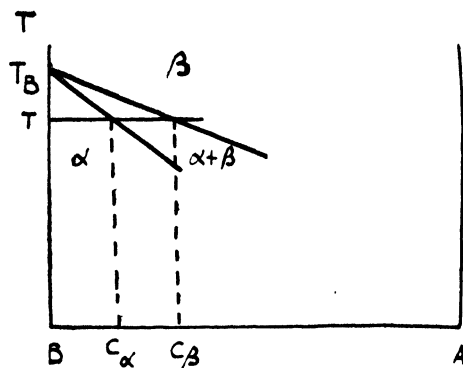
Figure 9.—Influence of solute A on the \alpha \beta allotropic transformation of solvent B.
