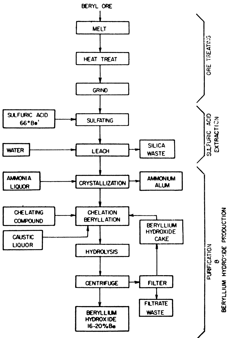
Fig. 1—Flow Sheet of Beryllium Hydroxide Production: Brush Process
