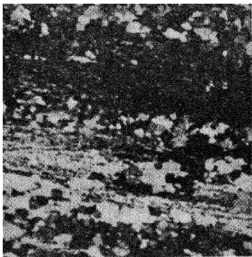
Fig. 14a. —50X. 89% reduction in area at 600°C.
