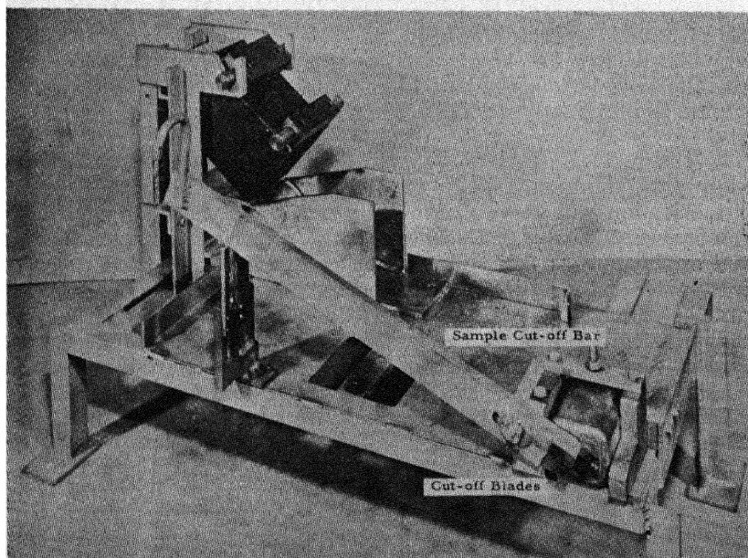
Fig. 11—Ingot Remover and Sampler.
