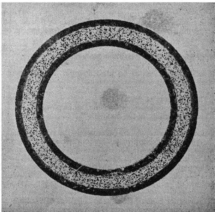
Figure 10. —Tubular fuel element. Core : 65 w/o \text{UO}_2 in aluminium. Cladding : aluminium (Mag. 15x). (Courtesy : Martin Company)
