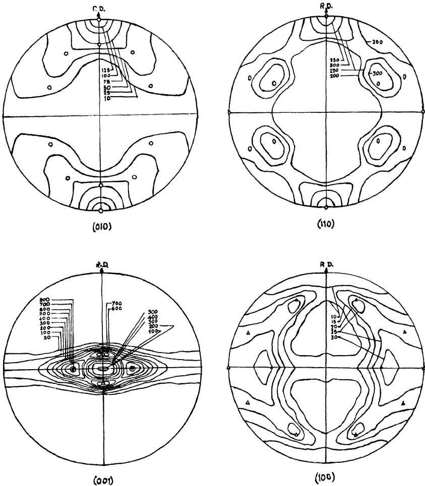
Fig. 10—Pole figures for uranium sheet rolled at 300°C to an 87% reduction.
