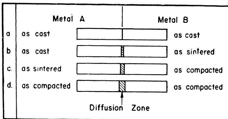
Figure 1. —Diffusion between two metals, A and B, under constant temperature, time and pressure conditions as a function of their method of preparation
