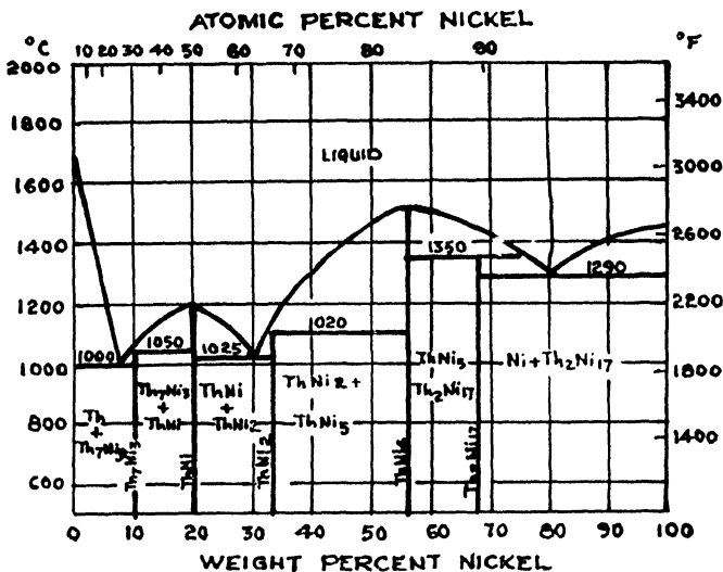
Fig. 16.—Thorium-nickel system
