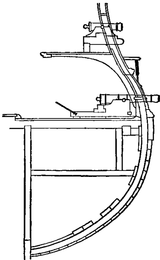
Section of frigate, with long gun on main-deck and carronade on spar-deck. Taken from "The American Artillerist's Companion," by Louis de Toussard (Philadelphia, 1811).
