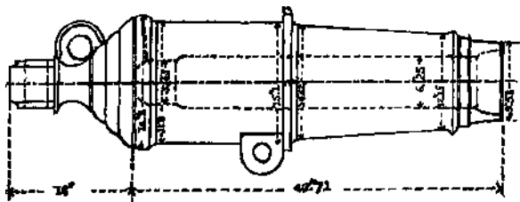
32-Pound Carronade, 1779.—Weight, 17 cwt.
