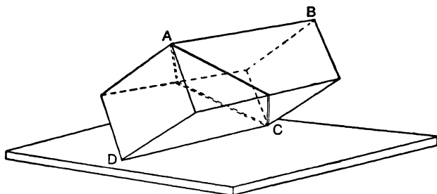
Fig. 134 a .—Method of cutting Rhomb of Iceland Spar to make a Nicol Prism
