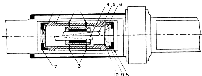
Fig. 163.—Bellingham and Stanley's Half-shade
