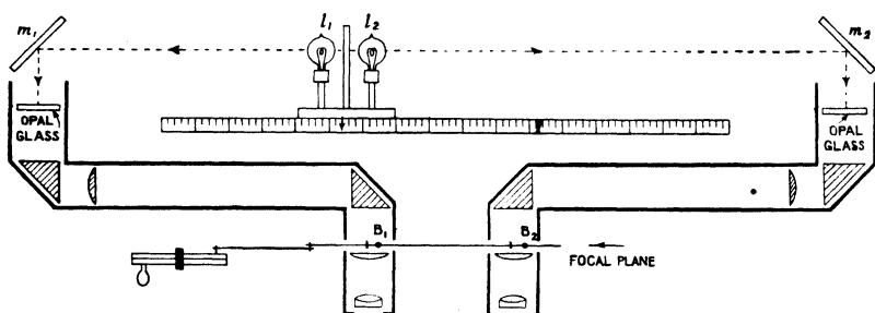
Fig. 159.—Stereoscopic Photometer used to compare two Lamps
