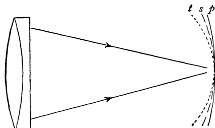
Fig. 2.—Curvature of Field (size of lens exaggerated)
