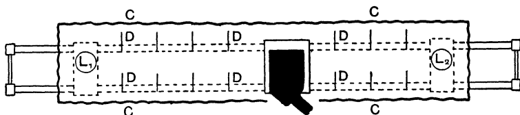
Fig. 141.—Photometric Bench with Diaphragms and Curtains
