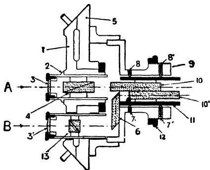
Fig. 153.—The Bellingham-Stanley Spectrophotometer
