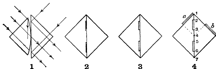
Fig. 143.—Forms of Photometer Prisms
