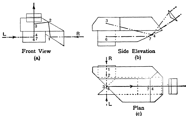
Fig. 62.—Barr & Stroud Centre Prism
