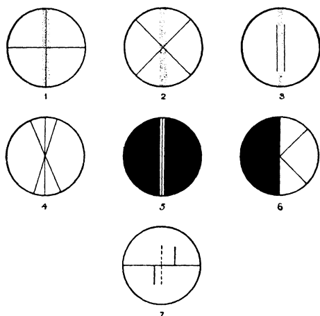
Fig. 16.—Types of Setting in Optical Instruments
