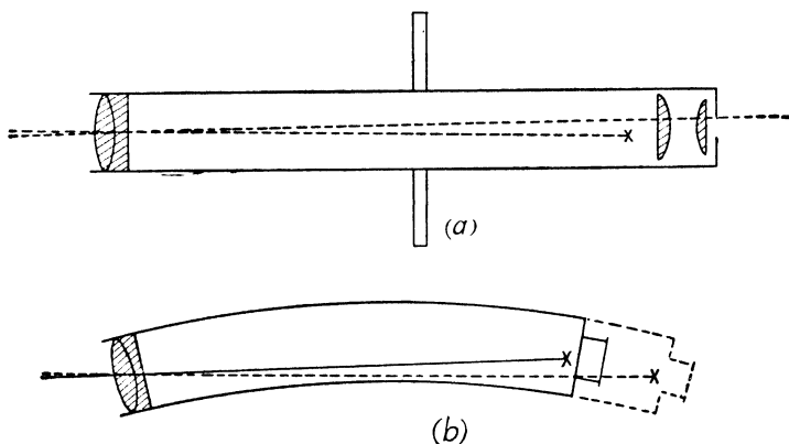
Fig. 35.—Collimation Error
