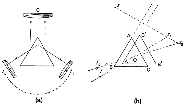
Fig. 77.—Determination of Prism Angles: Possible Errors
