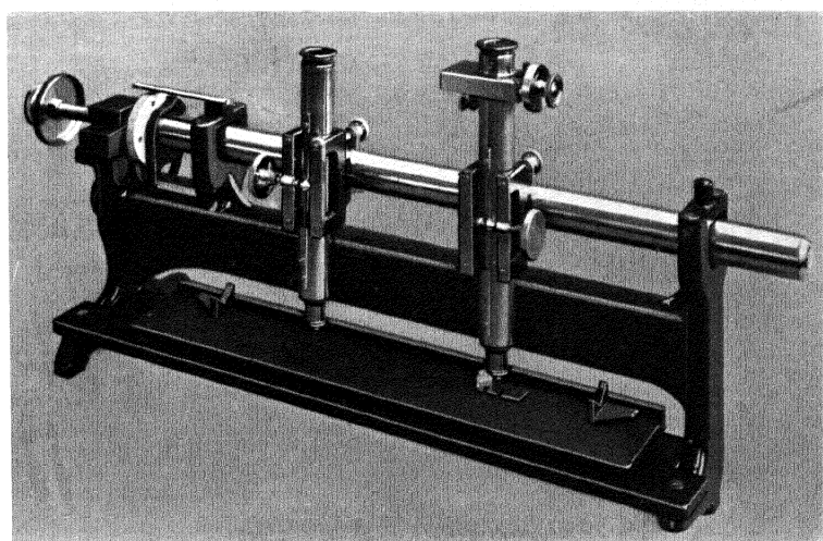
Fig. 27.—Comparator (Cambridge)
