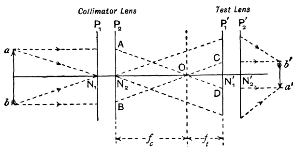
Fig. 122.—Use of Focal Collimator
