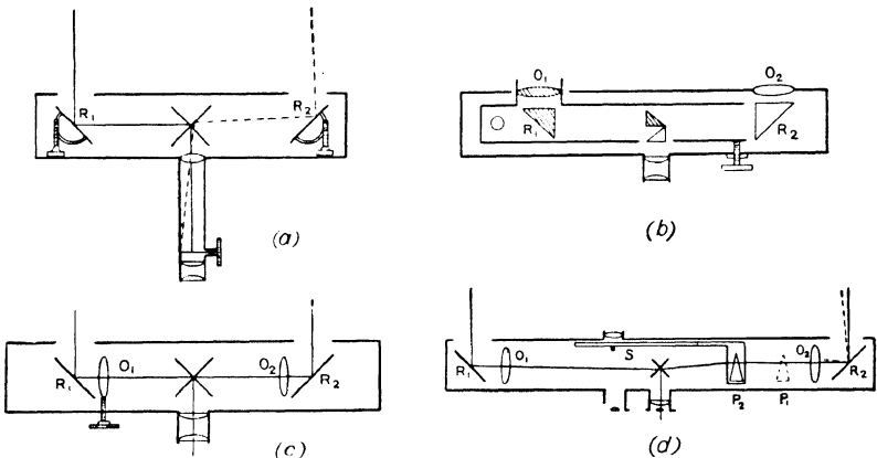
Fig. 56.—Early Types of Range-finder
