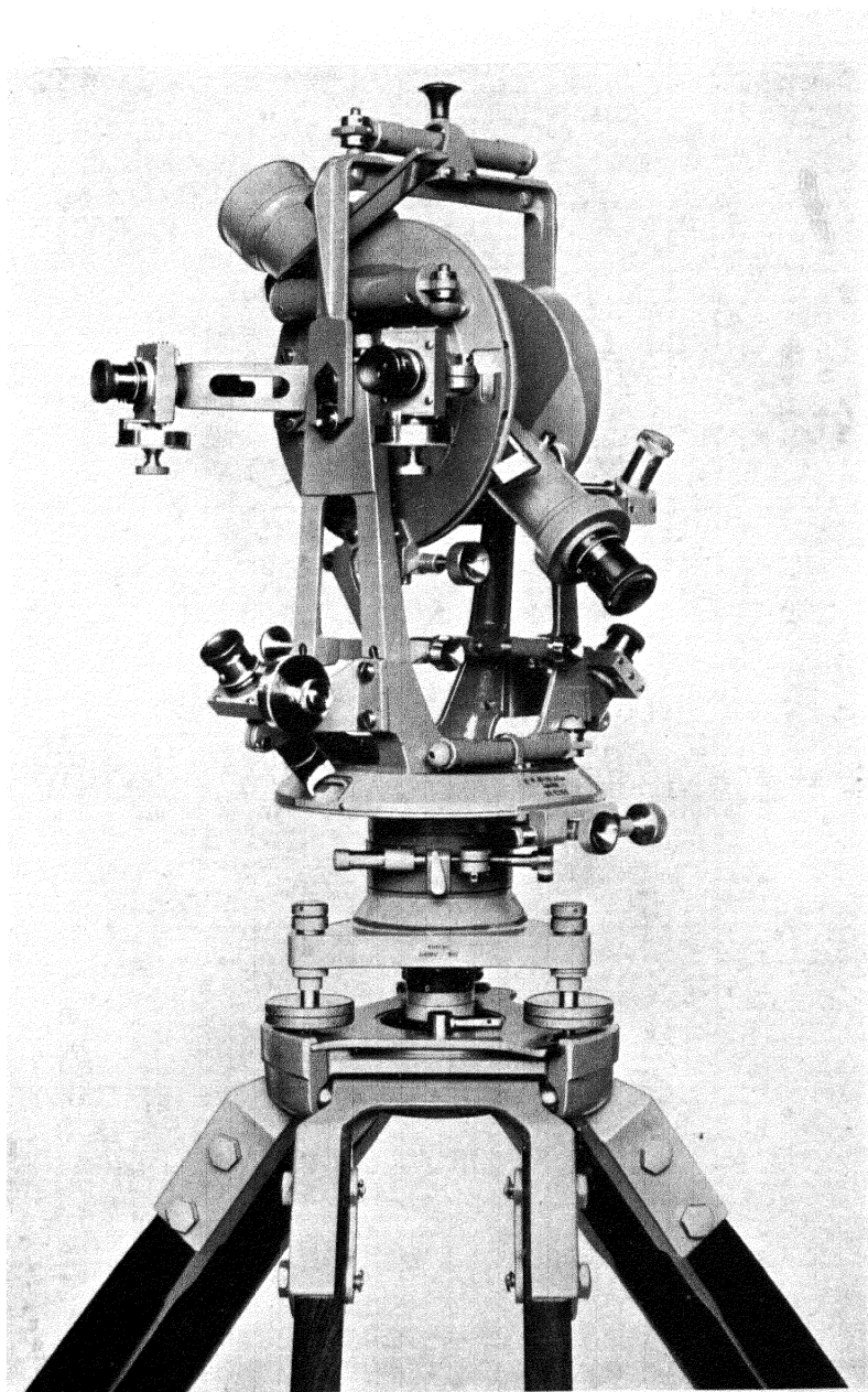
Fig. 41.—Watts' Micrometer Theodolite
