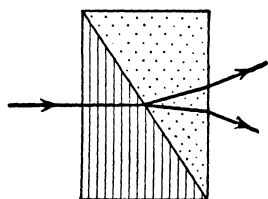
Fig. 137.—Wollaston Prism
