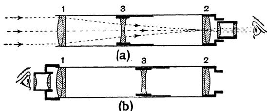
Fig. 53.—Reversible Telescope of the Zeiss Level
