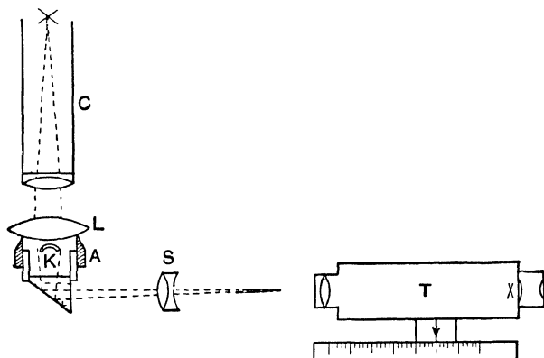
Fig. 130.—Zeiss Focometer
