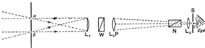
Fig. 144.—König-Martens Type of Photometer: to illustrate optical system
