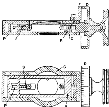
Fig. 20.—Construction of Micrometer Eyepiece
