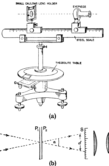
Fig. 121.—Apparatus for the Rotating Table Method
