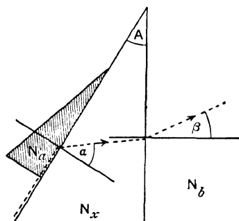
Fig. 86.—Critical-angle Refractometry
