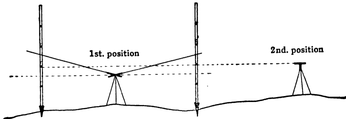
Fig. 49.—Adjustment of Dumpy Level (diagrammatic)
