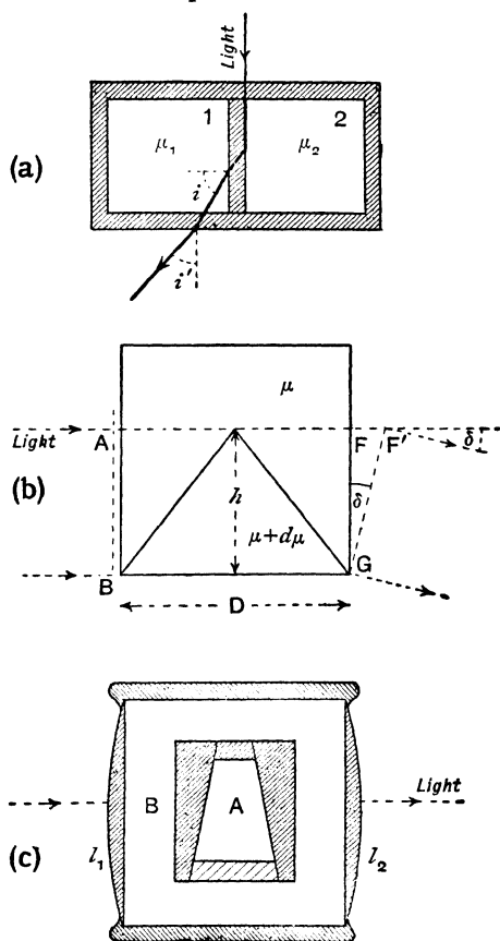
Fig. 99.—Differential Refractometers
