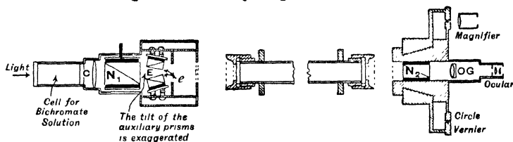
Fig. 168.—Diagram of Parts of Lippich Polarimeter
