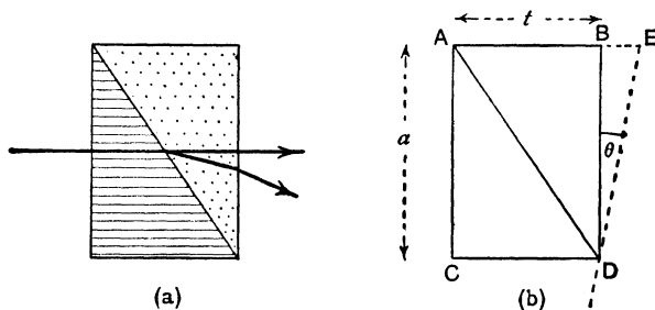
Fig. 136.—Rochon Prism and Theory
