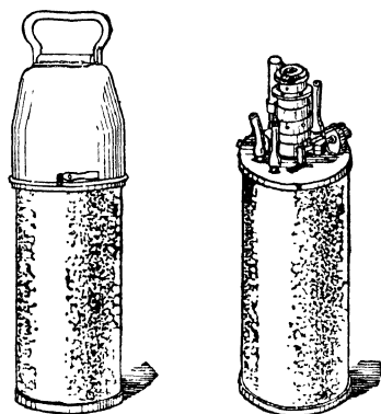
Fig. 103.—The Portable Gas Interferometer, shown with and without Carrying Guard Hood
