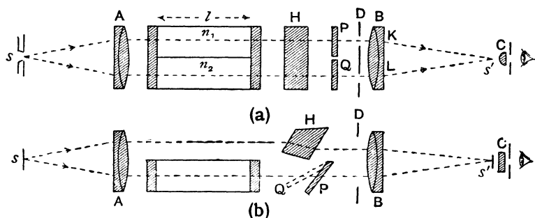
Fig. 100.—The Gas Refractometer
