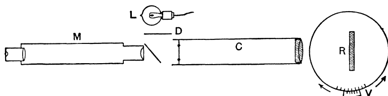
Fig. 123.—Adjustment and Determination of Constant of Focal Collimator
