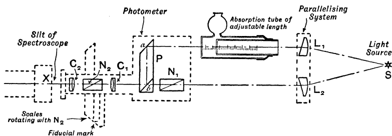
Fig. 151.—Optical System of Nutting Spectrophotometer
