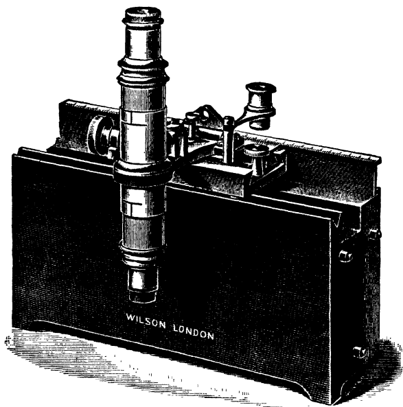
Fig. 11.—Laboratory Vernier Microscope by Wilson
