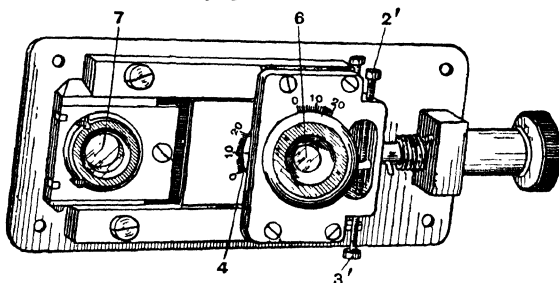
Fig. 167.—Bellingham and Stanley's Compensator
