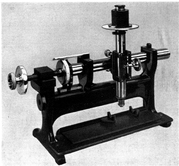
Fig. 17.—Cambridge Measuring Microscope
