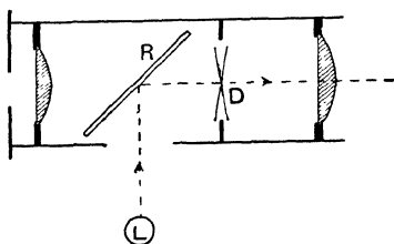
Fig. 76.—Gauss Eyepiece L, Source of light. R, Plain glass reflector. D, Diaphragm carrying cross wires.
