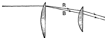
Fig. 117.—A Simple Huygenian Eyepiece (diagrammatic)
