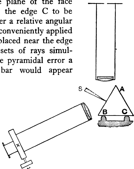
Fig. 81.—Angle Comparator (diagrammatic)
