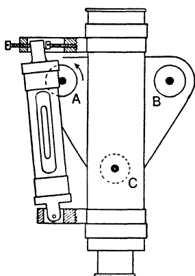
Fig. 54.—Plan of Zeiss Level (diagrammatic)
