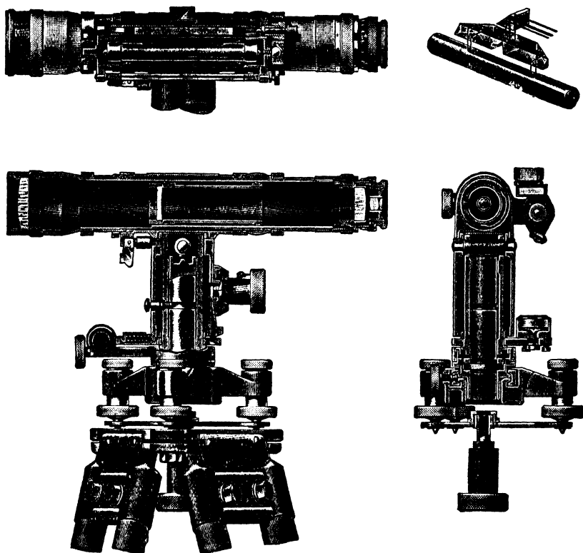
Fig. 51.—The Zeiss Level (Type 2)
