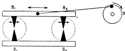
Fig. 158.—The Fixed and Moving Marks seen in the Field View of each Telescope
