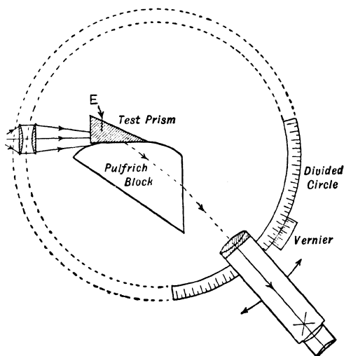
Fig. 88.—Pulfrich Refractometer (diagrammatic)
