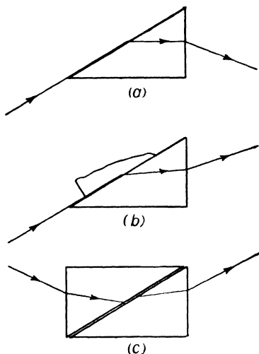
Fig. 93.—Grazing Incidence Refraction in Three Cases
