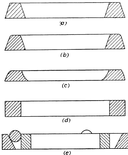
Fig. 110.—Forms of Support for Spherometers
