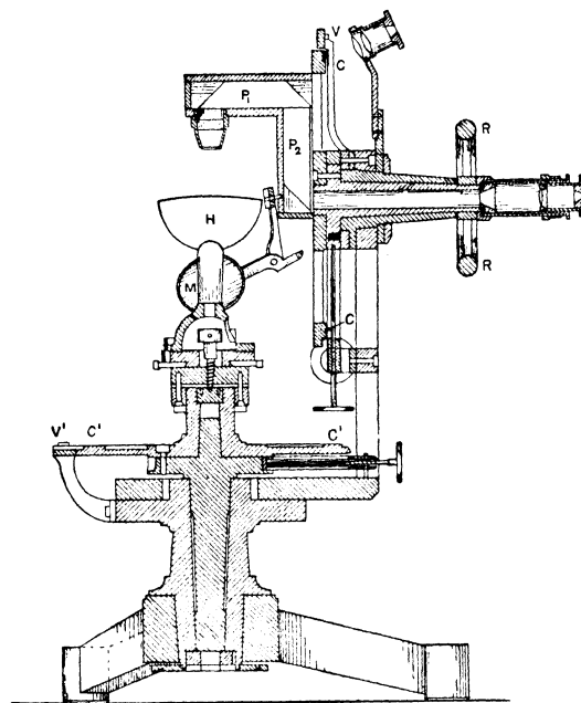
Fig. 98.—Cross-section of the Crystal Refractometer
