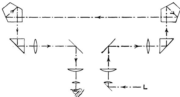
Fig. 73a.—Abbe Adjuster for Stereoscopic Range-finder
