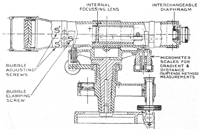
Fig. 48.—Engineers' Precise Level (Diagrammatic)
