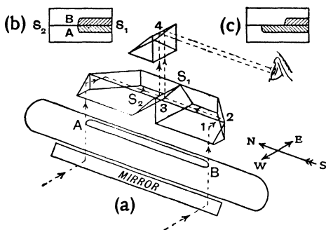
Fig. 52.—The Bubble Observation System of the Zeiss Level
