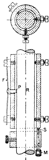
Fig. 8.—Cathetometer Mounting
