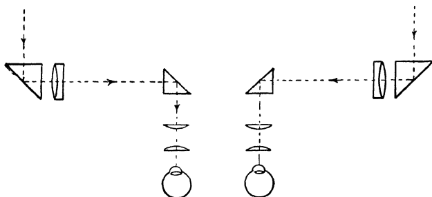
Fig. 71.—Stereoscopic Telescope
