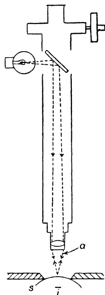
Fig. 111. — Curvature Measurement by Guild's Substitution Method
