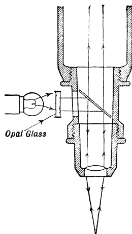
Fig. 25.—Vertical Illuminator
