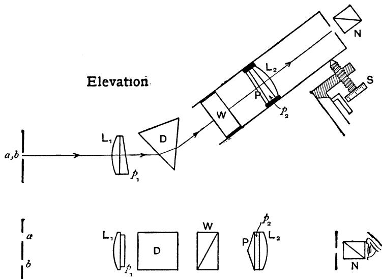
Plan (not allowing for upward deviation)
