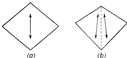
Fig. 160.—End views of (a) Nicol Prism, (b) Jellet-Cornu Prism. The arrows indicate the direction of vibration of the polarized light.
