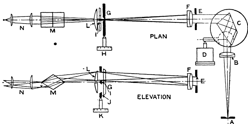
Fig. 154.—Bull's Spectrophotometer
