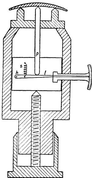
Fig. 108.—Spherometer with Mechanical Device for indicating Contact.
