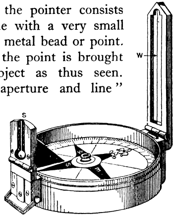
Fig. 9.—Prismatic Compass (to show sighting method)
