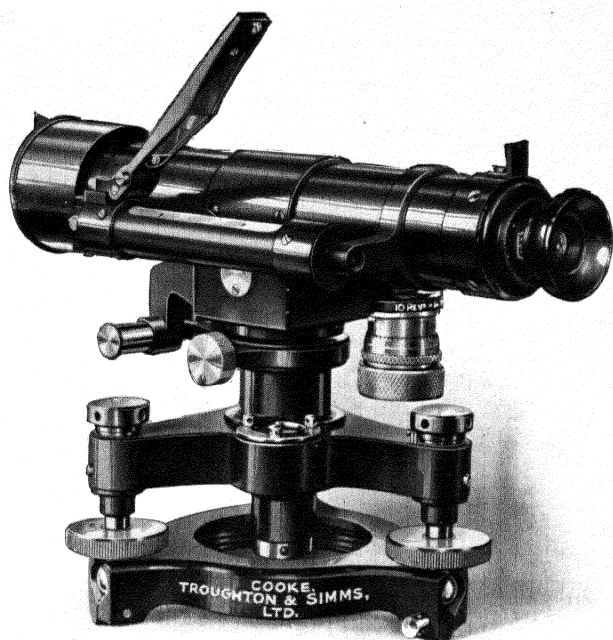
Fig. 47.—Engineers' Precise Level
