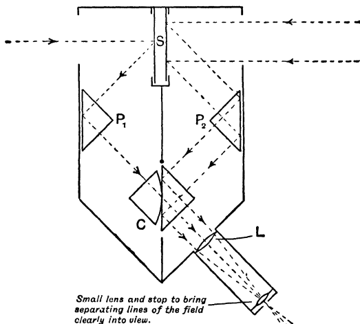
Fig. 142.—Lummer-Brodhun Photometer Head
