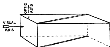
Fig. 135.—Glan-Thompson Prism
