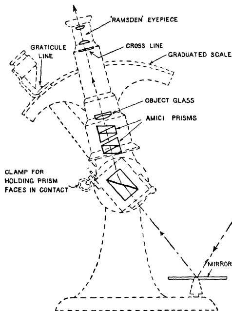
Fig. 92.—Optical System of Abbe Refractometer
