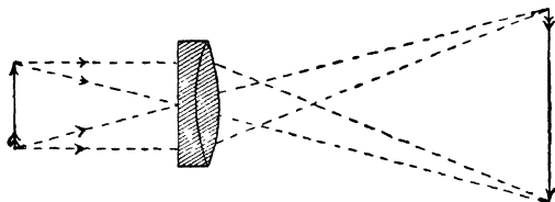
Fig. 116.—The Microscope Objective (diagrammatic)
