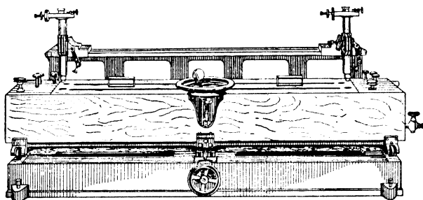
Fig. 26.—Large Comparator
