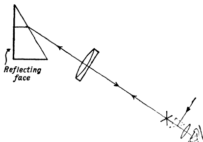
Fig. 84.—Auto-collimating Spectrometer
