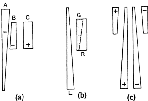
Fig. 165.—Quartz Wedge Compensators (a) Early type (solid). (b) Marten's modified type. (c) Double wedge.
