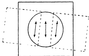
Fig. 161.—Diagram to illustrate production of Tripartite Field in a Polarimeter by use of two Auxiliary Prisms (Lippich end-point device).
