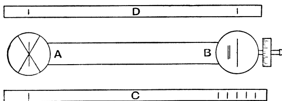
Fig. 24.—Comparator (diagrammatic)
