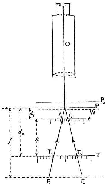
Fig. 126.—Optical Principles of Zeiss-Abbe Focometer
