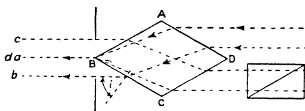
Fig. 150.—Hufner's Spectrophotometer
