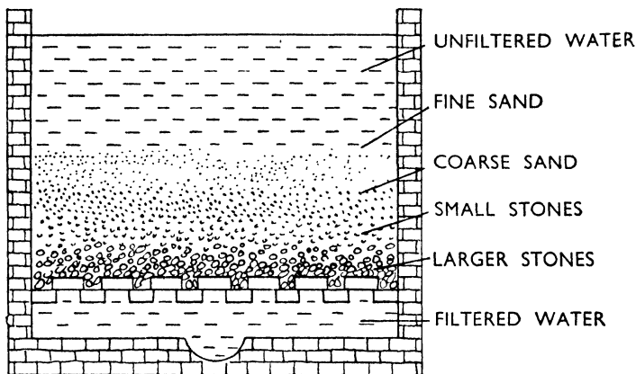
FIG. 60. SAND FILTER
