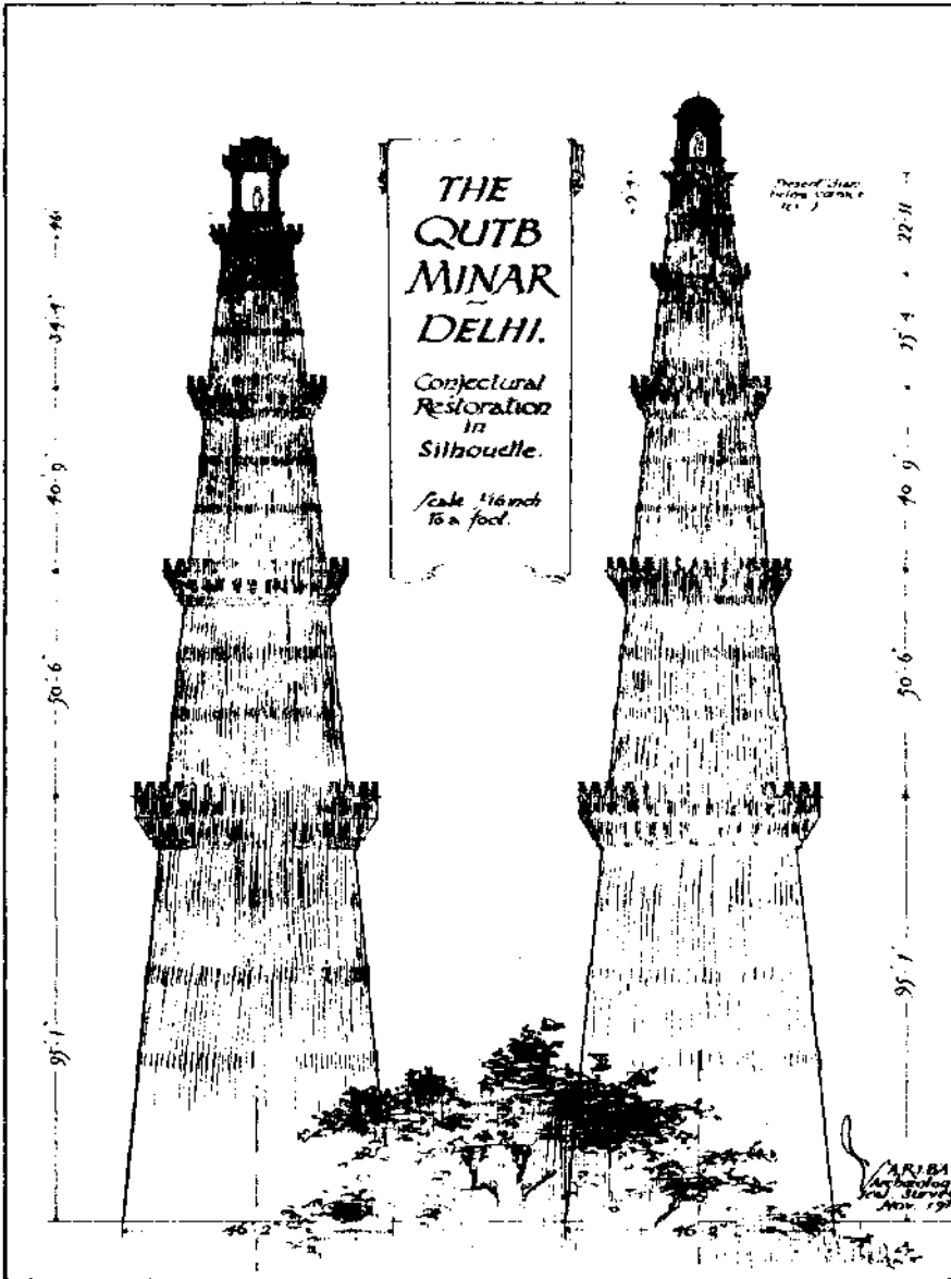
Original Minar, as completed by Altamish, 1230 A.D. Minar as heightened by Feroz Shah, 1370 A.D.
