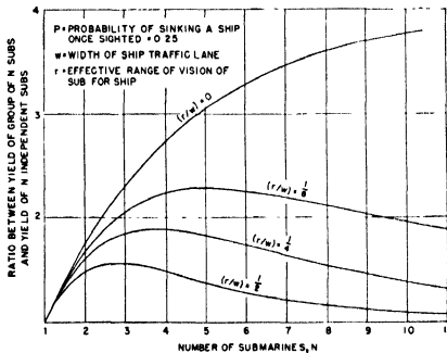
FIGURE 1 Relative advantage of group action over independent action for submarines against merchant vessels
