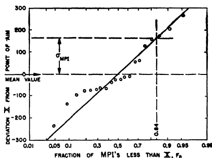
FIGURE 1. Use of probability paper. Deviations from MPI, \sigma = 18 , \sigma_n = 18\sqrt{2} = 25 .
