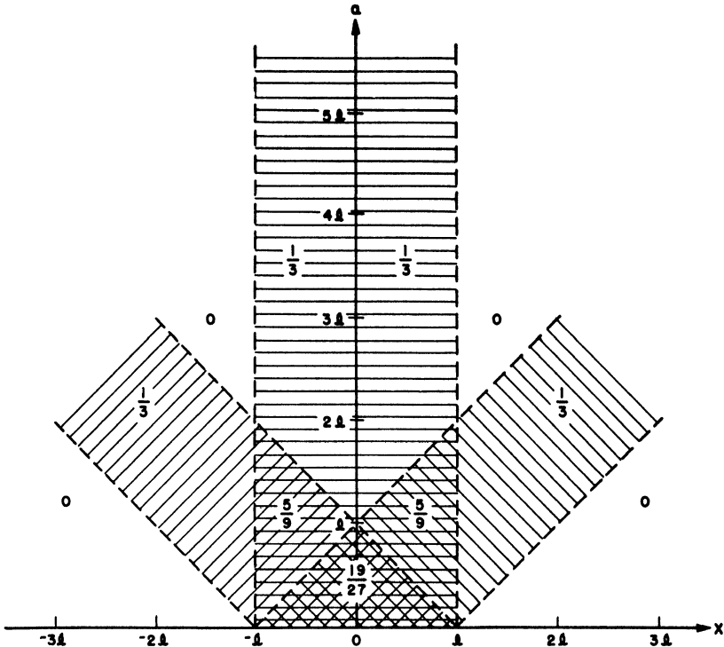
FIGURE 2 Damage function for spread of three torpedoes. No ballistic dispersion. D_p = 19/27 in triple-shaded region, 5/9 in double-shaded region, 1/3 in single-shaded region, 0 in unshaded region.
