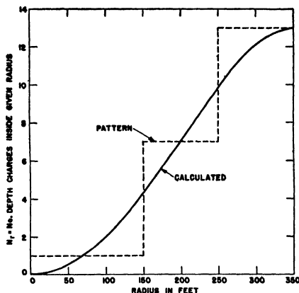
FIGURE 9. Number of depth charges inside radius r for 13-depth charge pattern.
