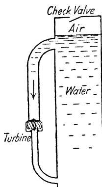
Bernoulli's Principle Applied to Perpetual Motion.
