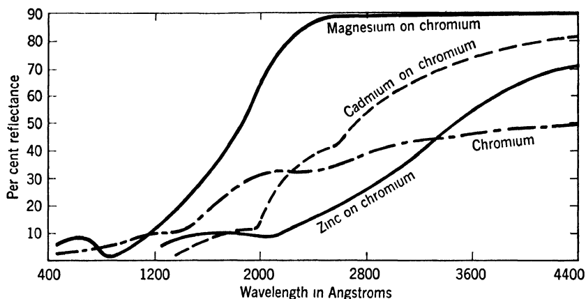
FIG. 9. Reflection from evaporated films of cadmium, magnesium, zinc, and chromium. (J. B. Sabine, loc. cit.)
