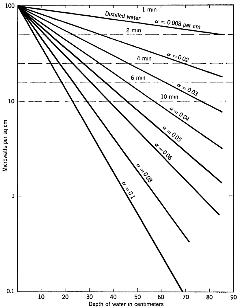
FIG. 12. Intensity of 2537 Å radiation as a function of depth below the surface of water for the various values of absorption coefficient.
