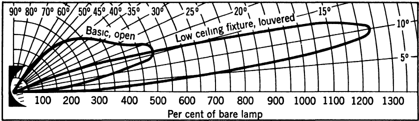
FIG. 9. Distribution of radiation from typical fixture. ( Gen. Elec. Lamp Bulletin LD-14.)
