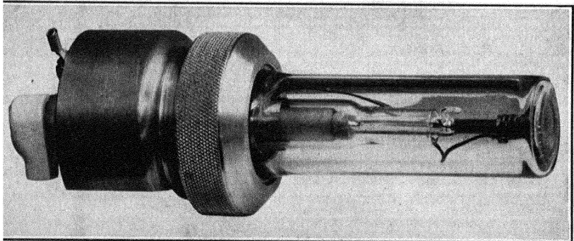
FIG. 18. Water-cooled high-pressure (110 atmospheres) mercury arc showing lamp in water jacket. (Courtesy of General Electric Co.)
