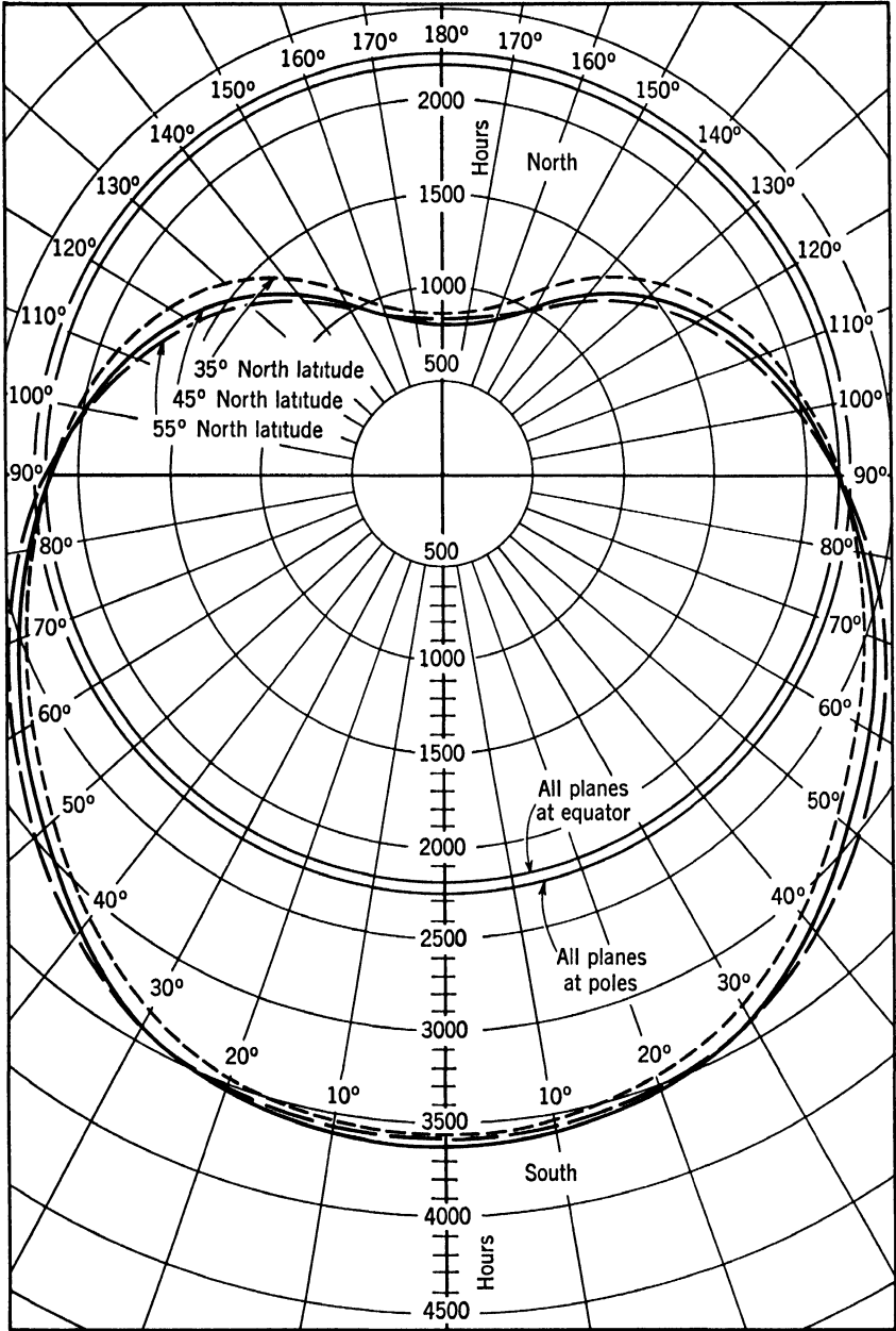
FIG. 19. Total annual hours of sunshine received on vertical surfaces facing various points on the horizon at different latitudes. (F. Benford and J. E. Bock, Trans. Illum. Eng. Soc. , 34 , 200, 1939.)
