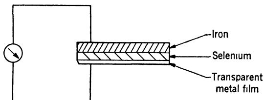
FIG. 11. Photovoltaic cell. Schematic diagram.
