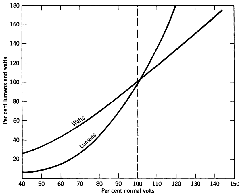
FIG. 5. Effect of voltage variation on output of incandescent lamp. ( Gen. Elec. Lamp Bulletin LD-1. )
