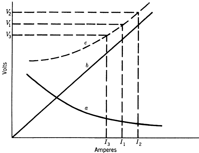
FIG. 3. Stability of an arc with a ballast resistance. a . Arc characteristic. b . Ballast characteristic. c . Combined characteristic.
