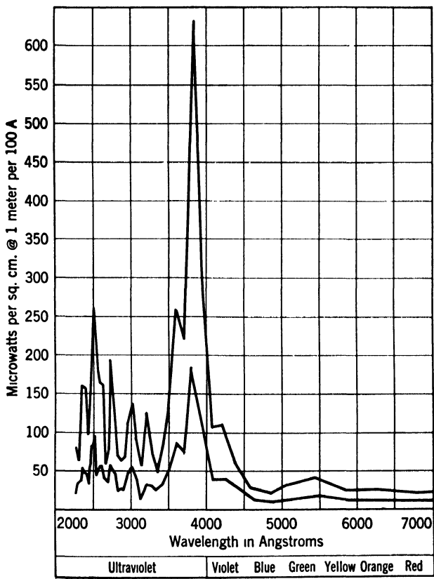
FIG. 33. Spectral energy distribution of carbon arc with iron-cored carbons (National B). Upper curve, 60 amperes alternating current, 50 volts across arc. Lower curve, 30 amperes alternating current, 50 volts across arc. ( National Carbon Co. Catalog, Section A-4300. )
