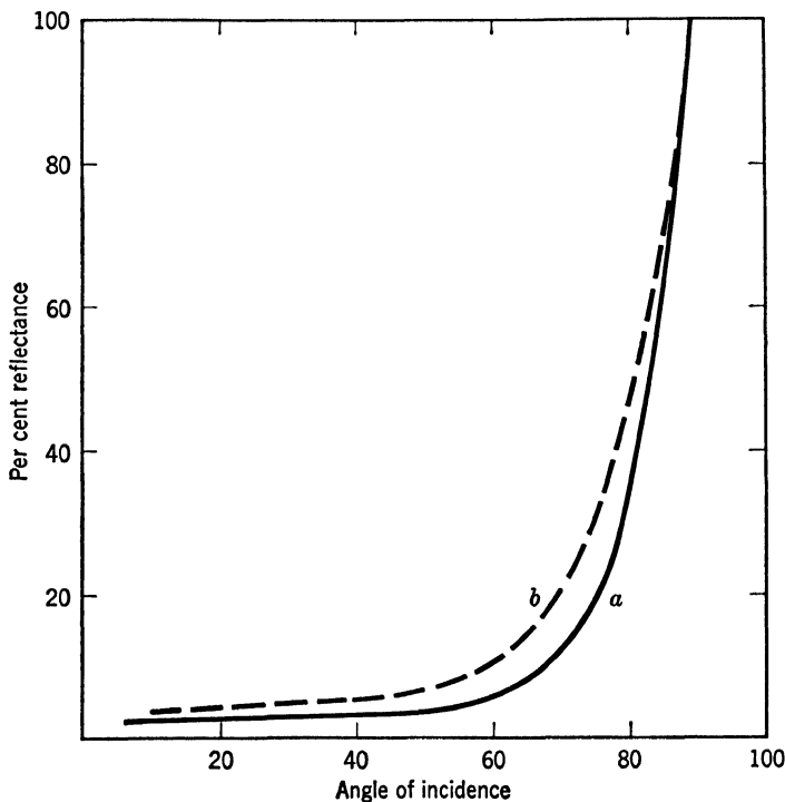
FIG. 13. a . Reflection of ultraviolet (3082 A) from the surface of glass at various angles of incidence. b . Reflection of ultraviolet from the surface of water at various angles of incidence.
