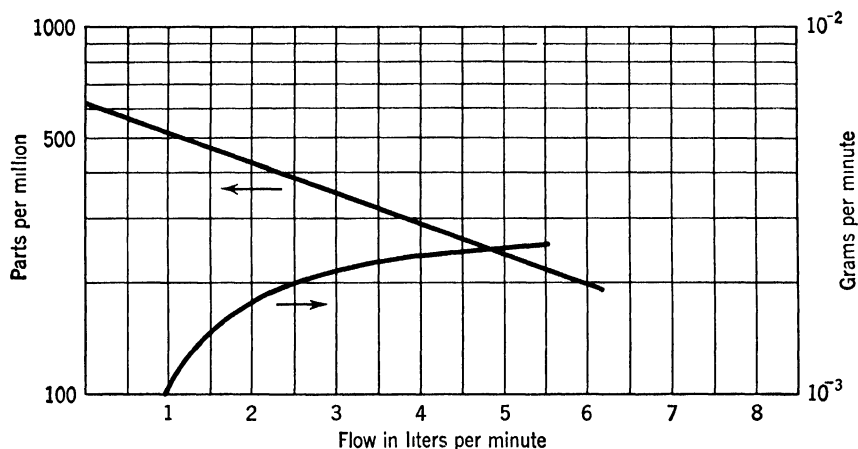
FIG. 13. Concentration of ozone produced from oxygen by low-pressure mercury quartz arc as a function of rate of flow of oxygen. (L. R. Koller, J. Applied Phys. , 16 , 816, 1945.)
