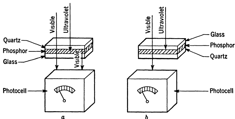
FIG. 14. Luckiesh-Taylor conversion-type ultraviolet meter.
