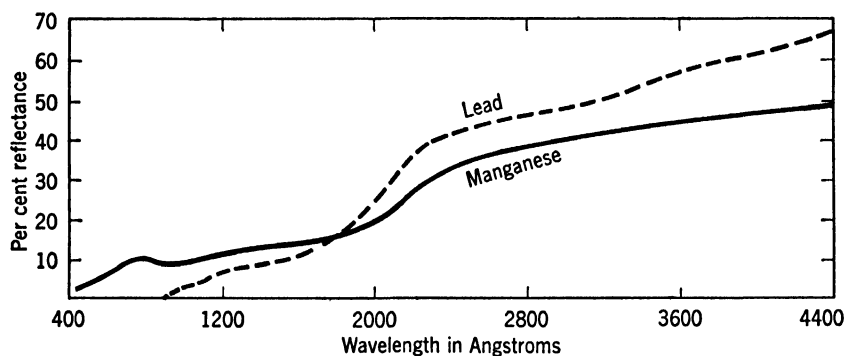
FIG. 5. Reflection from evaporated films of lead and manganese. (J. B. Sabine, loc. cit.)
