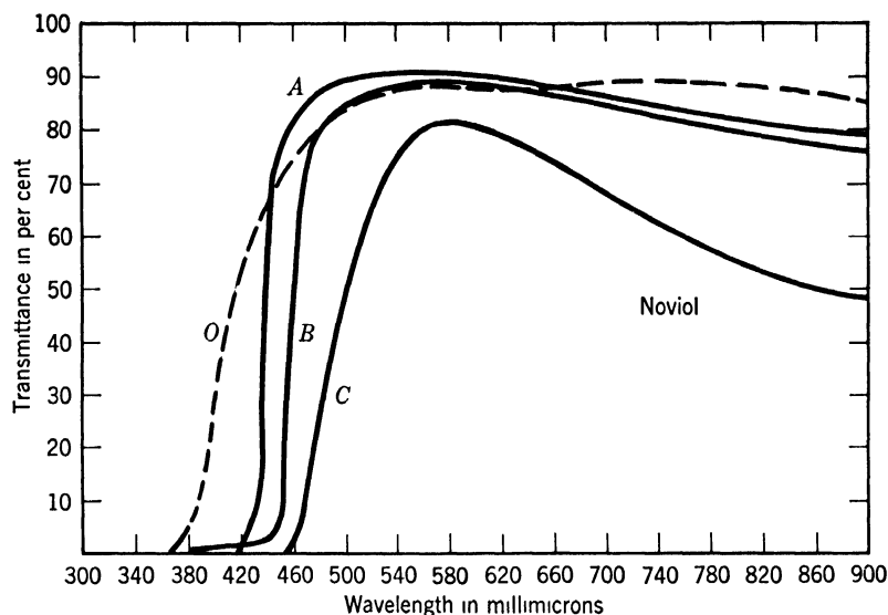
FIG. 21. Spectral transmittance of Noviol glass. Noviol O, thickness 2.63 mm. Noviol A, thickness 1.90 mm. Noviol B, thickness 2.89 mm. Noviol C, thickness 3.05 mm. ( Natl. Bur. Standards Circ. 471, 1948. )
