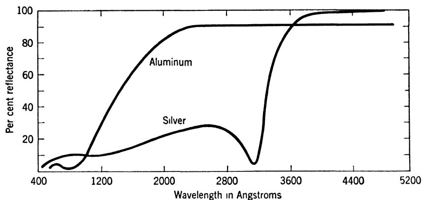
FIG. 3. Reflection from evaporated films of silver and aluminum. (J. B. Sabine, Phys. Rev. , 55 , 1064, 1939.)
