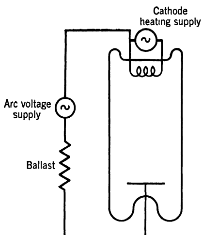
FIG. 8. Arc with separately excited cathode.
