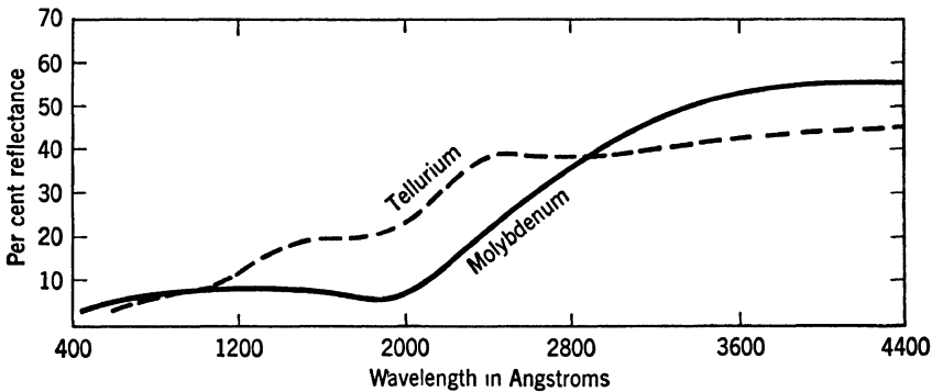
FIG. 8. Reflection from evaporated films of molybdenum and tellurium. (J. B. Sabine, loc. cit.)
