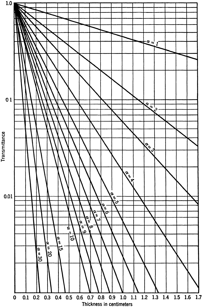
FIG. 2. Transmittance as a function of thickness for various values of absorption coefficient.
