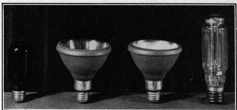
FIG. 16. High-pressure mercury lamps using the same type of arc in different types of bulbs. (Courtesy of General Electric Co.)
