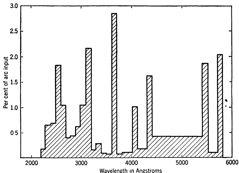
FIG. 12. Energy distribution in spectrum of UA-2 mercury vapor arc in quartz. ( Gen. Elec. Lamp Bulletin LD-1. )
