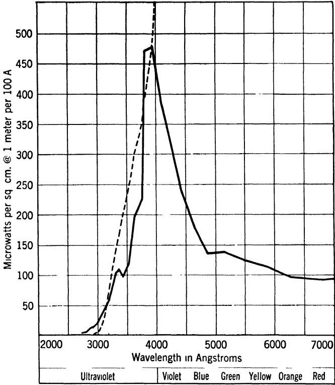
FIG. 32. National Sunshine Carbon with Corex filter compared with natural sunlight. Solid line, with Corex D filter. Dotted line, natural sunlight. ( National Carbon Co. Catalog, Section A-4300. )
