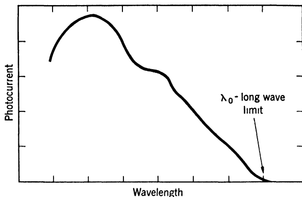
FIG. 6. Phototube spectral response curve.
