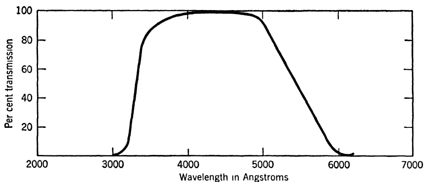
FIG. 15. Transmission of cupric sulfate: 5 cm of solution of \text{CuSO}_4 \cdot 5\text{H}_2\text{O} , 100 grams per liter. (M. Kasha, J. Optical Soc. Am. , 38 , 929, 1948.)
