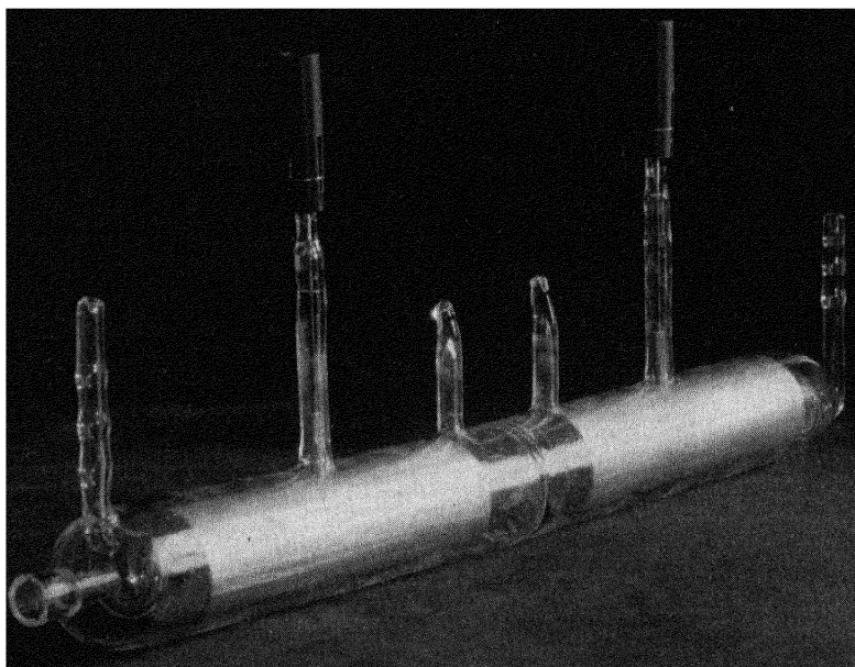
FIG. 27. Hydrogen arc in quartz. Emission is through windows at ends of tube. Vertical tubes at end are for water circulation. (Courtesy of Hanovia Chemical and Mfg. Co.)
