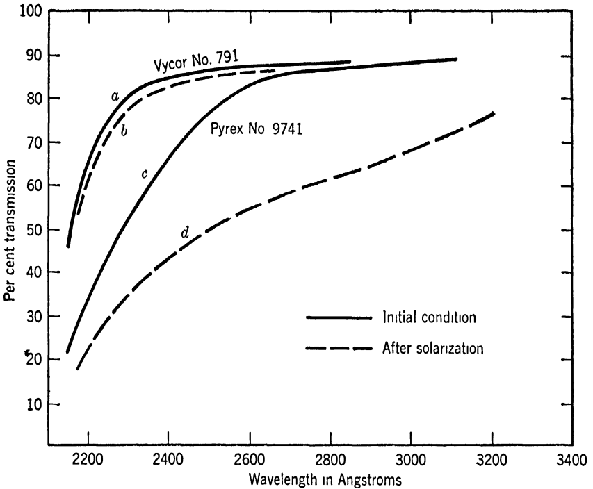
FIG. 11. Effect of solarization on Vycor and Pyrex glasses. (M. E. Nordberg, J. Am. Ceram. Soc. , 30 , 174, 1947.)
