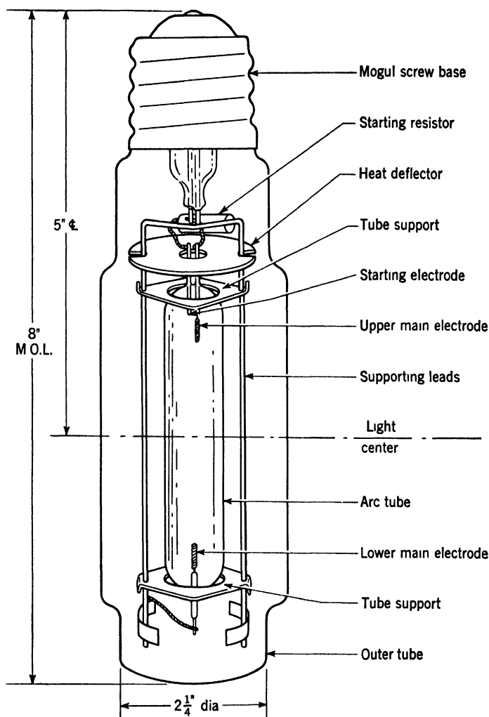
FIG. 15. Construction of a typical high-pressure mercury arc. (Courtesy of General Electric Co.)
