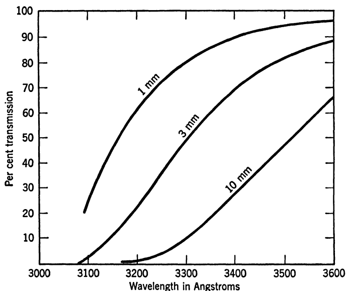
FIG. 4. Transmission for various thicknesses of window glass.
