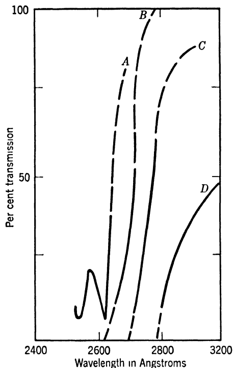
FIG. 12. Transmission of filters of various concentrations of benzene dissolved in octane. A. 1.0 grams per liter. B. 9.1 grams per liter. C. 100 grams per liter. D. Undiluted. (A. N. Bass, J. Optical Soc. Am. , 38 , 977, 1948.)
