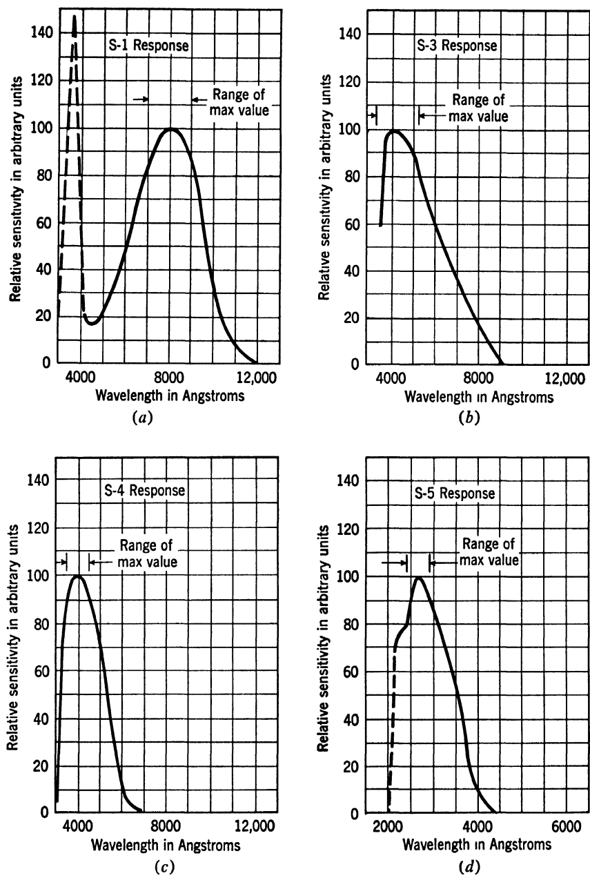
FIG. 8. Spectral response curves of various commercial phototubes. a-d. RCA Bulletin CRPS-102-A.
