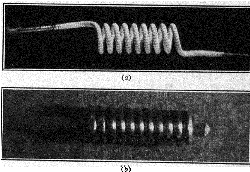
FIG. 7. Various forms of thermionic cathodes. a. Overwound oxide-coated cathode. b. Thorium-insert cathode. (Courtesy of General Electric Co.)
