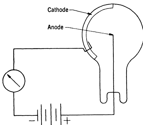
FIG. 1. Photoelectric tube and circuit.
