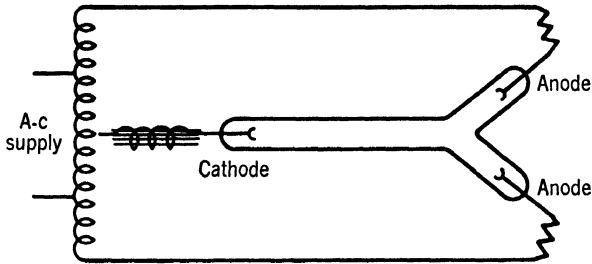
FIG. 10. A-c operated pool-type mercury arc.
