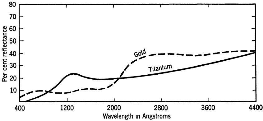
FIG. 7. Reflection from evaporated films of gold and titanium. (J. B. Sabine, loc. cit.)
