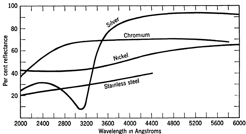
FIG. 1. Reflection from silver, chromium, nickel, and stainless steel. (M. Luckiesh, J. Optical Soc. Am. , 19 , 1, 1929.)
