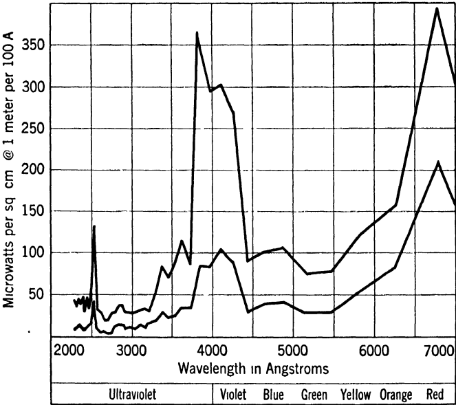
FIG. 36. Spectral energy distribution of carbon arc with strontium-cored carbons (National E). Upper curve, 60 amperes alternating current, 50 volts across arc. Lower curve, 30 amperes alternating current, 50 volts across arc. ( National Carbon Co. Catalog , Section A-4300.)
