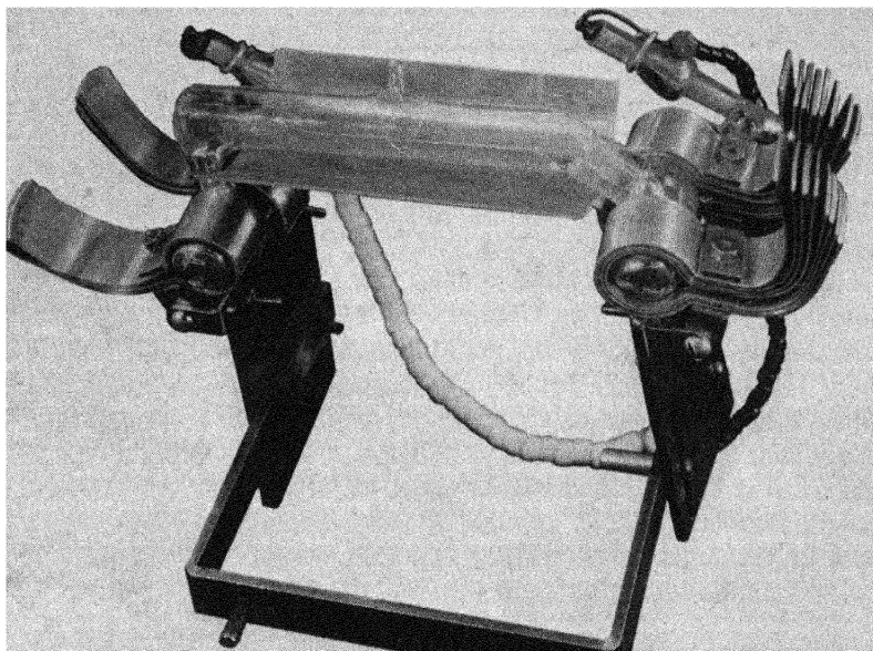
FIG. 9. Pool-type quartz mercury arc for vertical or horizontal operation. Now superseded. (Courtesy of Hanovia Chemical and Mfg. Co.)
