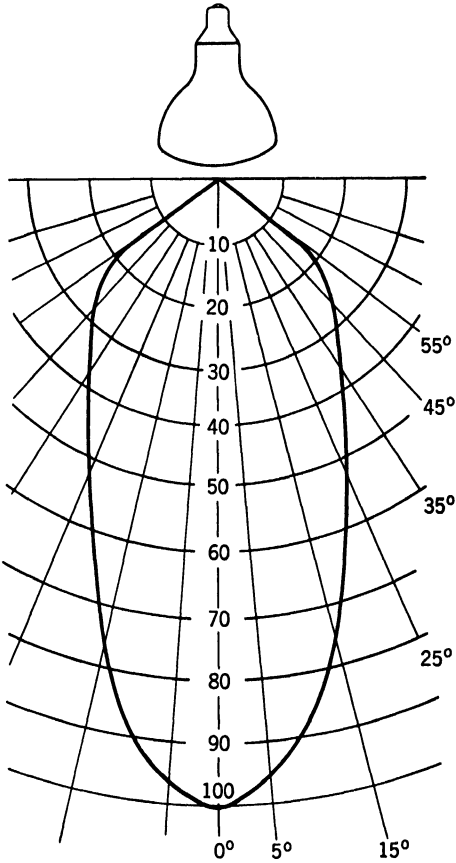
FIG. 17. Angular distribution of energy in the beam of the RS lamp. ( Gen. Elec. Lamp Bulletin LD-1. )
