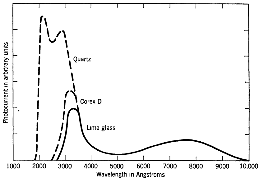
FIG. 9. Effect of envelope material on spectral response of S-1 photo surfaces. (V. K. Zworykin and E. G. Ramberg, Photoelectricity and Its Applications , John Wiley and Sons, New York, 1949.)
