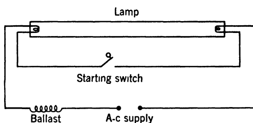
FIG. 21. Starting circuit for germicidal lamps.
