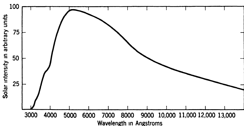
FIG. 12. Solar energy distribution for midsummer noonday sun in Washington, D. C. (Calculated from W. E. Forsythe, Measurement of Radiant Energy , McGraw-Hill Book Co., New York, 1937.)
