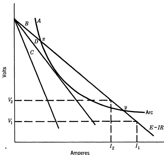
FIG. 4. Conditions for stability of an arc. (P. Copeland and W. H. Sparing, J. Applied Phys. , 16 , 302, 1945.)
