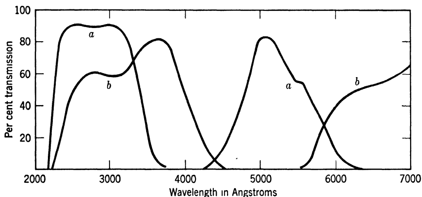
FIG. 13. Transmission of solutions of nickelous and cobaltous sulfate. a. 1 cm of \text{NiSO}_4 \cdot 6\text{H}_2\text{O} , 500 grams per liter. b. 1 cm of \text{CoSO}_4 \cdot 7\text{H}_2\text{O} , 300 grams per liter. (M. Kasha, J. Optical Soc. Am. , 38 , 929, 1948.)
