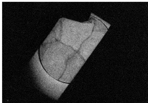
FIG. 9. Fluorescence excited in willemite by 2138 Å radiation after passing through fused quartz. The dark portions represent opacities in the quartz. (Courtesy of E. A. Taft.)
