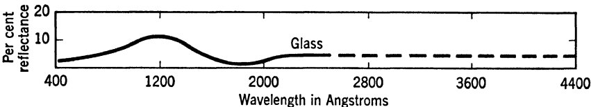
FIG. 12. Reflection from glass at normal incidence. (J. B. Sabine, loc. cit.)
