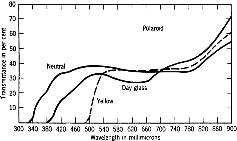
FIG. 22. Spectral transmittance of Polaroid glasses. Neutral Polaroid, thickness 5.20 mm. Polaroid Day glass, thickness 2.28 mm. Yellow Polaroid, thickness 5.65 mm. ( Natl. Bur. Standards Circ. 471, 1948. )
