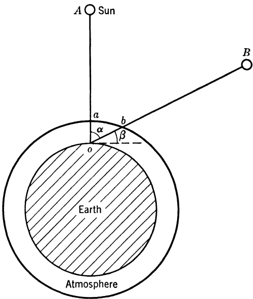
FIG. 2. Relation between air mass and solar elevation.
