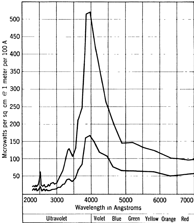
FIG. 31. Spectral energy distribution of carbon arc with cerium-cored carbons (National Sunshine). Upper curve, 60 amperes alternating current, 50 volts across arc. Lower curve, 30 amperes alternating current, 50 volts across arc. ( National Carbon Co. Catalog, Section A-4300. )
