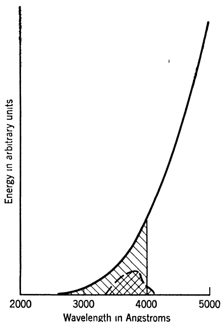
FIG. 4. Effect of filter on radiation from incandescent lamp. Shaded region, available ultraviolet energy; cross-hatched region, ultraviolet transmitted by filter.
