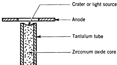
FIG. 25. Electrodes of zirconium concentrated arc.
