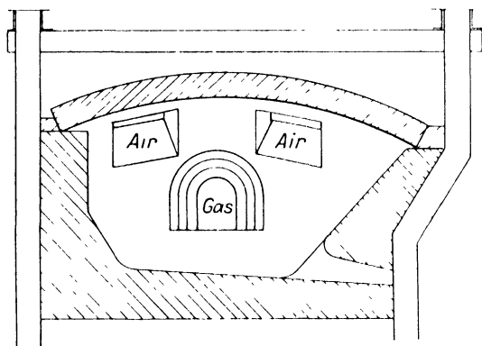
FIG. 72. Twin air ports
