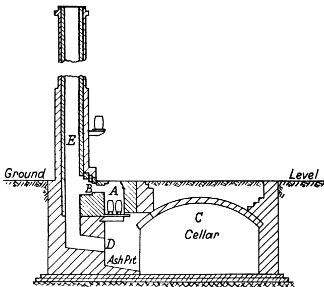
FIG. 177. Crucible furnace.
