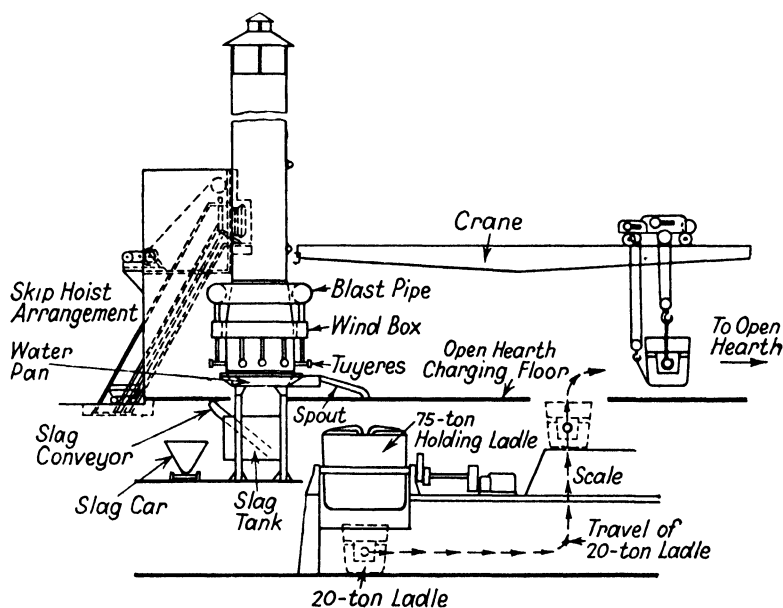
FIG. 173. Cupola plant. (By courtesy of "Iron Age".)
