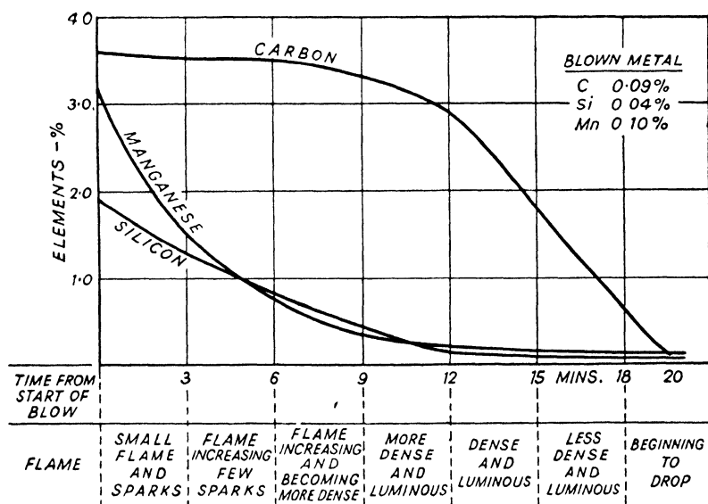
FIG. 12. Progress of high-manganese blow.
