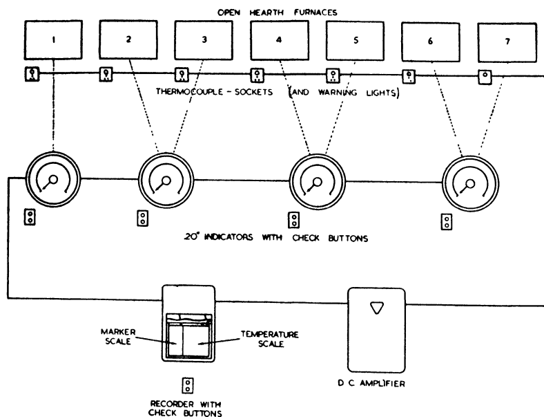
FIG. 212. Multi-point immersion pyrometer system.
