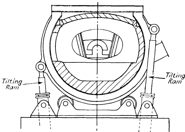
Section thro' Tilting Furnace
