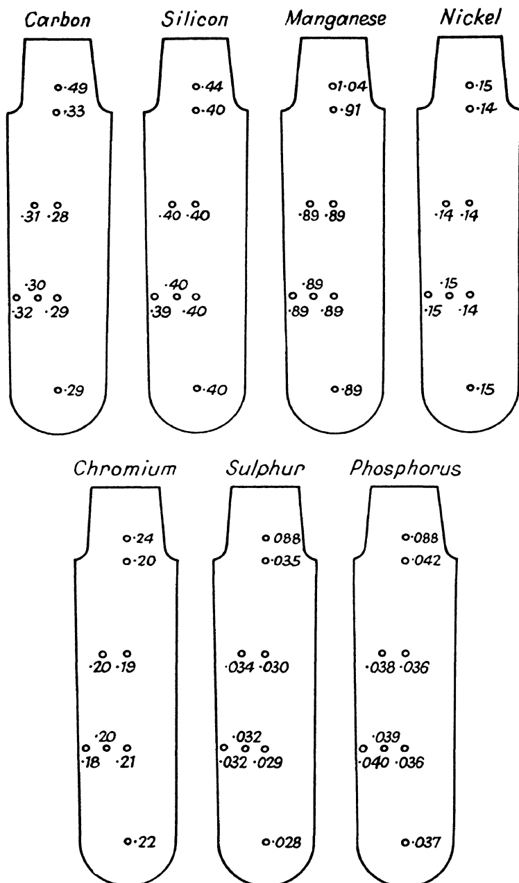
FIG. 164. Typical segregation—(killed steel). (Fourth Ingot Report—by courtesy of the Iron and Steel Institute.)
