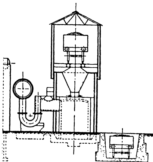
FIG. 59. Producer plant layout.
