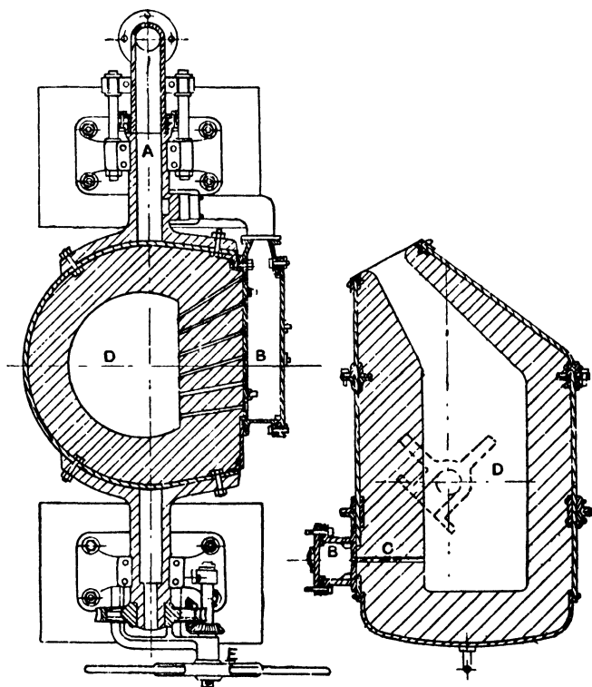
FIG. 167. Typical side-blown converter showing wind-box.
