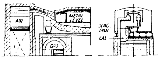
FIG. 74. Moll port. (By courtesy of the "British Steelmaker")
