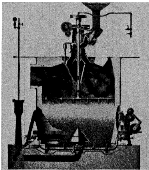
FIG. 54. Chapman gas machine.
