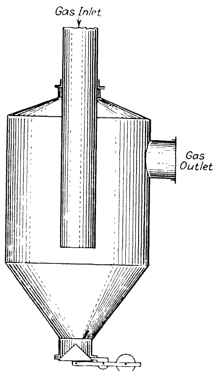
FIG. 60. Dustcatcher.
