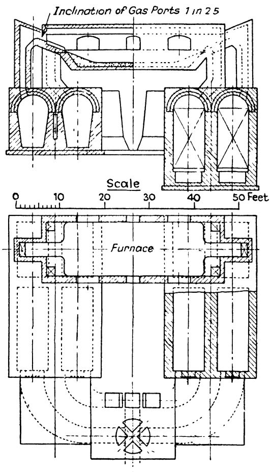
FIG. 22. Reverberatory furnace.
