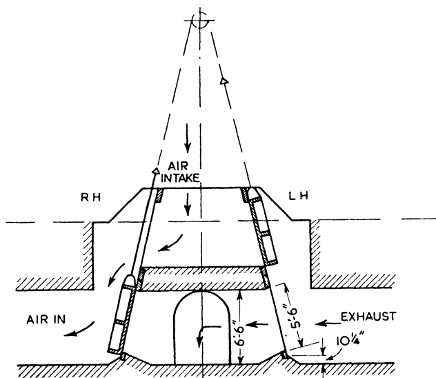
FIG. 29. Damper-type air valve.
