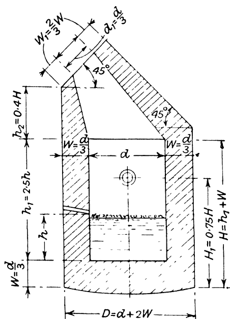
FIG. 171. Goldsbrough and Throssell converter design diagram.
