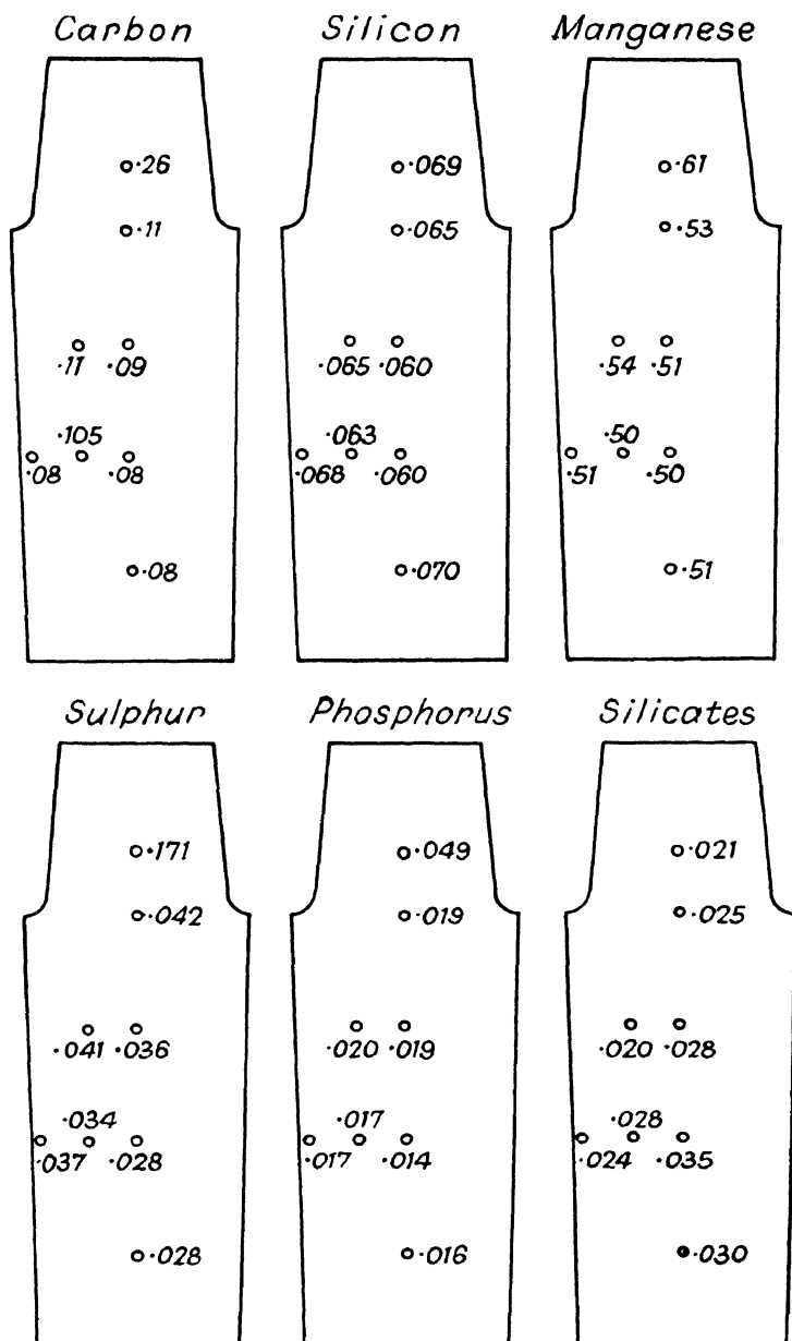
FIG. 166. Segregation in semi-killed steel. (Fourth Ingot Report—by courtesy of the Iron and Steel Institute.)
