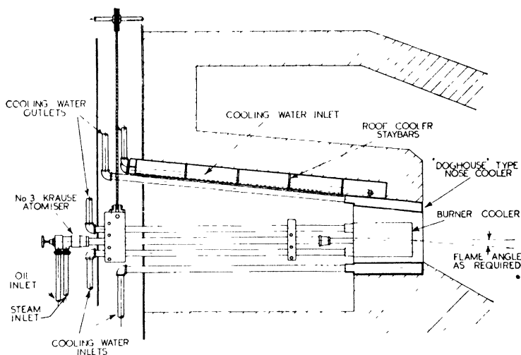
FIG. 65. Blaw-Knox oil burner. (By courtesy of "Metallurgia")
