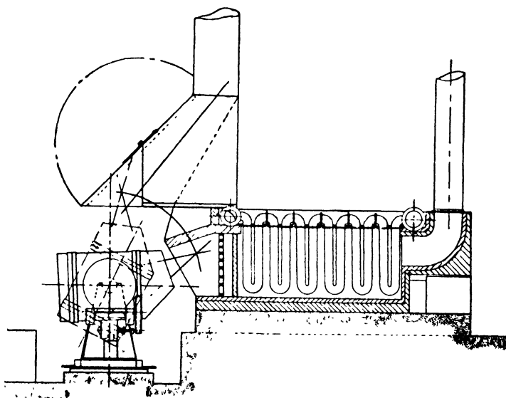
FIG. 169. Stock converter.
