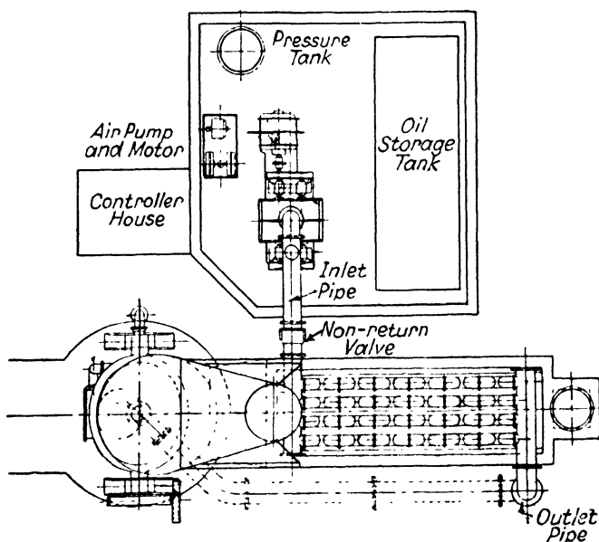
FIG. 170. Stock converter layout.
