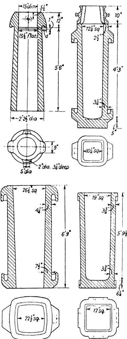
FIG. 139. Typical ingot moulds (various sources).
