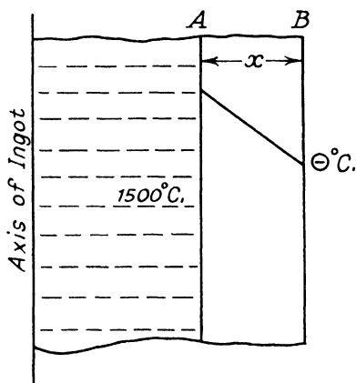
FIG. 155. Heat flow through mould wall. (McCance.)
