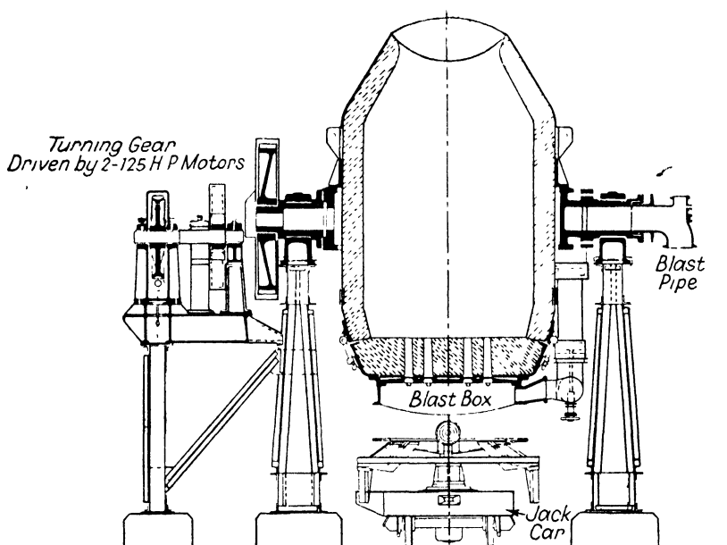
FIG. 7. A typical 25-ton acid converter.
