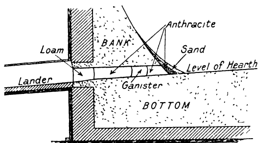
FIG. 105 Section through an acid open-hearth furnace. (From "Practical Steelmaking", by W. Tister, by courtesy of the author.)
