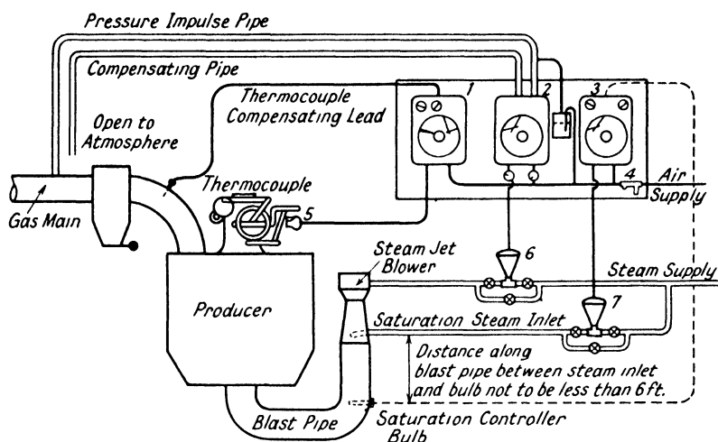
FIG. 207. General principles of gas pressure regulator.
