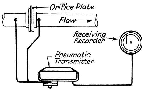
FIG. 187. Electroflo flow meter installation.
