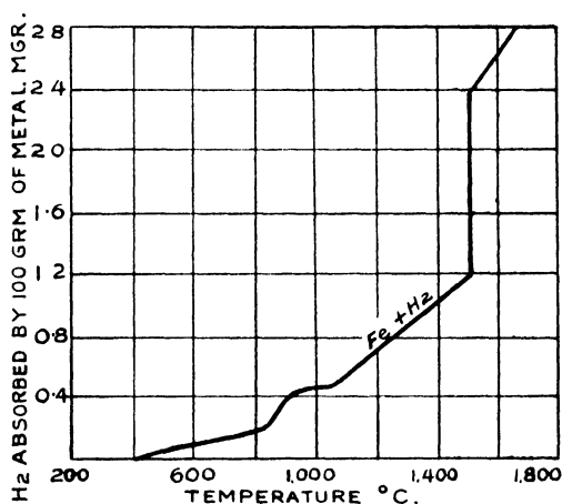
FIG. 149. Solubility of hydrogen in steel. (Sievert.)
