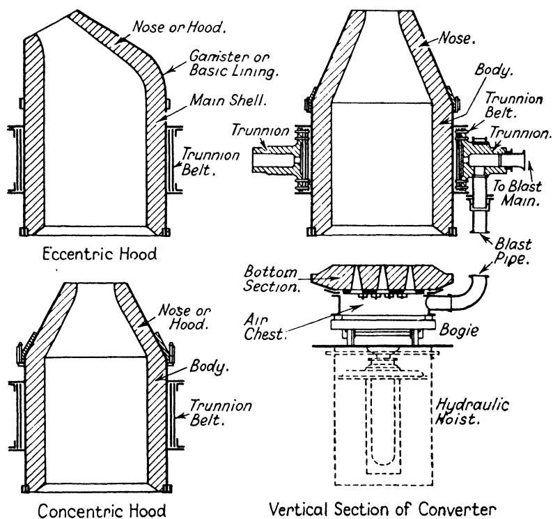
FIG. 4. Bessemer converter.
