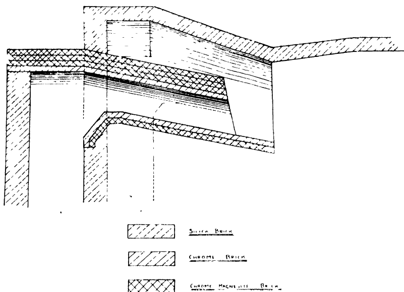
FIG. 73 Conventional fan port (By courtesy of the "British Steelmaker")
