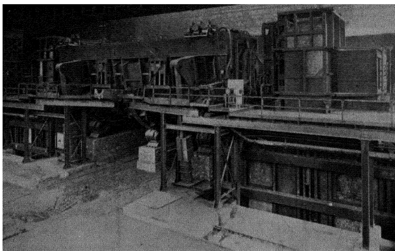
FIG. 89. Tapping-side of a 300-ton tilter.
