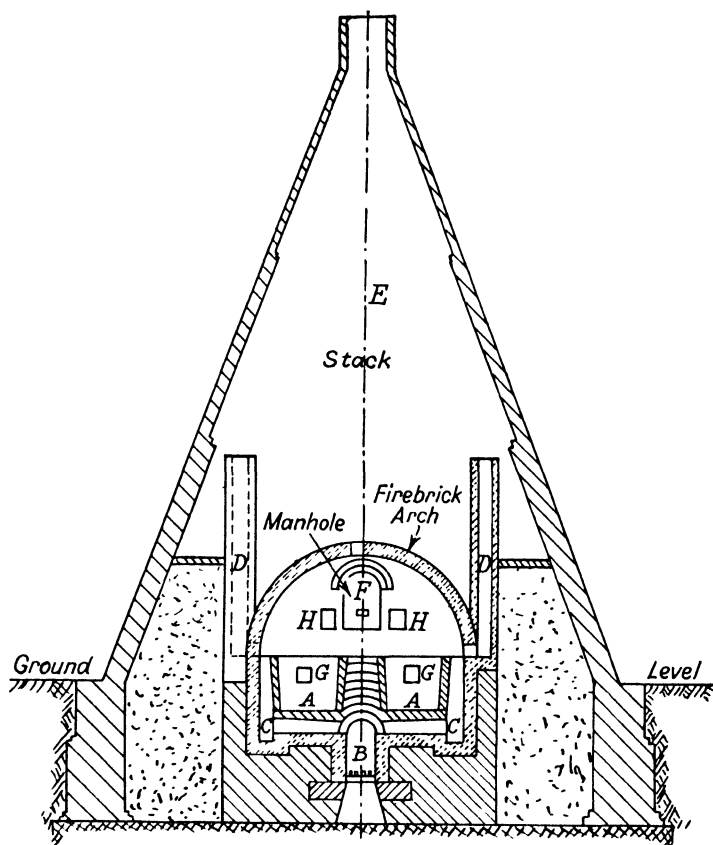
FIG. 176. Cementation furnace.
