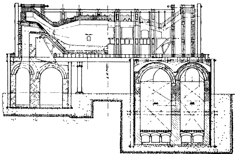
FIG. 69. A 90-ton fixed open-hearth furnace (By courtesy of the Iron and Steel Institute)
