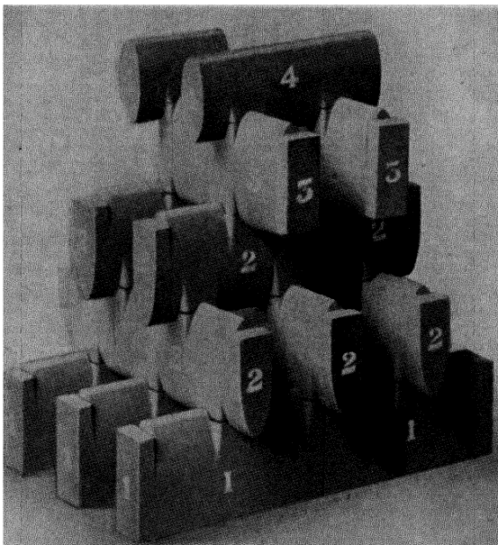
FIG. 70. Special checker-bricks.
