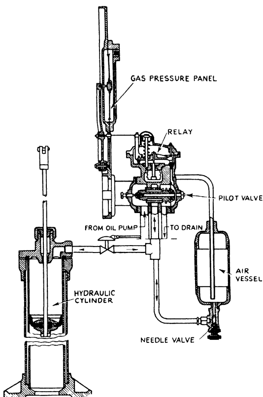
FIG. 56. Arka gas regulator.
