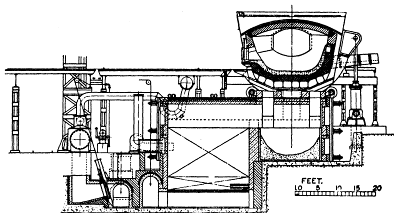
FIG. 88. 300-ton tilting furnace—cross-section.
