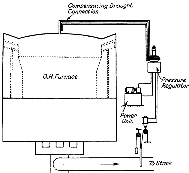
FIG. 192. Furnace pressure control—general arrangement.
