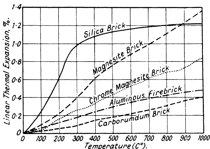
FIG. 218. Linear expansion of refractories.
