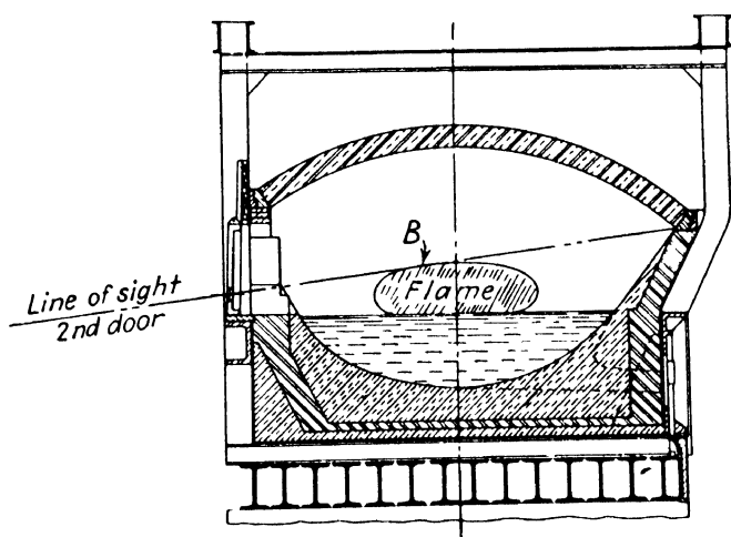
FIG. 68. Flame position in an oil-fired O. H. furnace.
