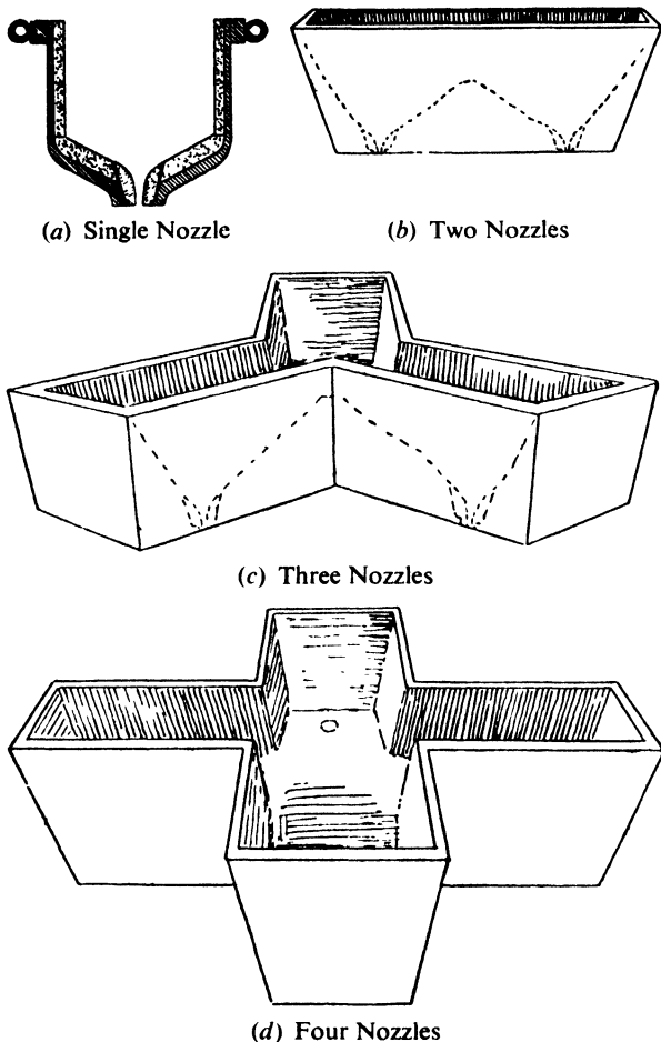
FIG. 142. Tundish design.
