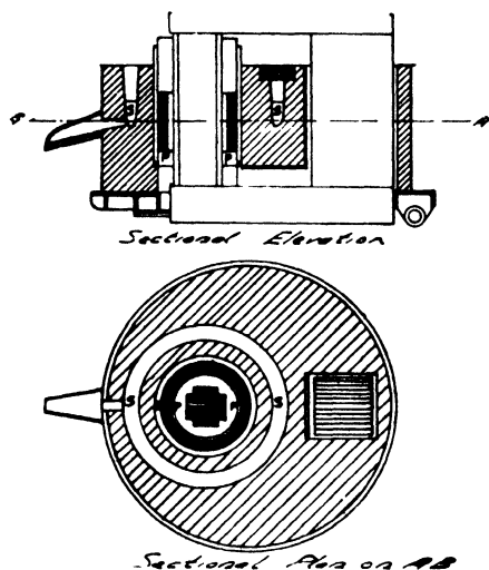
FIG. 125. Kjellin induction furnace.
