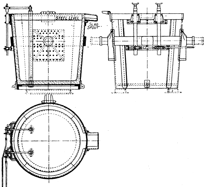
FIG. 135. Casting ladle.
