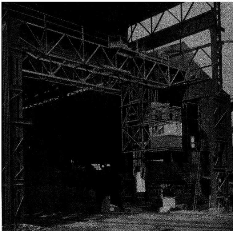
FIG. 133. Stripping crane.
