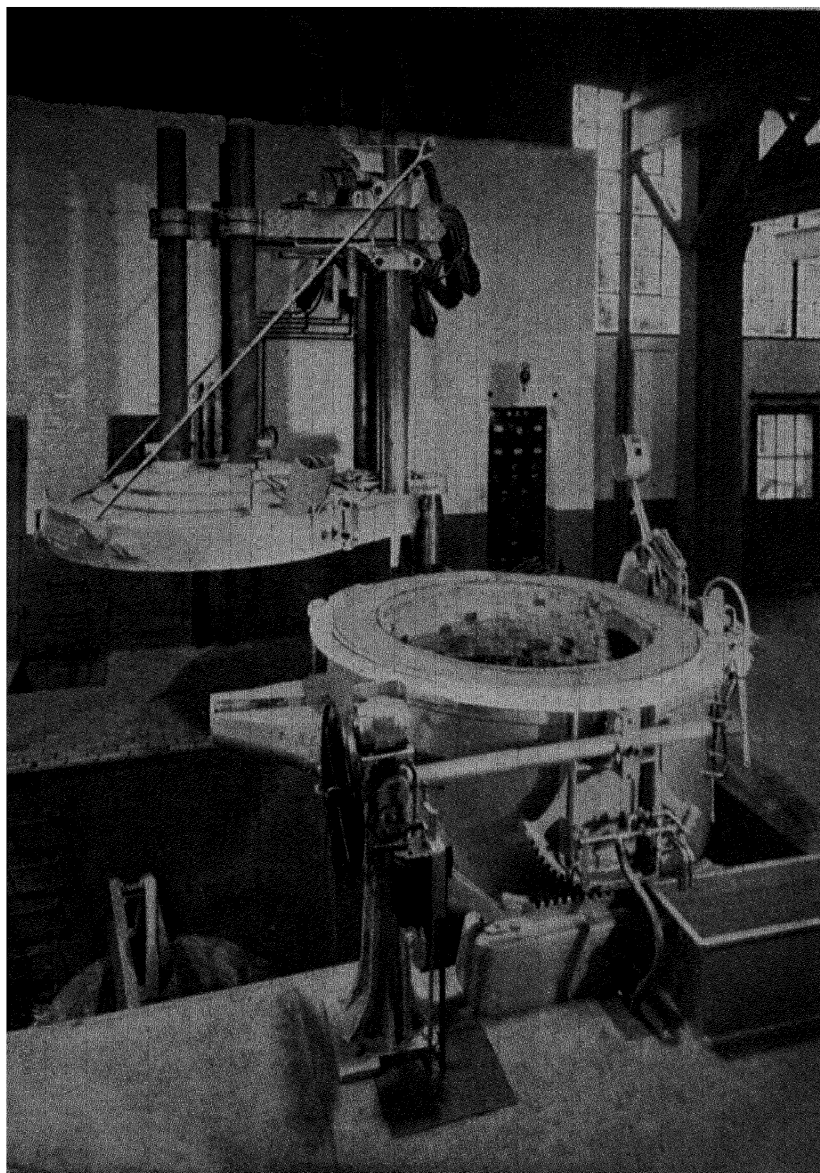
FIG. 122. Swing-roof type electric arc furnace.
