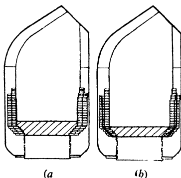
FIG. 20B. New type brick lining in shallow bath converter (a) start of first bottom and (b) wear during life start of fourth bottom (after Dickie).
