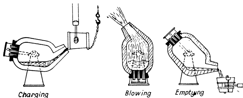
FIG. 5. The stages of the Bessemer process.
