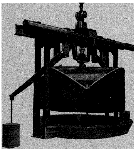
FIG. 26. Lake gas valve.
