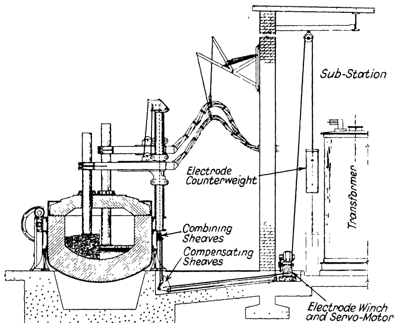
FIG. 118. "Electromelt" electrode-control.
