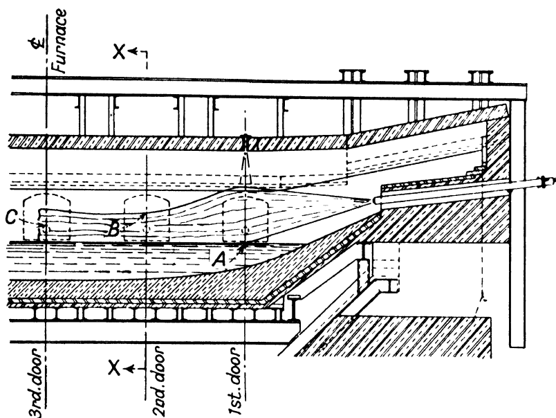
FIG. 67. Flame position in an oil-fired O. H. furnace.
