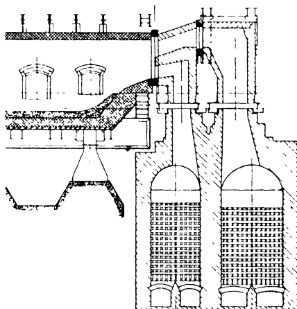
FIG. 92 Removable blocks for tilting furnaces.
