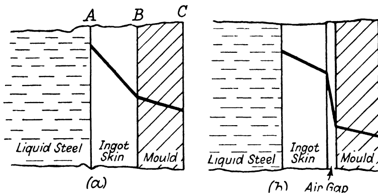
FIG. 156. Effect of air gap in ingot cooling. (McCance.)
