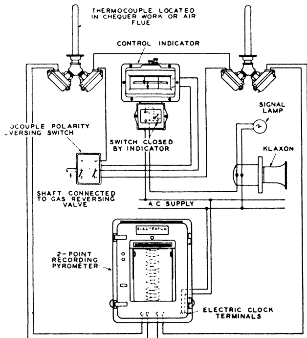
FIG. 194. Reversal control—Syren system.
