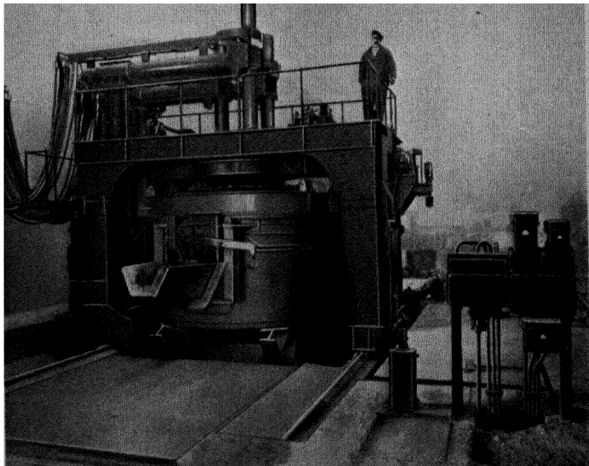
FIG. 123. A 12-ton Siemens-Halske arc furnace with removable cover.
