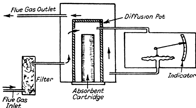
FIG. 190. Diffusion type \text{CO}_2 indicator. (From "Efficient Use of Fuel" by courtesy of H. M. Stationery Office.)
