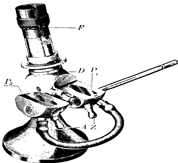
The Butter Refractometer, with the water-jacketed double prism P^1 P^2 ; the box-shaped centre part D and the telescope F .
