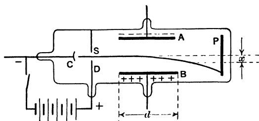
FIG. 128.--Determination of \frac{e}{m} for Cathode Rays, Electrostatic Deflection.
