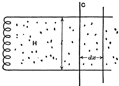
FIG. 97.—Calculation of the Magnitude of an Induced E.M.F.
