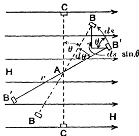
FIG. 101.—Theory of the Simple Dynamo.
