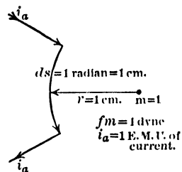
FIG. 17.—Definition of Unit Current.
