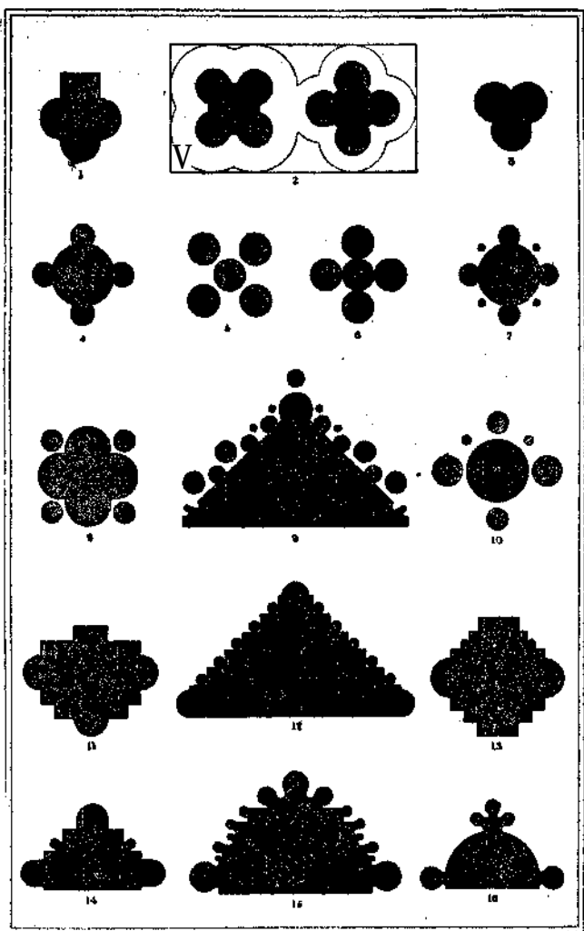
PLATE II. PLANS OF PIERS.
