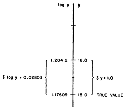
FIG. 9. Illustrating the relation between an error in y and an error in \log y . Here y changes by unity, and \log y changes by 0.02803. The approximate relation \delta \log y = 0.434 \delta y/y gives 0.02895, which is to be compared with the exact value 0.02803. Smaller changes (smaller values of \delta y ) show better agreement, but even for this rather large value of \delta y the approximate relation would be adequate for many purposes. (See Exercise 8c, p. 44.)
