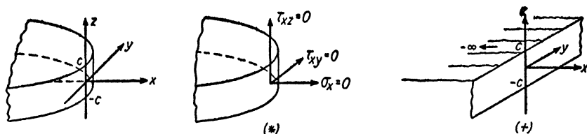
FIG. 1. Elastic plate, free along section of edge.
