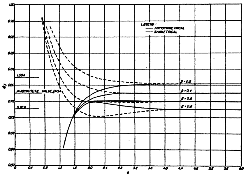
FIG. 4. Q_I vs. q for symmetrical and antisymmetrical wrinkling with \sigma = 0.25 , and \beta = 0.2, 0.4, 0.6 , and 0.8 .
