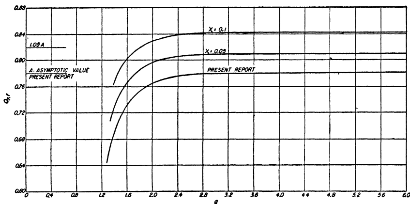
FIG. 6. Comparison of critical values Q_{xf} from the Cox formula with those from the present report for antisymmetrical wrinkling. \sigma = 0.25 , \beta = 0.4 .
