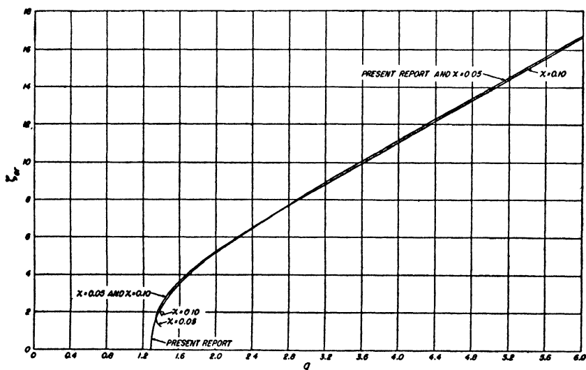
FIG. 7. Comparison of values of \zeta_{cr} as obtained by the Cox formula with those obtained by the formula of the present report for antisymmetrical wrinkling. \sigma = 0.25 ; \beta = 0.4 . NOTE: When \zeta is shown as a two-valued function of q , the smaller value corresponds to a relative maximum.
