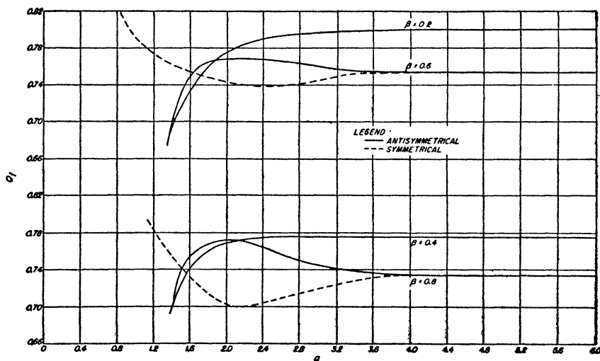
FIG. 5. Q_f vs. q for symmetrical and antisymmetrical wrinkling with \sigma = 0.5 , and \beta = 0.2, 0.4, 0.6 , and 0.8 .
