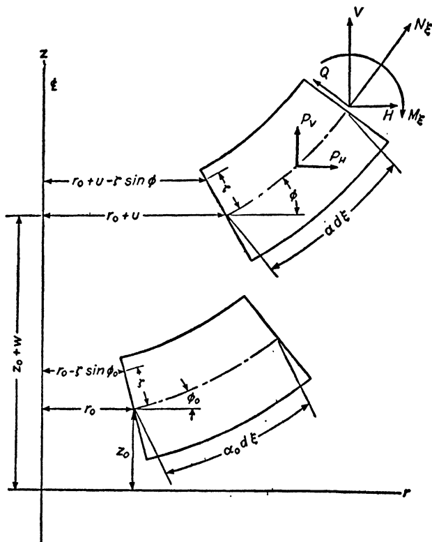
FIG. 1. Side view of element of shell in undeformed and in deformed state. Also shown are visible stress resultants and couples and load intensity components.
