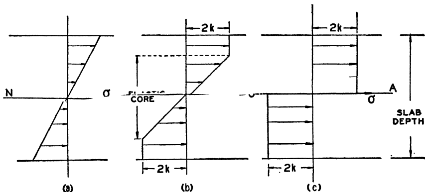
FIG. 5. Development of the stress distribution in a bent slab.
