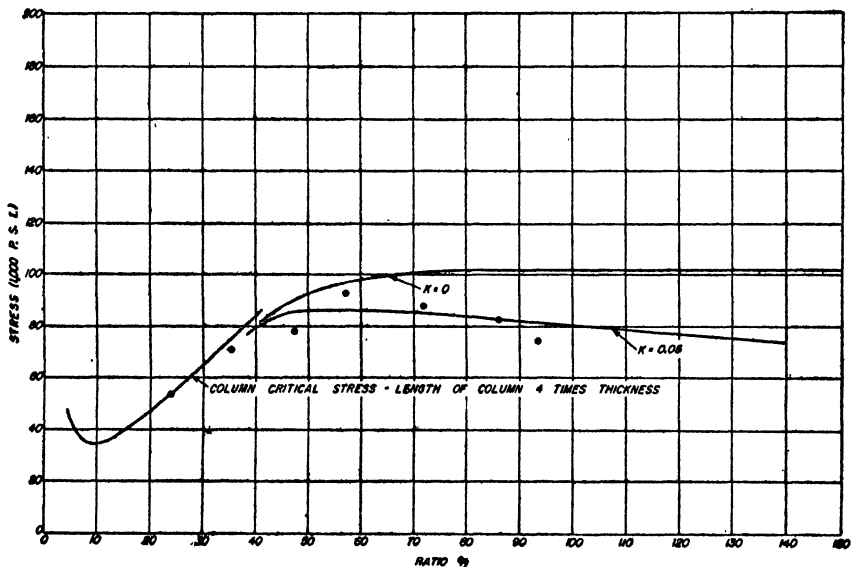
FIG. 11. Sandwich constructions having 0.01-in. steel facings and cellular cellulose acetate cores (flatwise). Curves represent computed values. Each plotted point represents the average of four specimens.
