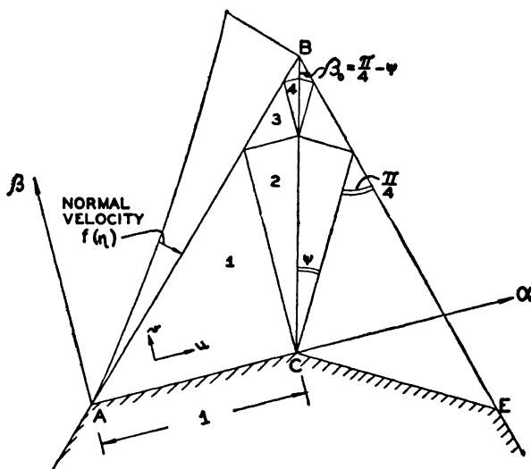
Fig. 3. Slip-line field for uniform pressure on one face of an acute-angled wedge.
