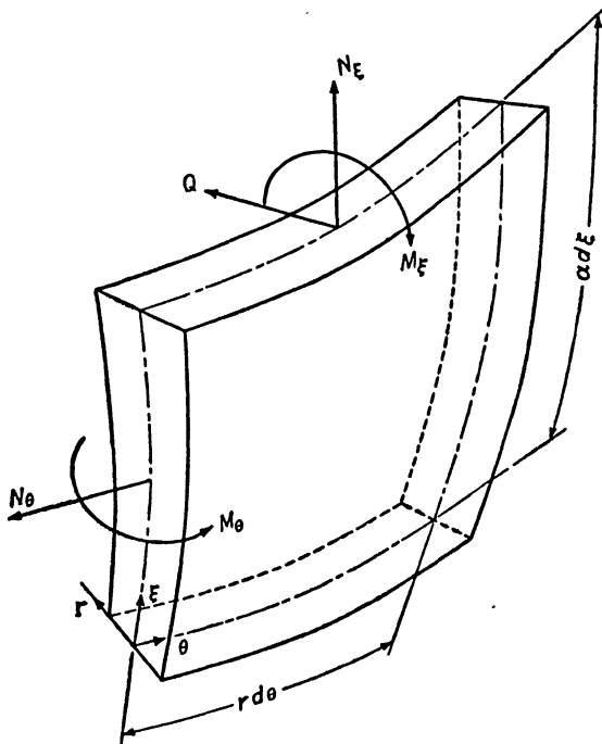
FIG. 2. Element of shell showing stress resultants and stress couples.
