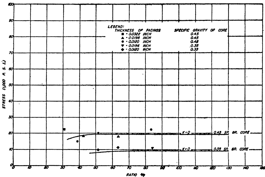
FIG. 10. Sandwich constructions having aluminum facings and cork cores. Curves represent computed values, and each plotted point represents the average of 10 test specimens.
