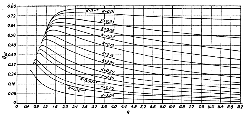
FIG. 9. Plot of Q_N vs. q for various values of K . Initial amplitude proportional to core thickness. \sigma = 0.25 , \beta = 0.4 .
