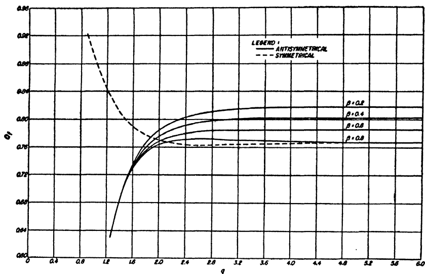
FIG. 3. Q_I vs. q for symmetrical and antisymmetrical wrinkling with \sigma = 0 , and \beta = 0.2, 0.4, 0.6 , and 0.8 .
