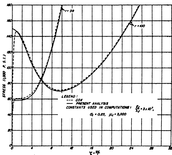
Fig. 8. Comparison of graphs of stress in facings vs. \zeta obtained by the Cox formula with those obtained by the formula of the present report. Isotropic facings and core.
