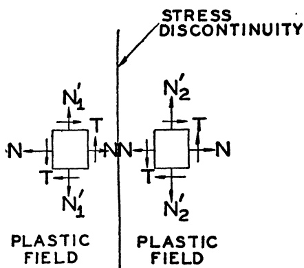
FIG. 2. Stress components at a discontinuity of stress.
