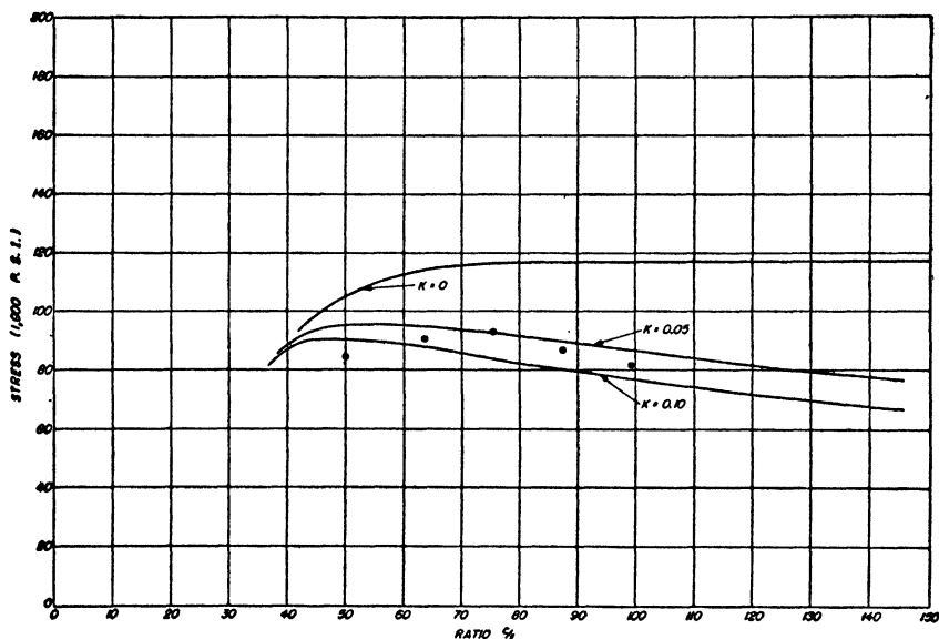
FIG. 12. Sandwich constructions having 0.01-in. steel facings and cellular cellulose acetate cores (edgewise). Curves represent computed values, and each plotted point represents the average of four specimens.
