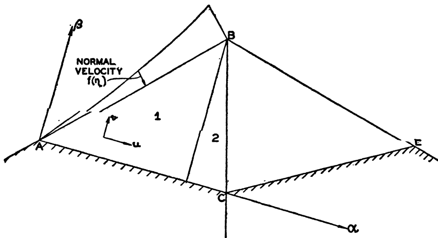
Fig. 6. Slip-line field for uniform pressure on one face of an obtuse-angled wedge.
