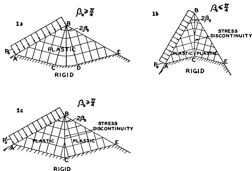
FIG. 1. Slip-line fields for uniform pressure on one face of a wedge.
