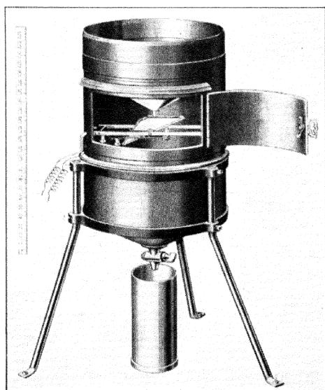
FIG. 75. Tipping-bucket rain gage.
