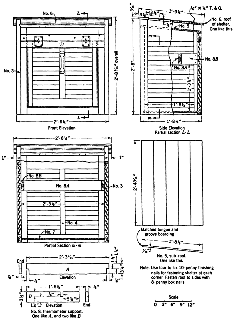
FIG. 88. Instrument-shelter details.
