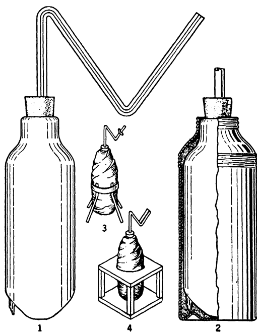
FIG. 97. Vacuum-bottle variometer.
