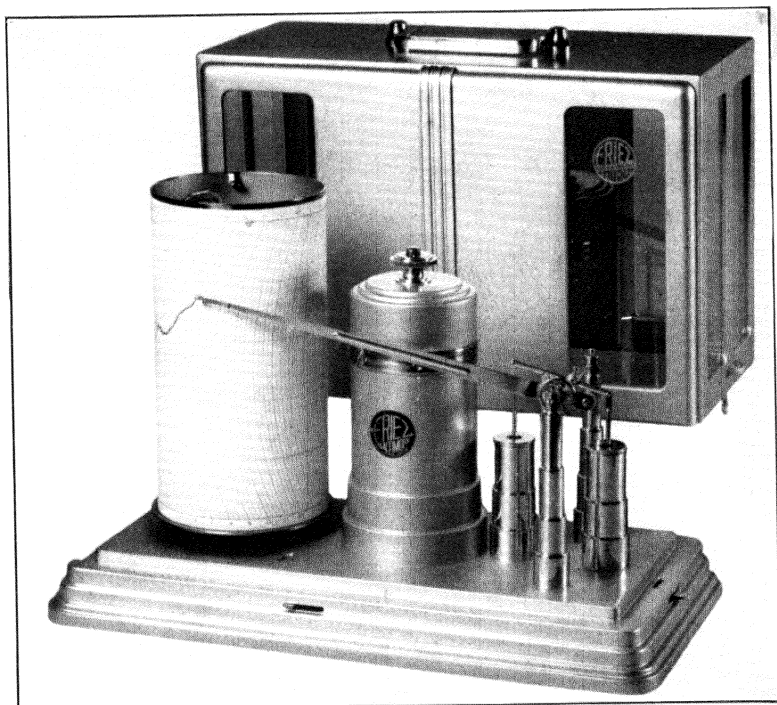
FIG. 70. Aneroid barograph.
