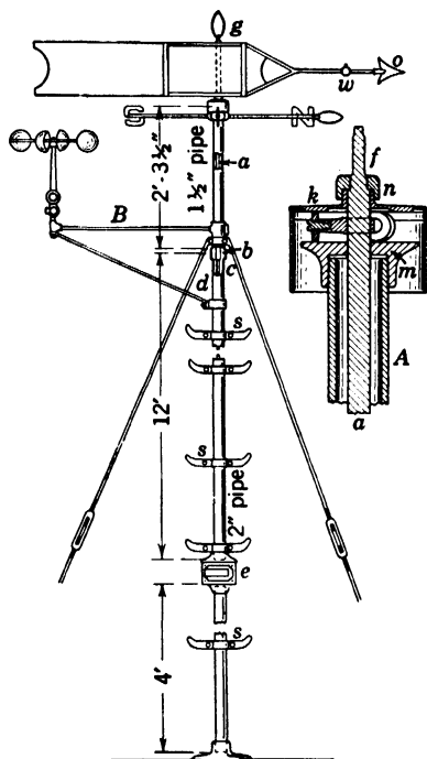
FIG. 57. Anemometer and wind vane on support; a axis of vane (solid iron rod); b coupling; c joint; d indicates where one end of pipe is screwed firmly into the lower end of the solid rod of the vane; e contact box; f indicates where axis rod is squared; g spearhead nut; k carrier or frame for antifriction rollers; m cap; n shoulder formed on rod; o arrow point; w counterweight; B cross-arm support for anemometer; s foot rests; A support pipe and vane bearing detail.
