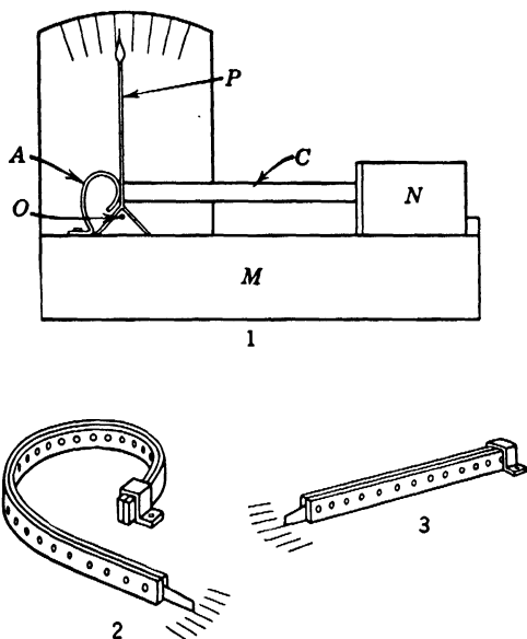
FIG. 98. Bimetallic thermometer.
