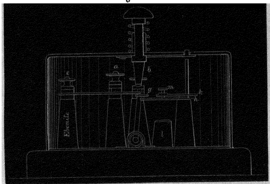
Section on line s, t, w .
