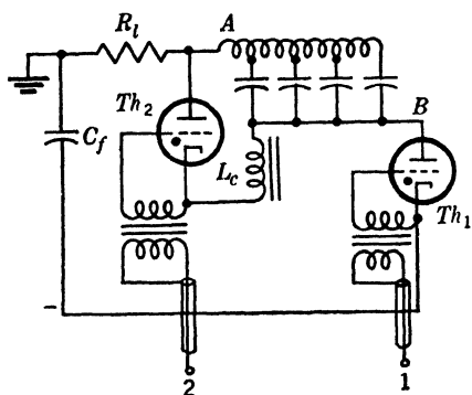
FIG. 11-18.—The Anger circuit with a hold-off thyatron.
