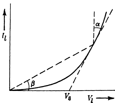
FIG. 3-16.—Current-voltage characteristic of a nonlinear load.
