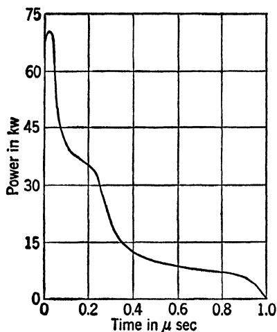
FIG. 8-31.—Power dissipated in one WX3226 gap as a function of time for a single pulse.
