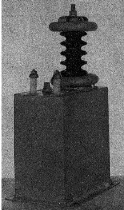
FIG. 15-37.—Porcelain solder-seal bushings on a 35-kv trigger transformer.
