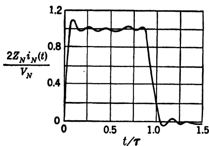
FIG. 6-27.—Calculated pulse shape for the five-section network of Fig. 6-22.
