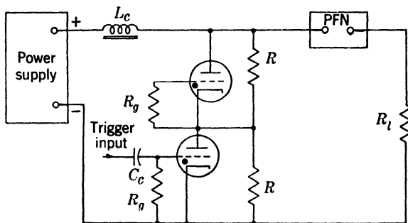
FIG. 8-42.—Series operation of thyratrons.
