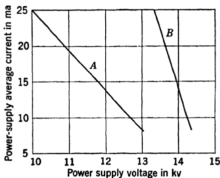
FIG. 5-7.—Regulation obtained with the voltage-doubler power supply used in a light-weight medium-power airborne pulser. Curve A is for 8 ohms in series and B is for no resistance in series with the primary of the power transformer.
