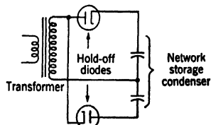
FIG. 9-30.—Two-diode charging circuit.
