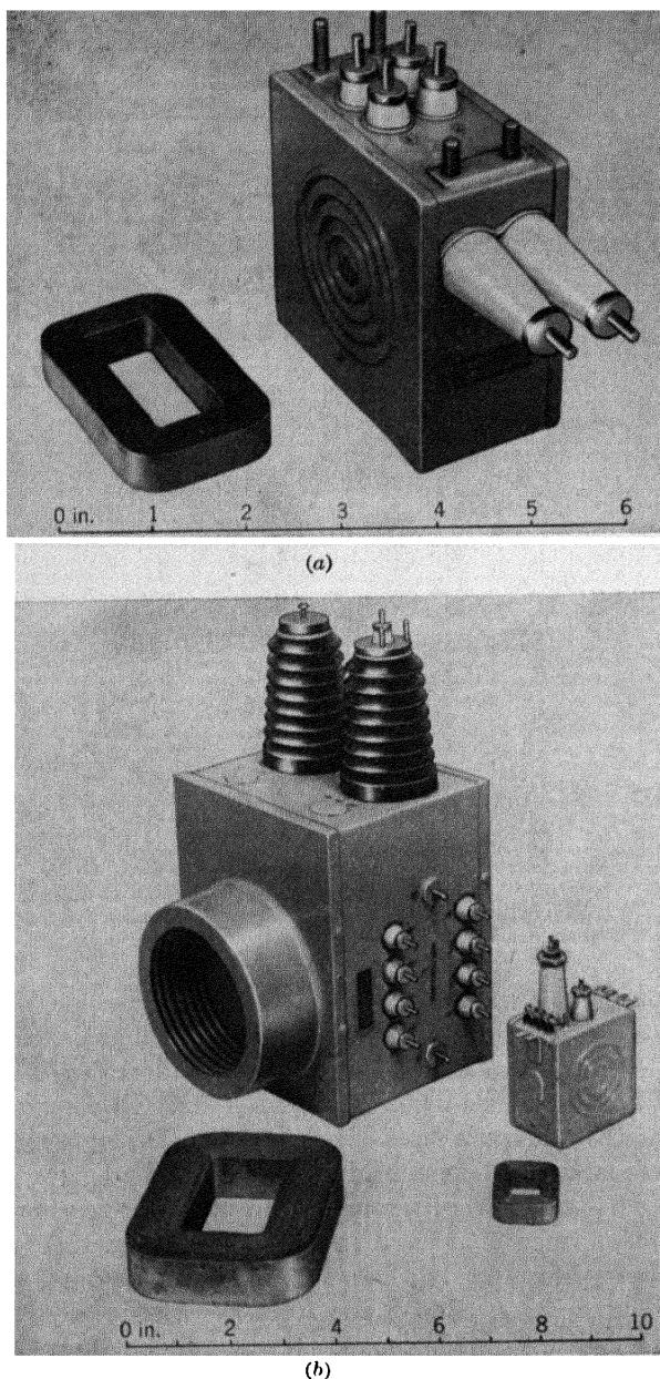
FIG. 13-12.—Three pulse transformers constructed with continuously wound permalloy cores (Western Electric Company). (a) Rectangular core of 1-mil 4-79 molybdenum permalloy and pulse transformer in which it is used. Pulse power: 100 kw. (b) 3-lb. rectangular core of 2-mil 45 permalloy and \frac{1}{4} -lb. core of 1-mil 4-79 molybdenum permalloy with the pulse transformers in which they are used.
