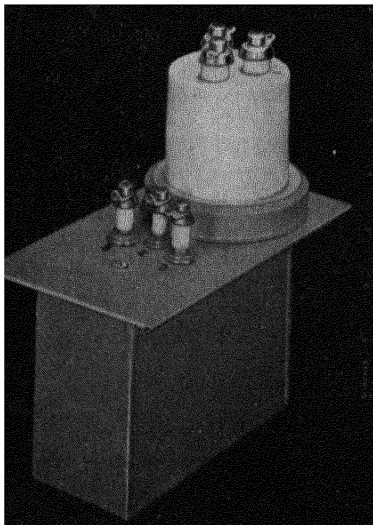
FIG. 15-36.—An airborne 250-kw 0.5- to 5.0-sec pulse transformer with a filament transformer enclosed in the high-voltage porcelain solder-seal bushing.
