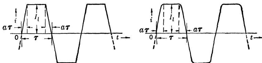
(a) Trapezoidal alternating-current wave. (b) Alternating-current wave with flat top and parabolic rise and fall.
