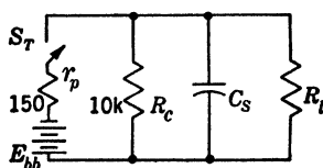
(m) Equivalent circuit for calculations.
