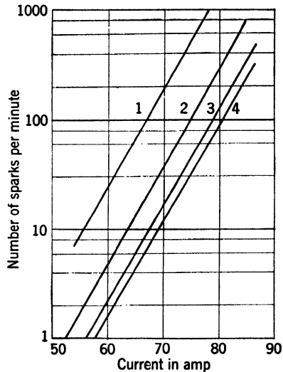
FIG. 10-24.—Sparkling rate vs. current for different networks of identical pulse duration and variable dv/dt .
