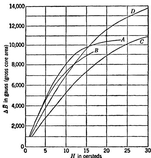
FIG. 15-9.—Loci of the tips of pulse B - H loops taken on butt-joint cores, with 1- \mu -sec pulses. Curve A is for Monimax 0.003 in., \frac{1}{2} in. by \frac{1}{2} in. leg section. Curve B is for silicon Nicaloi 0.003 in., \frac{1}{2} in. by \frac{1}{2} in. leg section. Curve C is for silicon Nicaloi 0.004 in., \frac{1}{2} in. by \frac{3}{8} in. leg section. Curve D is for Hipersil 0.002 in., \frac{1}{2} in. by \frac{3}{8} in. leg section.
