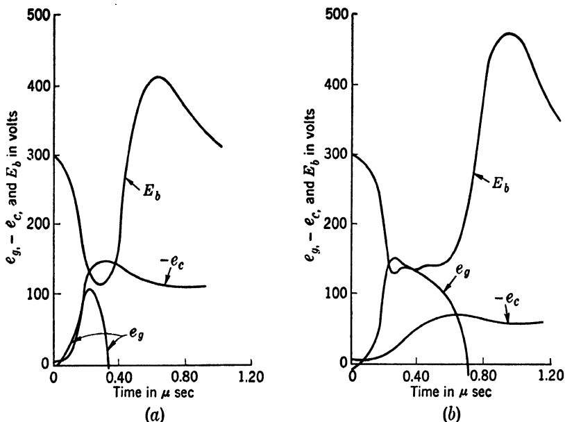
FIG. 14-25.—Typical pulse shapes obtained from a regenerative pulse generator employing a 6SN7 triode, a 132AW2 pulse transformer (see Table 13-2), for which R = 25,000 ohms, and E_{bb} = 300 volts. (a) C = 235 \mu\mu f . (b) C = 2700 \mu\mu f .
