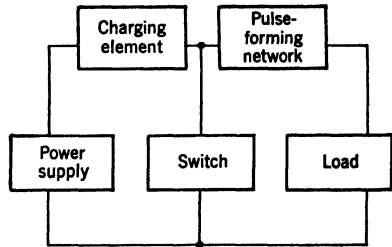
FIG. 9-1.—Block diagram of a line-type pulser.
