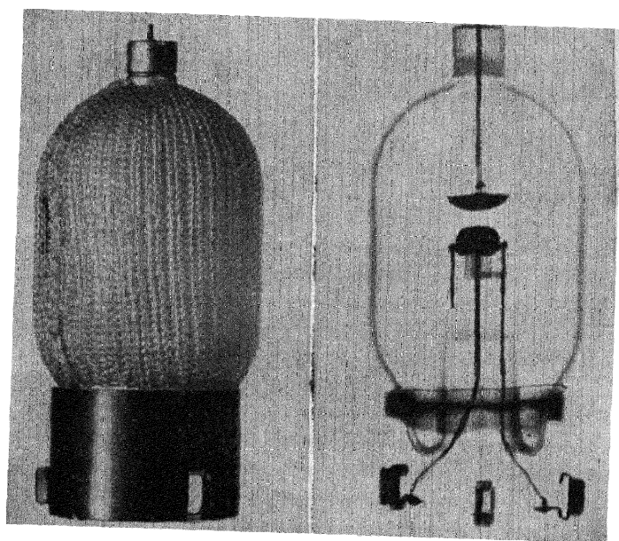
FIG. 8-33.—(a) A photograph and (b) an x-ray print of the CV125 three-electrode gap.
