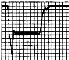
(e) Wirewound resistor No. 2. Resistance load current pulses.
