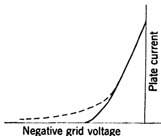
FIG. 3-2. a Plate-current—grid-voltage characteristic of a high-vacuum tube showing the effect of leakage current resulting from improper grid structure.
