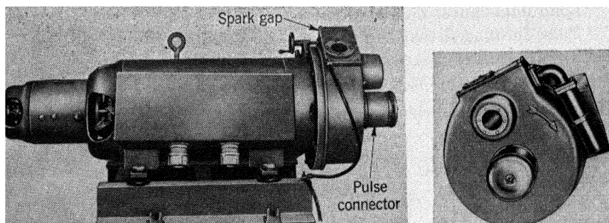
FIG. 11-36.—(a) Motor-generator and rotary-gap switch for the multiple-load pulser. (b) Rotary spark gap.
