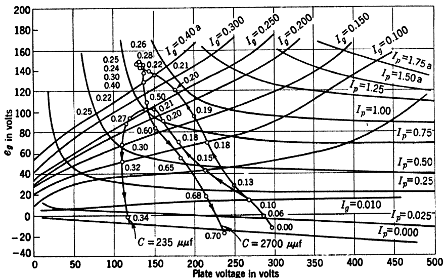
FIG. 14-26.—Operating curves for the two pulses shown in Fig. 14-25 with time intervals indicated in \mu\text{sec} .
