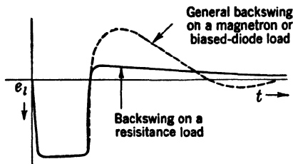
FIG. 14-9.—Typical backswings with resistance and biased-diode loads.
