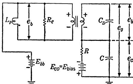
FIG. 14-24.—Equivalent circuit for the operation of a regenerative pulse generator during the tail of the pulse.
