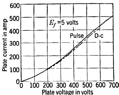
FIG. A-34.—Plate-current—plate-voltage characteristic of type GL-8020 diode.
