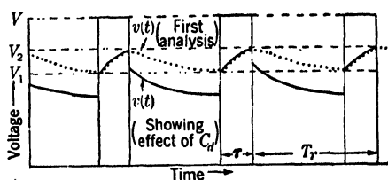
FIG. A-32.—Impressed voltage pulses and resulting voltage on the capacitance C of Fig. A-29 (distorted time scale).
