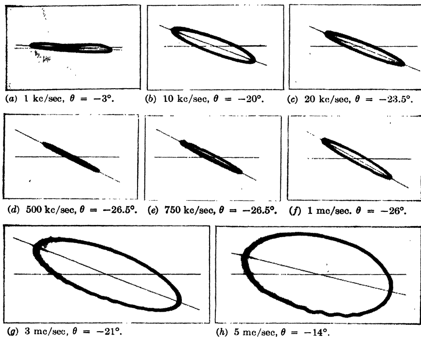
FIG. 14-35.—Photographs of oscilloscope presentation of the frequency-response characteristics of a pulse transformer with n = -1 and R_l = R_G = 1000 ohms.
