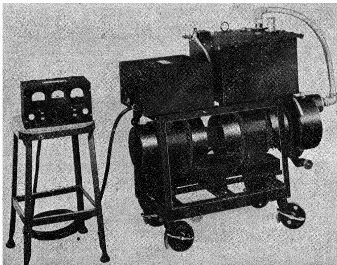
FIG. 11-2.—High-power line-type pulser of Fig. 11-1, side view.
