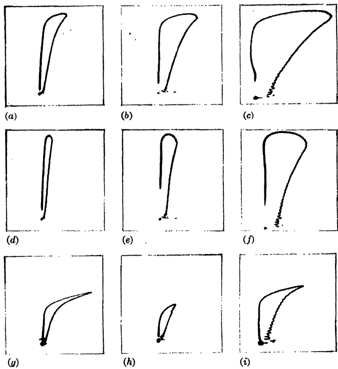
FIG. 15-10.—Photographs of oscilloscope traces of pulse B - H loops at various pulse durations. \bar{B} is vertical and H is horizontal.
