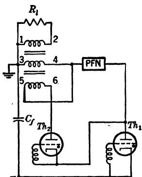
FIG. 11-40.—Circuit diagram for a double-switch single-network pulser.
