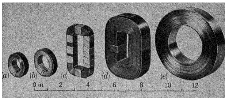
FIG. 15-7.—Various uncut Ni steel pulse-transformer cores. (a), (b), and (c) 0.001-in. Mo permalloy cores. (d) and (e) 0.002-in. 45-permalloy cores.
