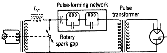
FIG. 11-1.—Schematic diagram of a high-power line-type pulser using a rotary-spark-gap switch and a-c resonant charging.
