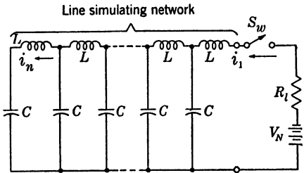
FIG. 6-4.—Two-terminal line-simulating network derived by Rayleigh's principle.
