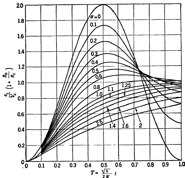
FIG. 14-3.—Plot of \frac{e_l}{V_g} \left( 1 + \frac{R_g}{R_l} \right) vs. T = \frac{\sqrt{b}}{2\pi} t .
