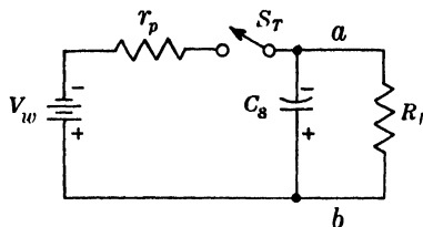
FIG. 2-7.—Equivalent output circuit for a hard-tube pulser with a resistance load. The charged storage condenser is replaced by a battery.
