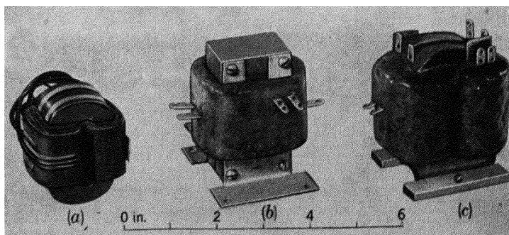
FIG. 13-10.—Three pulse transformers designed for operation at 120 kv, 0.5, 1.0, and 2.0 \mu sec. (a) Core-and-coil assembly of an oil-filled pulse transformer (232-BW2) on a 0.002-in. Hipsil core. (b) G. E. pulse transformer with Permafil insulation on a 0.003-in. Monemax core. (c) Westinghouse pulse transformer with Fosterite insulation on a 0.002-in. Hipsil core.
