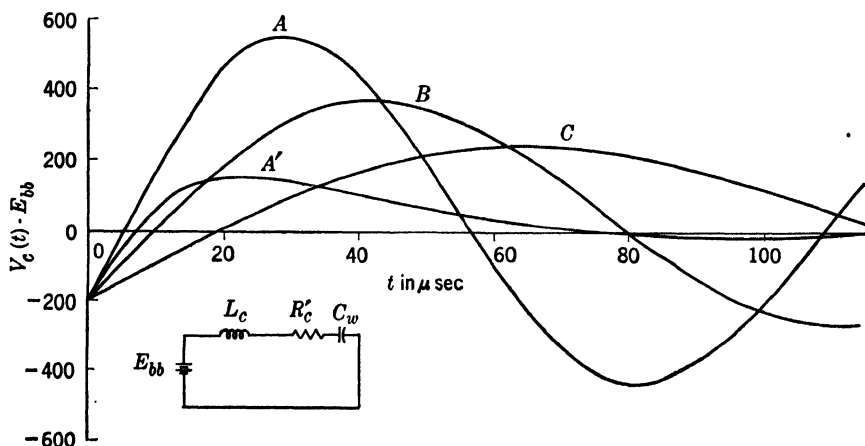
FIG. 2-40.—Storage-condenser voltage as a function of time during the recharging interval for an inductive element in series with the power supply; small values of R'_c/L_c . For curves A , B , and C the value of R'_c/L_c is 10 ohms per mh with L_c = 5 mh, 10 mh, and 20 mh respectively. For curve A' , L_c = 5 mh and R'_c = 500 ohms. E_{bb} = 10 kv and C_w = 0.05 \mu\text{f} for all curves.
