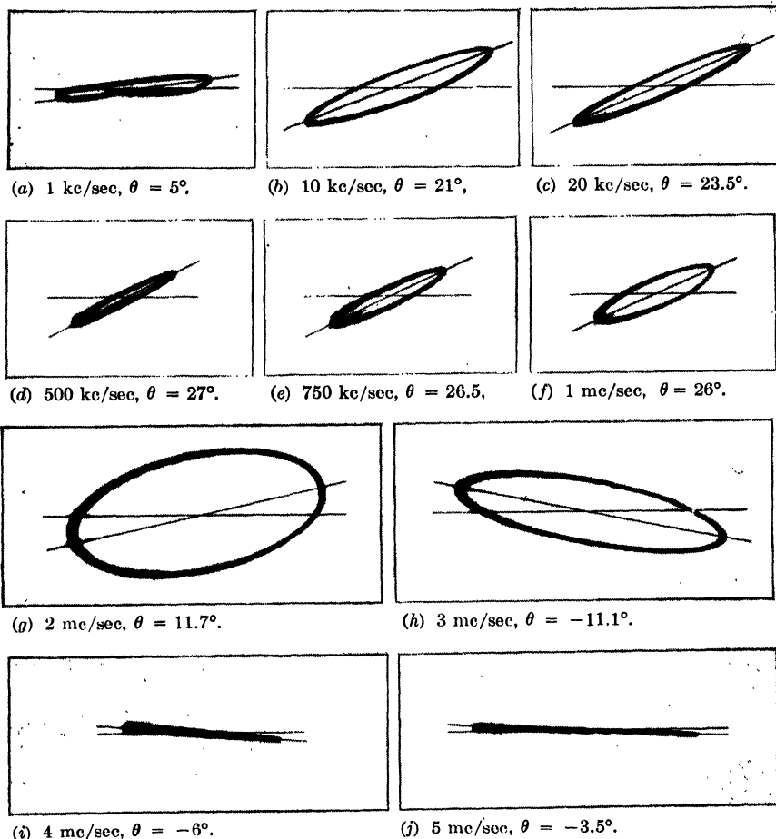
FIG. 14-36.—Photographs of oscilloscope presentation of the frequency-response characteristics of two pulse transformers ( n = \frac{1}{5} and n = 5 ) with resultant n = 1 .
