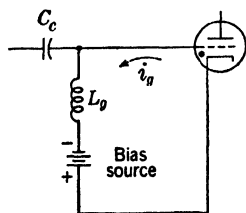
FIG. 8-55.—Thyatron grid circuit with bias.
