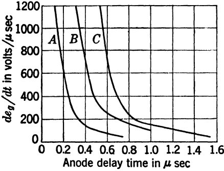
FIG. 8-53.—Effect of the rate of rise of trigger voltage on the anode delay time. Curve A is for the shortest delay, curve B is for the longest delay, and curve C is an average based on A and B and statistical data. (4C35, V_N = 8 kv, trigger amplitude = 150 v.)
