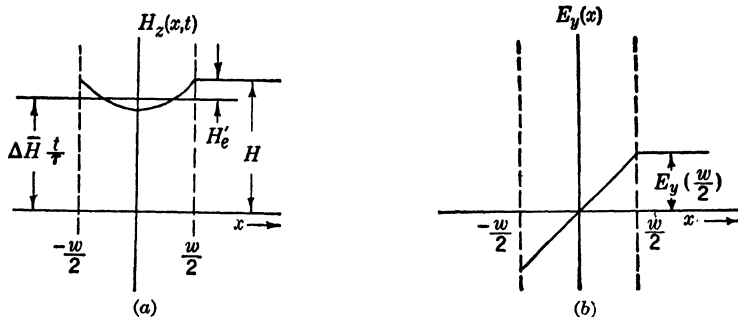
FIG. 15-25.—Steady-state distribution throughout the core of (a) H_z(x,t) , where H_e' = 10^{-9}\mu\pi w^2\Delta\bar{H} oersteds, and (b) E_y(x) , where E_y\left(\frac{w}{2}\right) = \frac{10^{-8}\mu\Delta\bar{H}w}{2\tau} volts.
