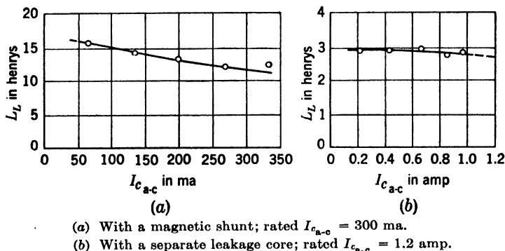
Fig. 9-22.—Leakage inductance vs. secondary a-c current for typical a-c charging transformers.
