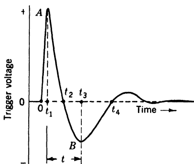
FIG. 8-13.—Bidirectional trigger pulse for satisfactory operation of a two-gap switch.
