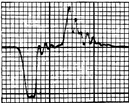
(e) Time derivative of (c) observed with short leads and mismatched cable.
