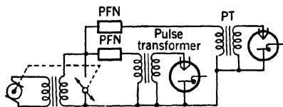
FIG. 11-33.—Schematic diagram of a multiple-load pulser.
