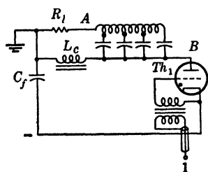
FIG. 11-21.—The revised Anger circuit.
