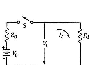
FIG. 7-6.—Simplified equivalent circuit for a line-type pulser with a resistance load.
