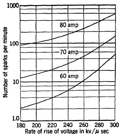
FIG. 10-25.—Sparking rate vs. rate of rise of voltage for several pulse currents at \tau = 1.89\mu\text{sec} .
