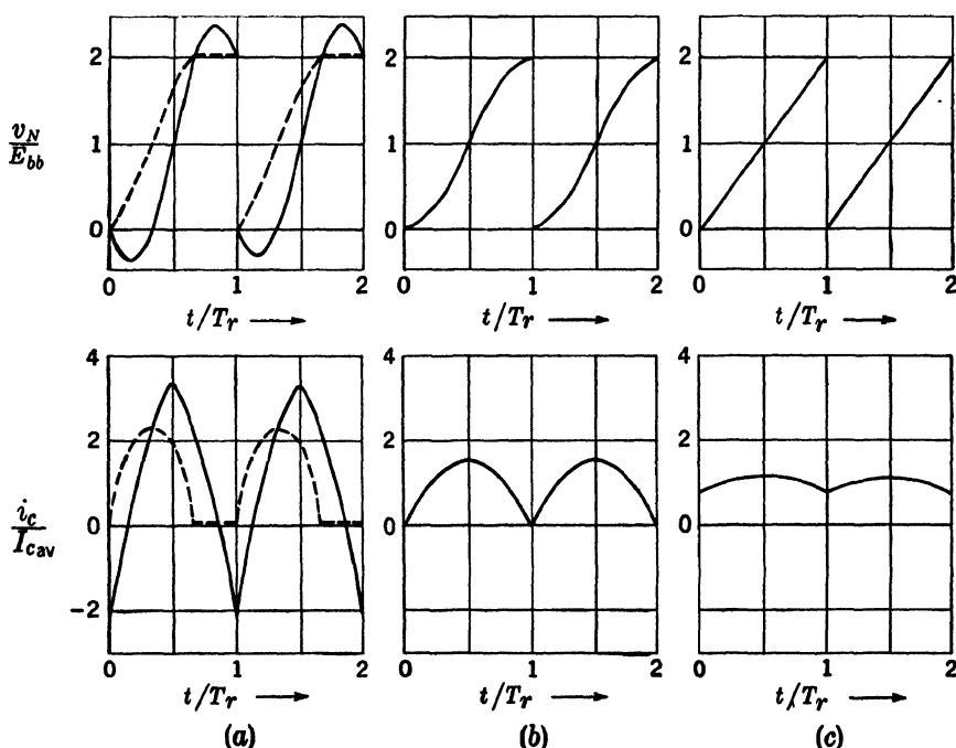
FIG. 9-3.—Charging-voltage and current wave shapes. v_N(0) = 0 , R_c = 0 , (a) L_c = \frac{1}{3}L_r , (b) L_c = L_r , (c) L_c = 4L_r . The dotted lines correspond to the use of a charging diode.
