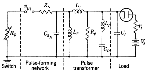
FIG. 7-13.—Equivalent discharging circuit for a line-type pulser.
