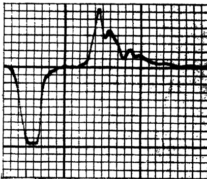
(d) Time derivative of (c) observed with short leads and matched cable.
