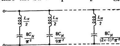
FIG. 6-8.—Two-terminal network to simulate an open-ended transmission line, obtained by rational-fraction expansion of the admittance function.
