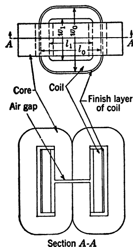
FIG. 9-11.—Sketch of d-c resonant-charging reactor.
