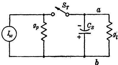
FIG. 2-8.—Equivalent circuit for calculating the leading edge and top of the pulse for a hard-tube pulser with a resistance load, I_w = g_p V_w , g_p = 1/r_p and g_l = 1/R_l .
