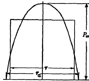
FIG. B-4.—Sine-wave power pulse.
