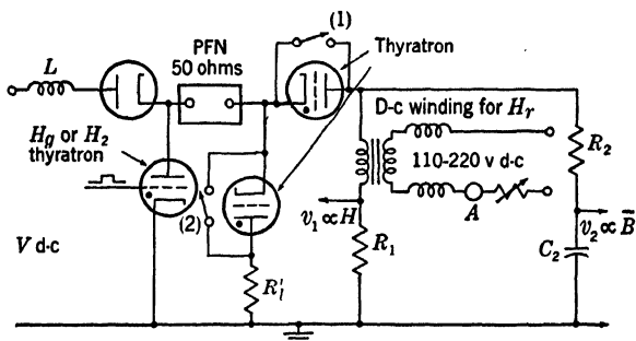
FIG. 15-28.—Circuit for obtaining pulse B - H loops with a line-type pulser.
