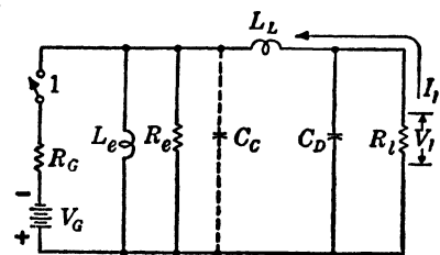
FIG. 13·1.—Equivalent circuit used in the consideration of the optimum relationships among R_L , C_D , L_L , L_e , and R_e for a specified load impedance and pulse duration.
