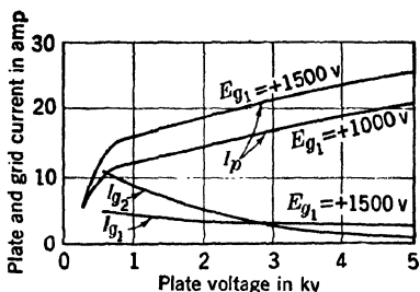
(a) 6D21 (Raytheon), E_{g2} = 2\text{kv} .
