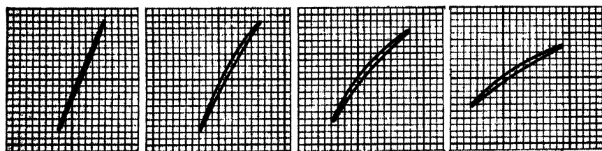
(i) I_{c_{av}} = 0.150 amp, L_c = 27.1 henrys. (j) I_{c_{av}} = 0.200 amp, L_c = 20.9 henrys. (k) I_{c_{av}} = 0.250 amp, L_c = 10.6 henrys. (l) I_{c_{av}} = 0.300 amp, L_c = 7.1 henrys.
