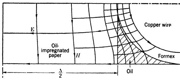
FIG. 15-39. —Flux plot showing lines of E and H for a typical pulse-transformer winding. No. 25 quadruple formex wire, dia = 0.0219 in., bare Cu dia = 0.0179 in. Spacing between windings \Delta = 0.040 in.
