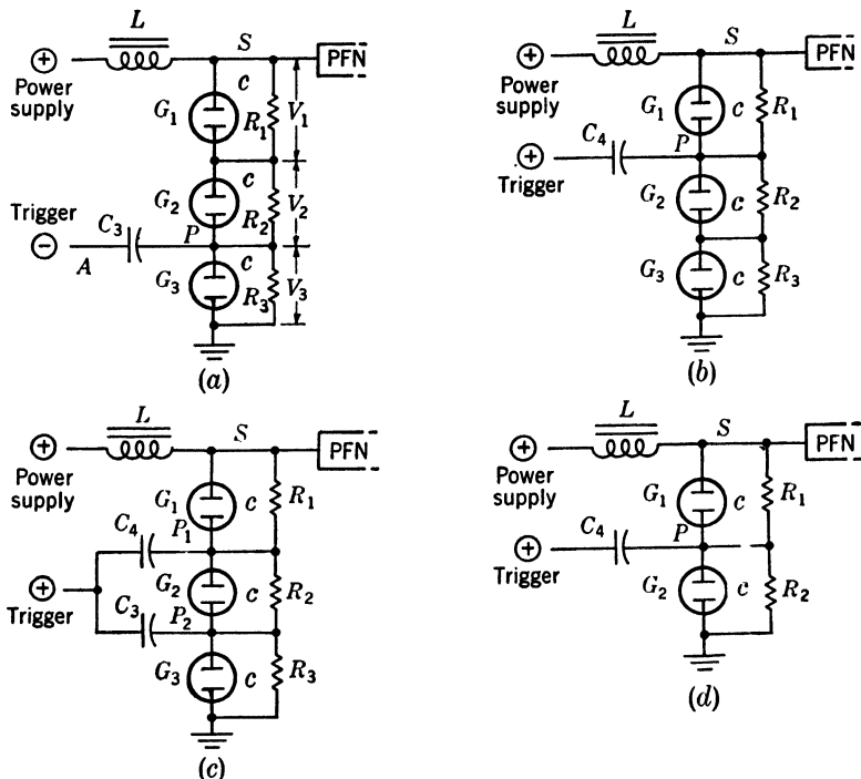
FIG. 8-9.—Four commonly used series-gap circuits.
