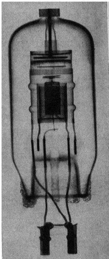
FIG. 8-38.—X-ray photograph of a hydrogen thyatron.
