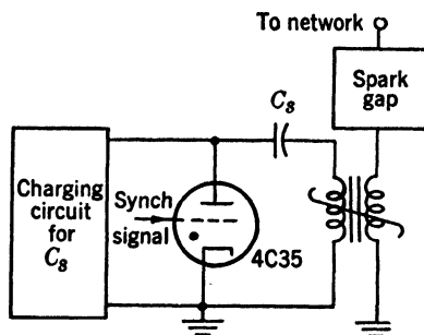
FIG. 8-20.—Trigger circuit using a saturable-core transformer.
