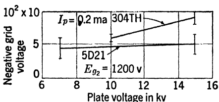
(b) The 304TH triode and the 5D21 tetrode.
