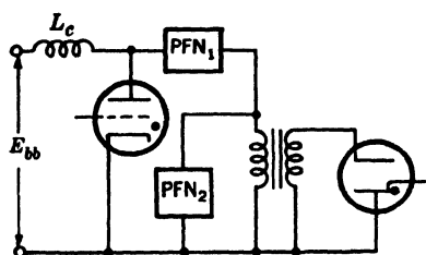
FIG. 11-43.—Circuit diagram for single-switch multiple-network pulser.
