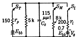
(g) Equivalent circuit for calculations.
