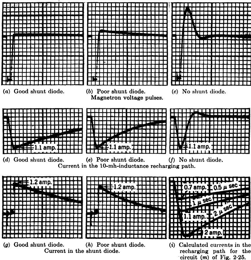
Fig. 2-26.—Oscilloscope traces and calculated recharging-path currents for a hard-tube pulser with a magnetron load and a 10-mh inductance as the recharging path. (a) and (d) are the slow-sweep-speed presentations corresponding to the 1- \mu sec pulses of Fig. 2-25. Horizontal scale = 1 \mu sec/div.
