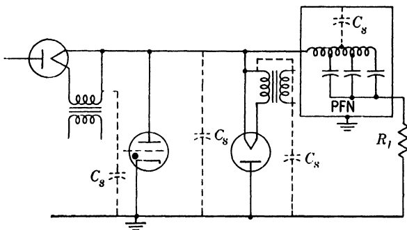
FIG. 8-49.—Typical pulser circuit showing distributed capacitance.
