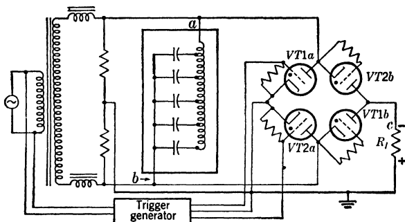
FIG. 11-32.—Schematic diagram of the thyatron-bridge circuit.
