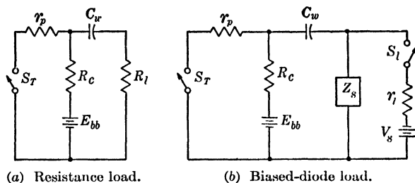
FIG. 2-30.—Hard-tube pulser circuits with a resistance as the isolating element in series with the power supply.
