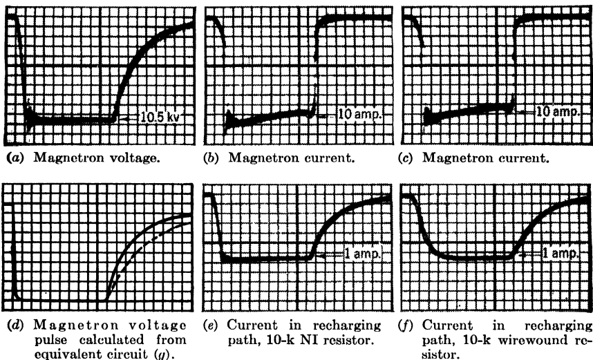
FIG. 2-19.—Oscilloscope traces and calculated voltage pulse for a hard-tube pulser with a magnetron load, a resistance recharging path and C_s = 115 \mu\text{mf} . The dotted line on the calculated pulse (d) is the trailing edge obtained with the magnetron assumed to be infinite resistance after S_l opens. The solid line is the trailing edge assuming an effective resistance of 8000 ohms for the magnetron, that is, switch S_M closes when S_l opens. Sweep speed: 10 div. = 1 \mu\text{sec} .
