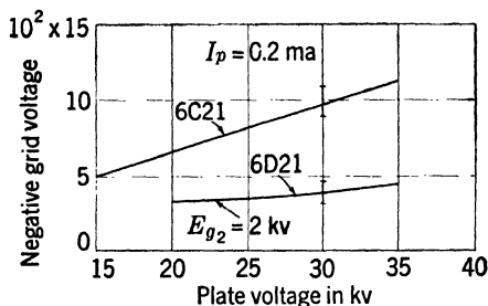
(a) The 6C21 triode and the 6D21 tetrode.
