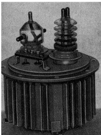
FIG. 15-38.—Illustration of the use of cast-glass bushings on a 1.5-Mw 2.0-sec pulse transformer. The seal is accomplished by the adhesion of molten borosilicate glass to nickel iron.
