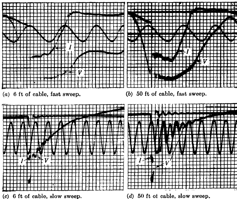
FIG. 7-29.—Oscillograms showing the effect of cable length on the pulse shapes for a 0.2\text{-}\mu\text{sec} current pulse.
