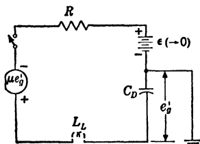
FIG. 14.17.—Circuit of Fig. 14.16 further simplified by setting e'_g = |e_g - E_{co}| .
