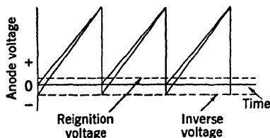
FIG. 8-47.—Anode-voltage waveform with and without inverse voltage.
