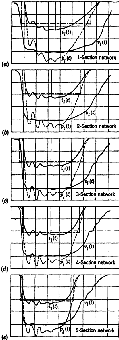
FIG. B-5.—Voltage, current, and computed power pulses in an HK7 magnetron, (a) with a 1-section pulse-forming network, (b) with a 2-section pulse-forming network, (c) with a 3-section pulse-forming network, (d) with a 4-section pulse-forming network, (e) with a 5-section pulse-forming network.
