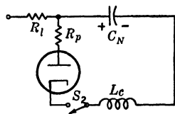
FIG. 11-20. Schematic diagram of the potential-reversing circuit.
