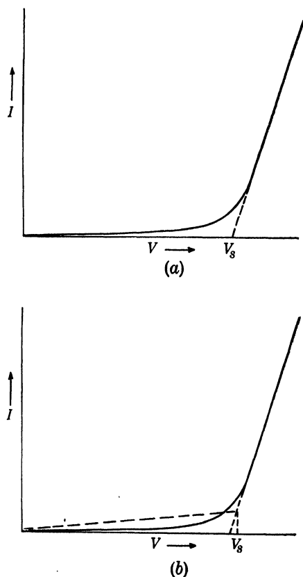
FIG. 2-11.—Current voltage characteristic of a magnetron.
