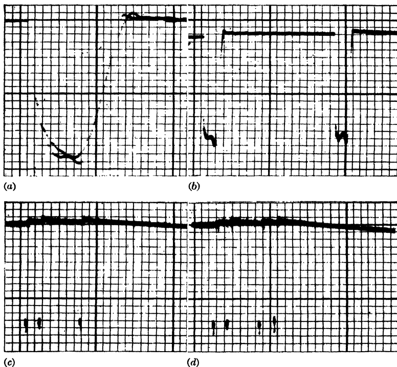
FIG. 11.42.—Pulse shapes obtained on a resistance load with multiple-switch single-network circuit. (a) Circuit arranged for single-pip operation with uniform interpulse intervals. (b) Circuit arranged for two-pip operation, (c) for three-pip operation, and (d) for four-pip operation.
