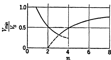
FIG. 8-12.—Ratio of V_{\min} to V_s as a function of n .
