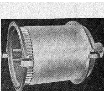
FIG. 11-9.—Outside view of the completed can showing mounting rings and shock mounts. (Courtesy of the Westinghouse Research Laboratories.)
