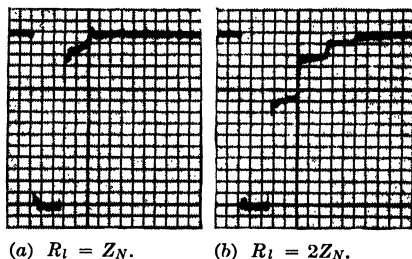
FIG. 6-11.—Voltage pulse shapes obtained with network of Fig. 6-8 as seen with a slow sweep speed.
