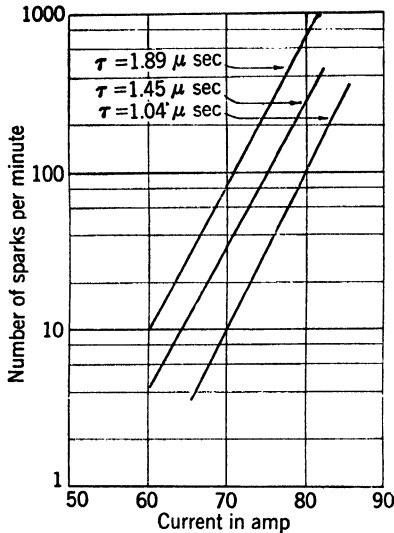
FIG. 10-23.—Sparkling rate vs. current for variable pulse durations. In all cases, dv/dt = 200 kv/ \mu sec at 60 amp.
