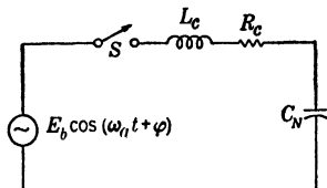
FIG. 9-15.—Schematic circuit for a-c inductance charging.
