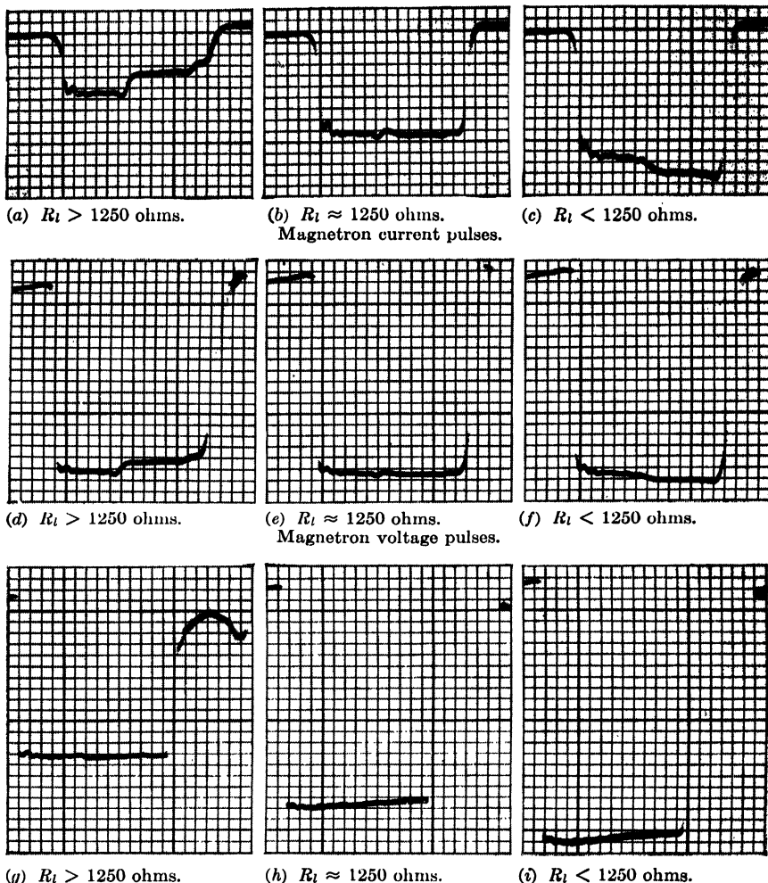
FIG. 2-46.—Oscilloscope traces for 2- \mu sec pulses of magnetron current, magnetron voltage, and pulser output voltage for a hard-tube pulser with the 232AW and the 232BW pulse transformers and 175 ft of 50-ohm pulse cable. The 50-ohm cable impedance is transformed to 1250 ohms at the output of the pulser and the input to the magnetron because the turns ratio for each transformer is 1 to 5. The transit time for the transformers and cable is 0.42 \mu sec.
