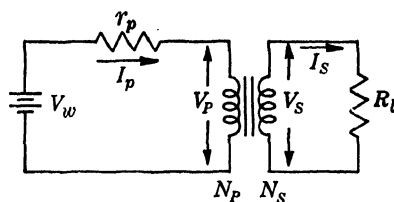
FIG. 2-41.—Equivalent circuit for a hard-tube pulser with pulse-transformer coupling to the load.
