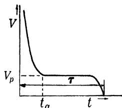
FIG. 7-10.—Typical switch drop as function of time.
