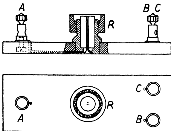
FIG. 40.—Electrolytic slide.
