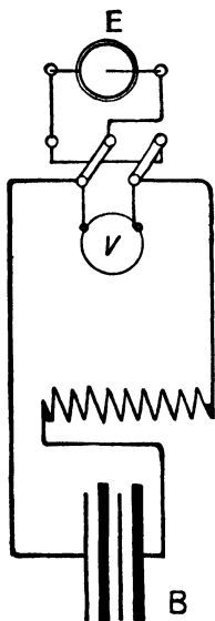
FIG. 83.—Wiring diagram for electrolytic copper determination.
