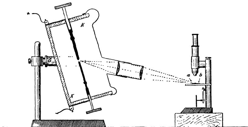
FIG. 65.—Testing for fluorescence and fine turbidity.
