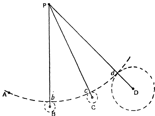
Fig. 23.—Sound-ranging Diagram
