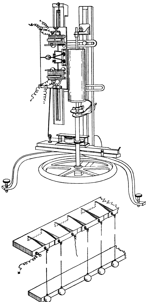
Fig. 1.—The Bashforth Chronograph and Screen. Reproduced by courtesy from "Description of a Chronograph", by F. Bashforth, B.D., Proceedings of the Royal Artillery Institution , 5, 1867.
