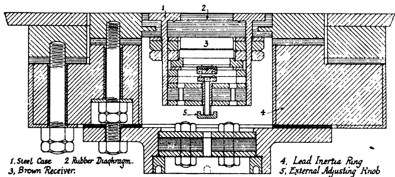
Fig. 17.—Air-drive Magnetophone
