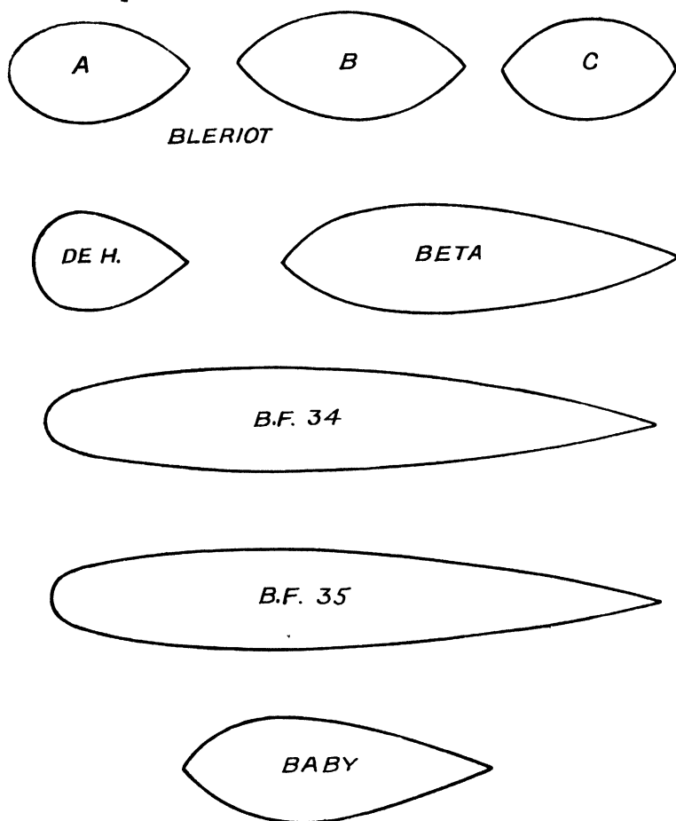
Fig. 6.—Strut Sections.
