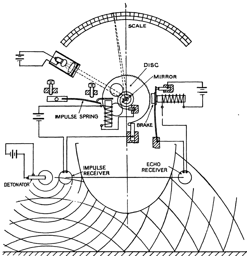
Fig. 29.—Behm's Acoustic Depth-sounding Method
