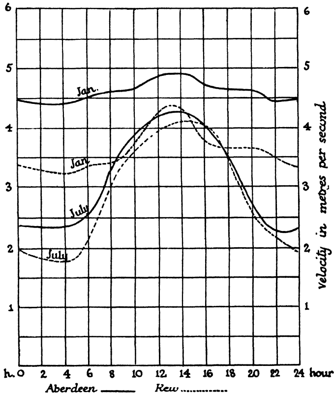
Fig. 5.—Diurnal Variation in Wind Velocity for January and July, for the period 1881-1910
