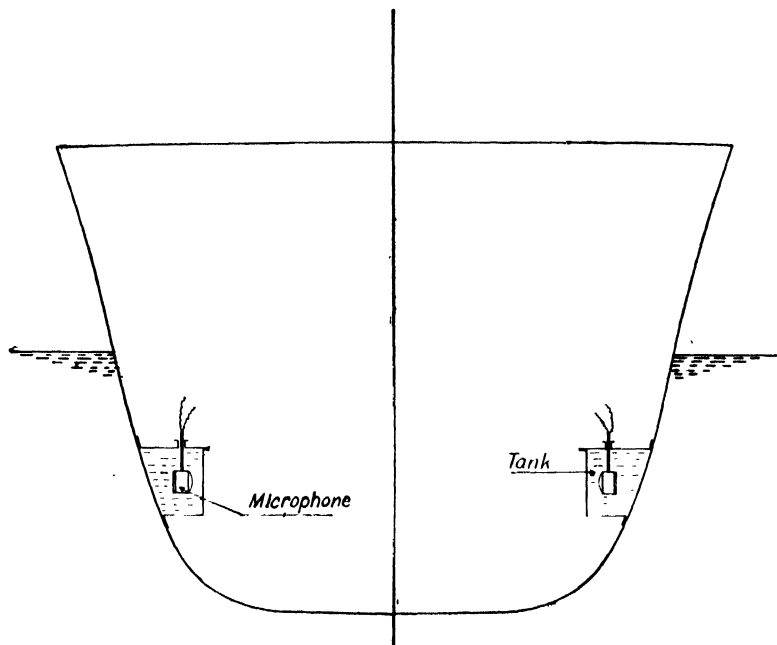
Fig. 21.—Reception by Hydrophone in Tanks
