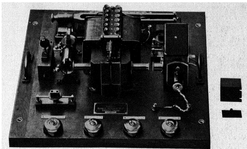
FIG. 25--EINTHOVEN CAMERA FOR SOUND RANGING
