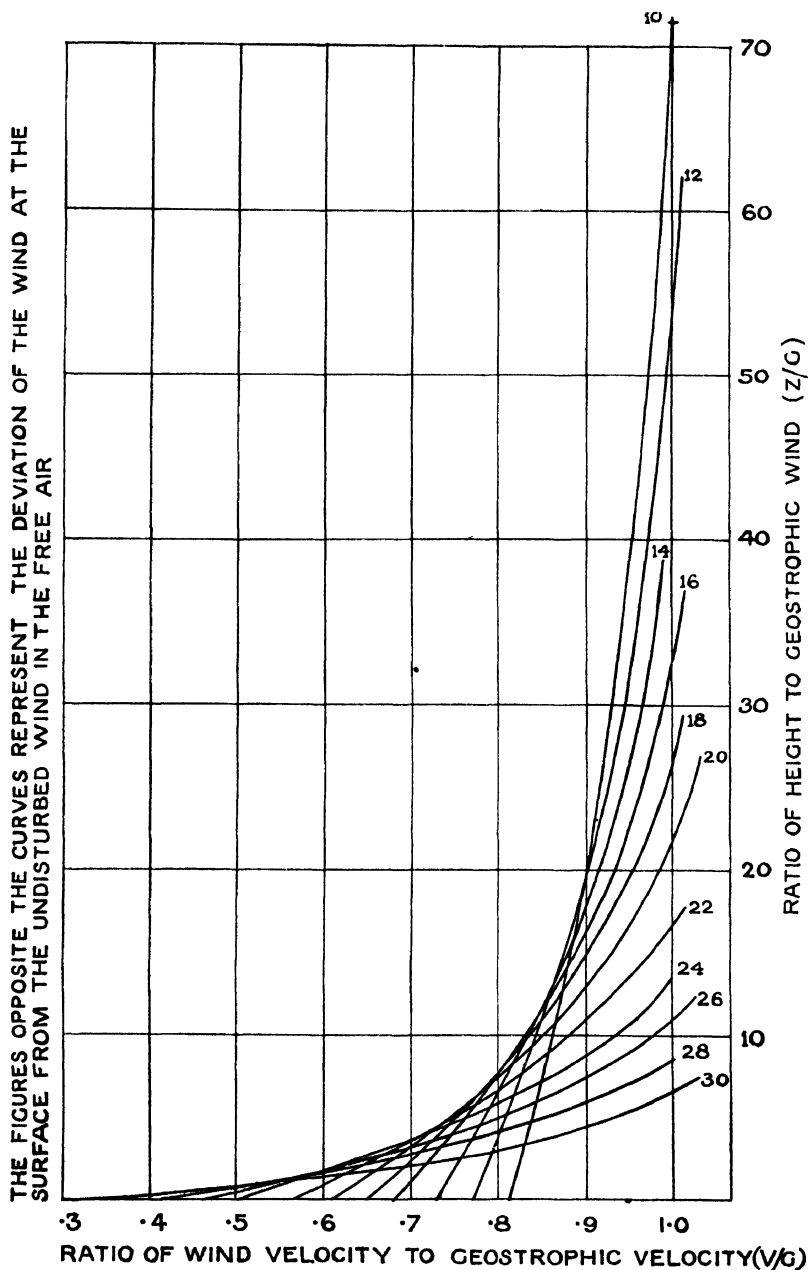
Fig. 8.—Curves showing Variation of Wind Velocity with Height, according to the Theory of the Diffusion of Eddy-motion.
