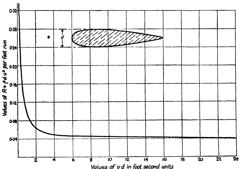
Fig. 5.—Resistance of Strut Sections.
