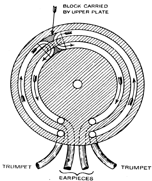
FIG. 4(a).—AMERICAN COMPENSATOR FOR DIRECTIONAL LISTENING
