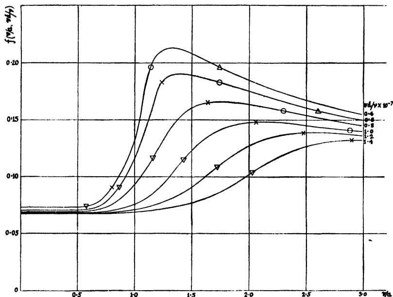
Fig. 4.—Curves of f(v/a, vd/v) for constant values of vd/v
