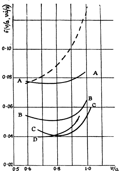
Fig. 9.—The Drag Coefficient deduced from High-speed Air-stream Experiments
