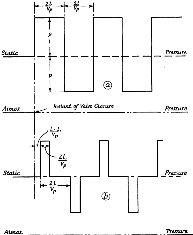
Fig. 1.—Ideal Case of Water-hammer in Pipe Line
