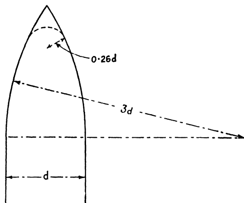
Fig. 6.—Shape of Head
