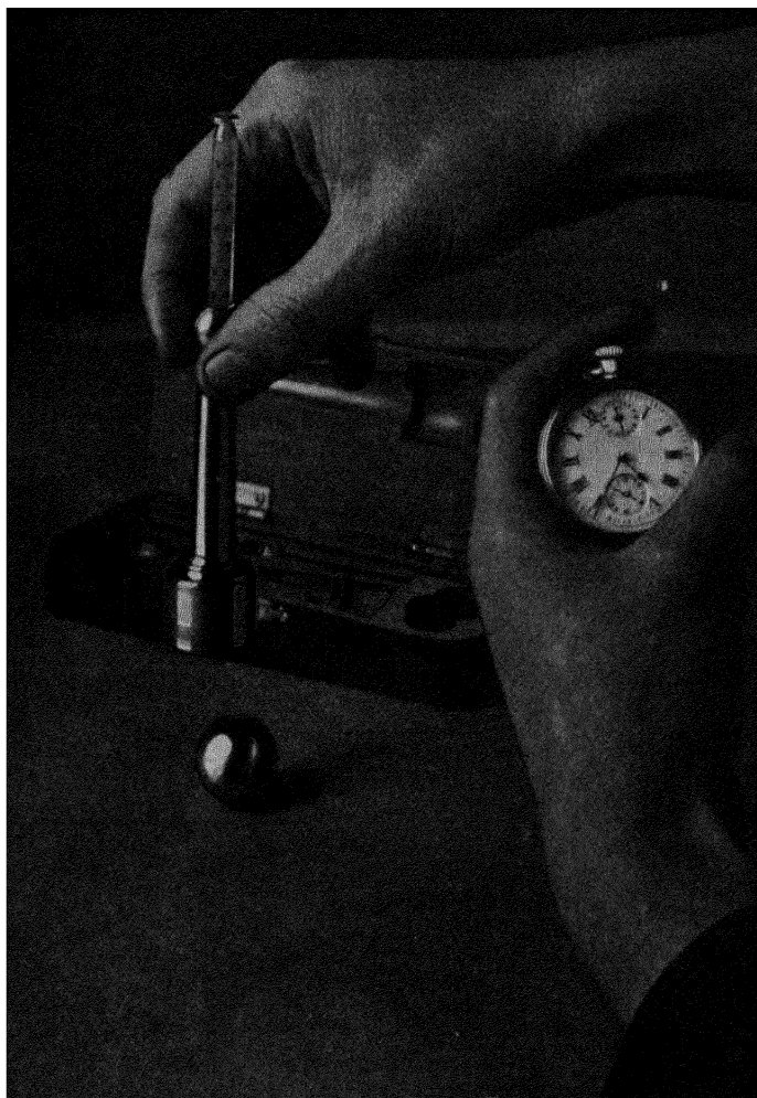
Fig. 13.—Cup-and-ball Viscometer
