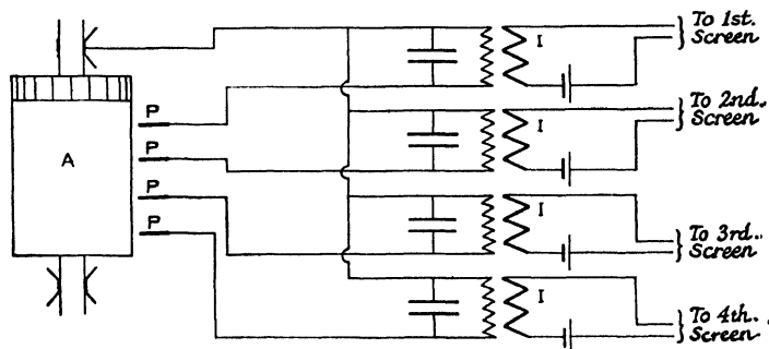
Fig. 2.—The Spark Chronograph used in Krupp's 1912 Experiments
