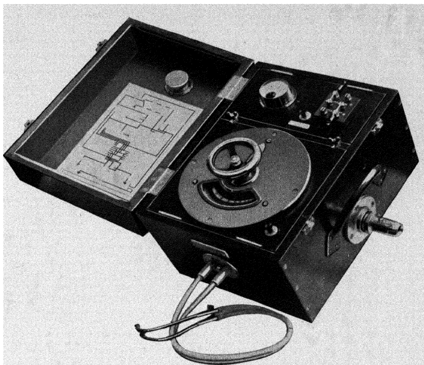
FIG. 4(a).—AMERICAN COMPENSATOR FOR DIRECTIONAL LISTENING
