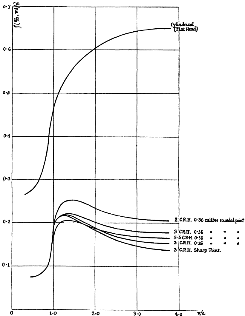
Fig. 7.—The Drag Coefficients for 10-cm. Projectile with Various Shapes of Head, plotted as a Function of Velocity
