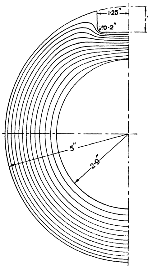
Fig. 5.—Lines of Shearing Stress in the Torsion of a Hollow Shaft with Keyway
