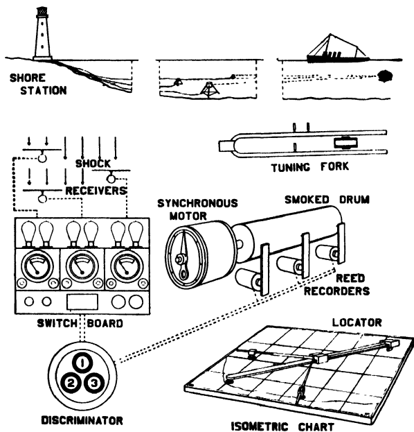
Fig. 27.—Sound-ranging Apparatus
