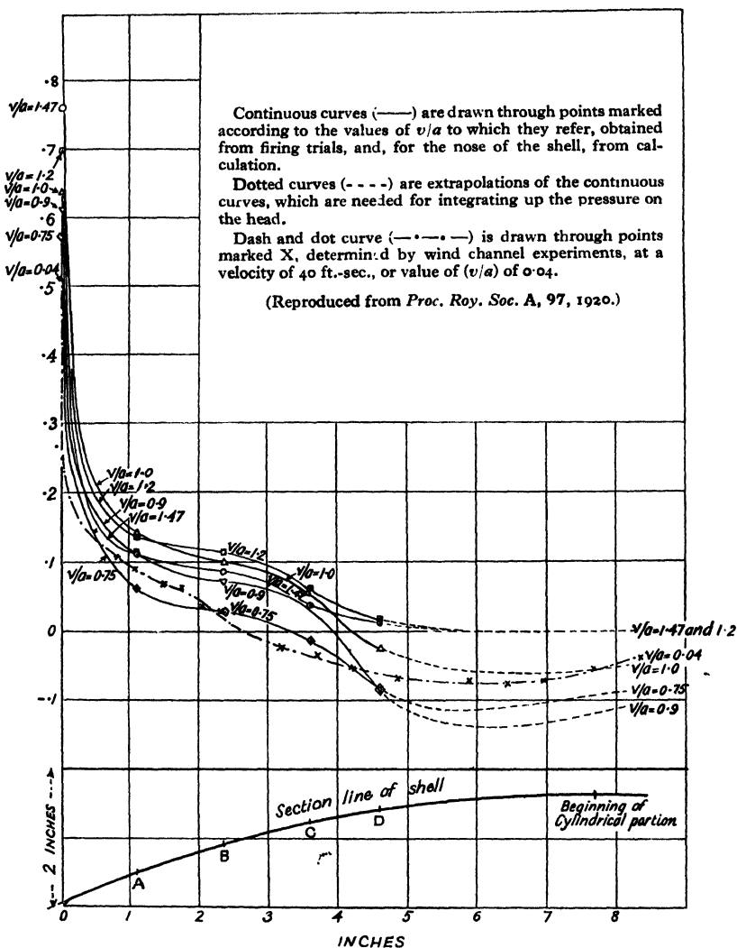
Fig. 10.—Distribution of Pressure on the 6-cal.-rad. Head of a 3.3-in. Shell
