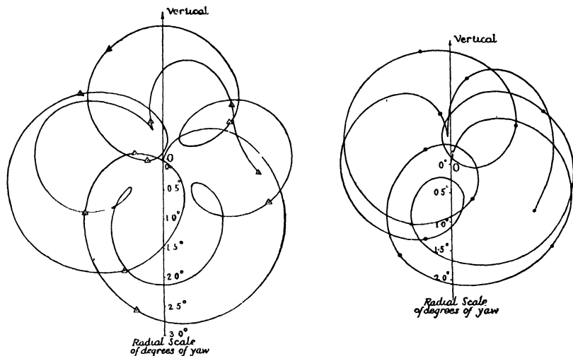
Fig. 16.—Examples of Path of Nose of Shell relative to the Centre of Gravity
