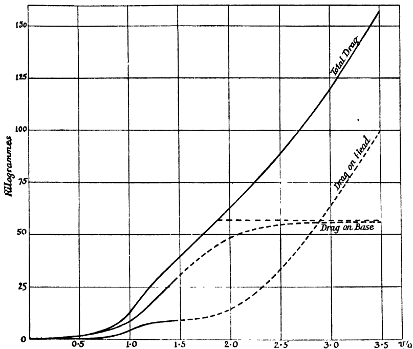
Fig. 11.—Drag in Kilogrammes Weight on a 3.3-in. 6 C.R.H. Projectile
