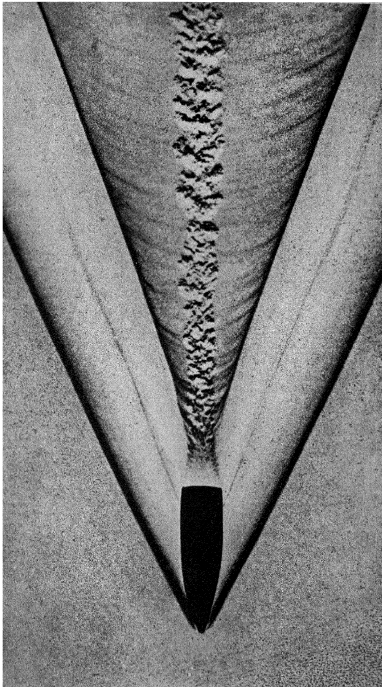
FIG. 3. — PHOTOGRAPH OF AN 8-MM. BULLET MOVING WITH VELOCITY OF ABOUT 880 M./S.
