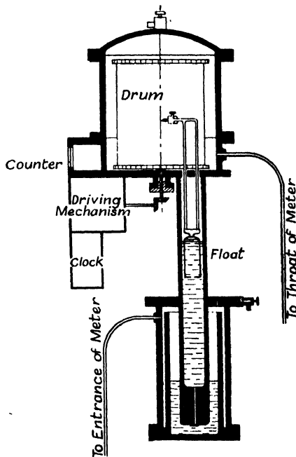
Fig. 12.—Recording Mechanism for Venturi Meter.
