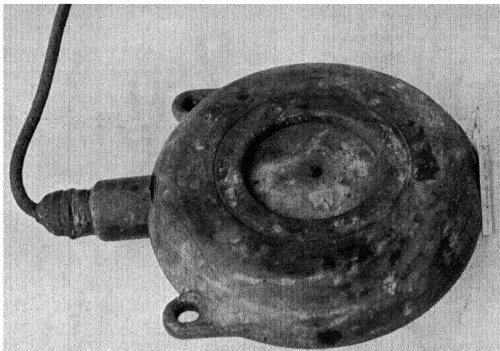
FIG. 19.—DOUBLE-DIAPHRAGM BI-DIRECTIONAL HYDROPHONE
