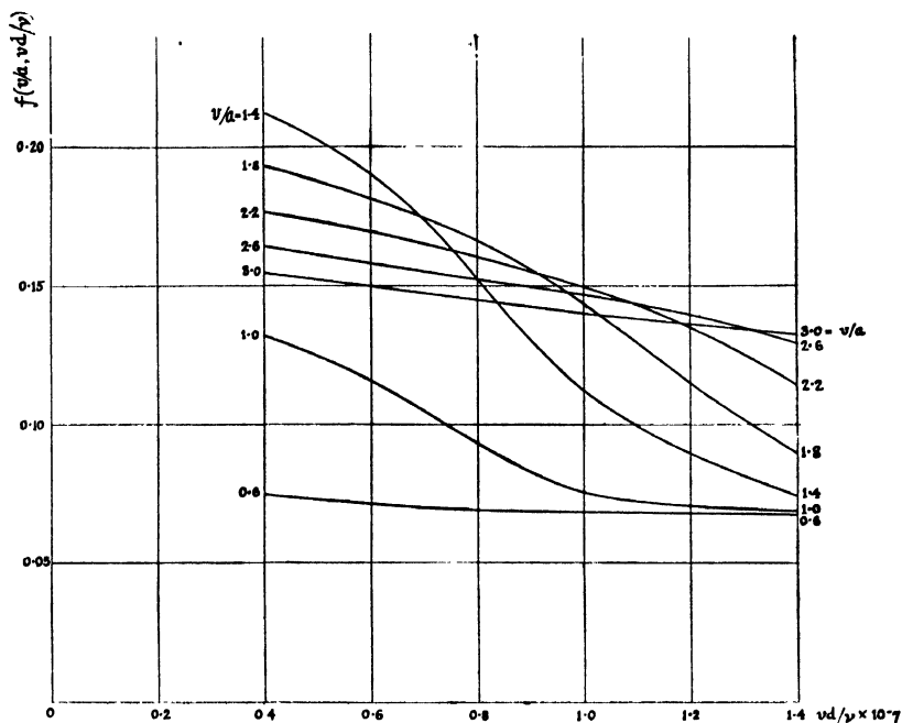
Fig. 5.—Curves of f(v/a, vd/v) for constant values of v/a
