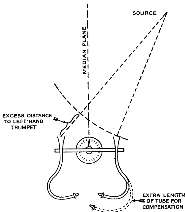
Fig. 2.—Binaural Listening with Trumpets
