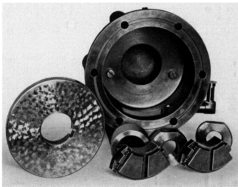
FIG. 26.—THRUST SHOES
