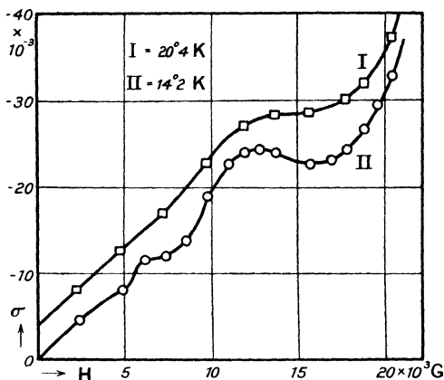
FIG. 29.—The curve for 20.4^\circ K. has been displaced -4 \times 10^{-3} along the \sigma axis, to avoid confusion with the other curve.
