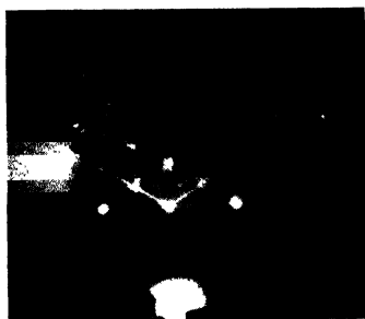
3. Reflection pattern from a cleavage face of zinc blende ( J. R. Tillman ).
