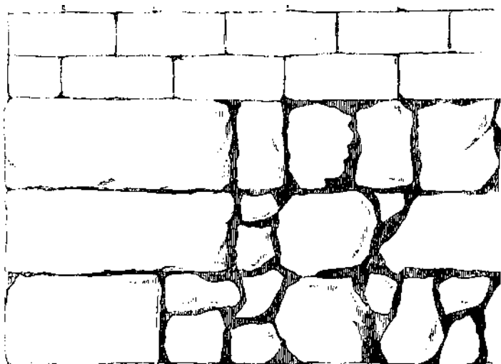
Masonry of town-wall (Khorsabad).
