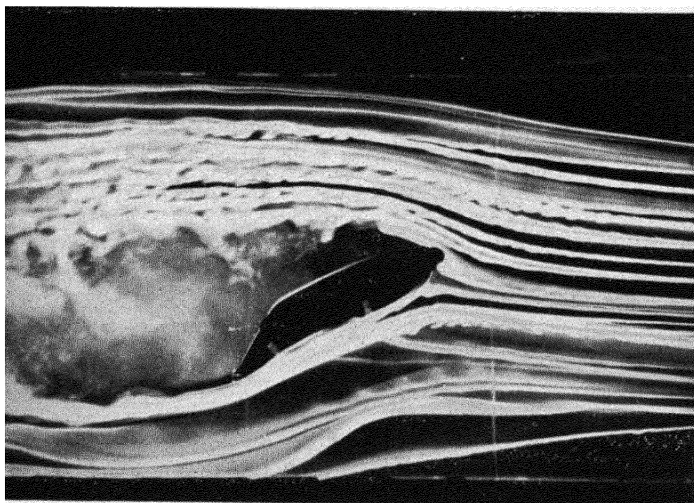
FIG. 123. Flow separation over airfoil with flap. (N.A.C.A.)
