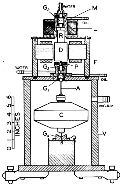
FIG. 115. Section of magnetically supported, electrically driven, vacuum-type centrifuge as described on page 258.
