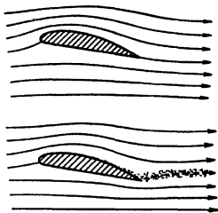
FIG. 117. Diagrams showing streamline pattern of flow of a frictionless fluid (above); and flow with friction (below).
