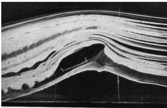
FIG. 123. Flow separation over airfoil with flap. (N.A.C.A.)
