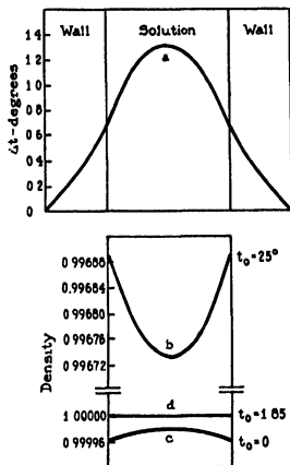
FIG. 91. Temperature and density relations across a tube through which current is passing.
