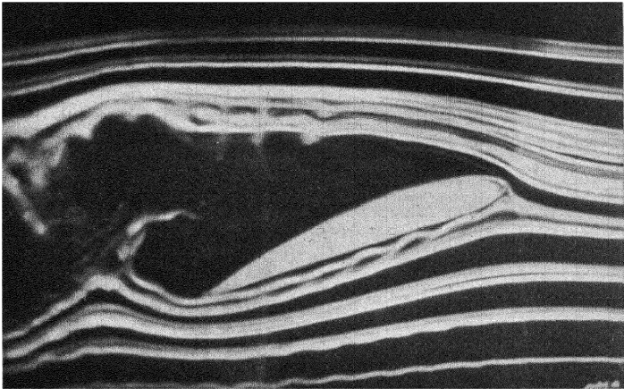
FIG. 122. Flow separation over top of airfoil. (N.A.C.A.)
