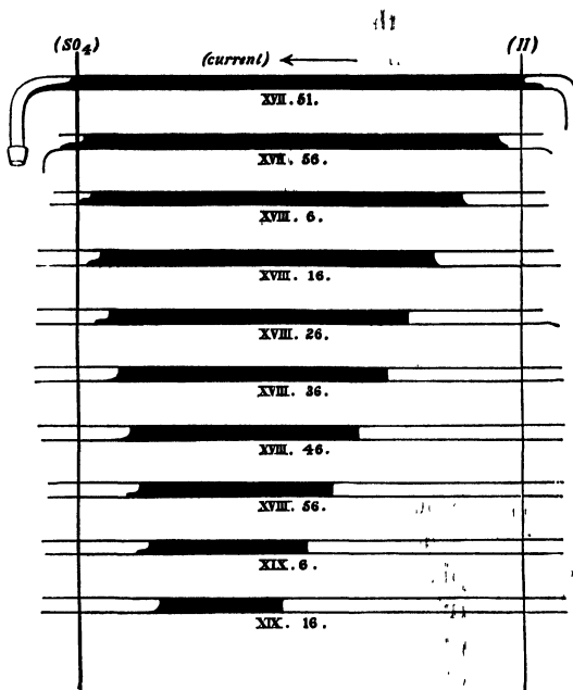
FIG. 77. Showing the motion of boundaries in Lodge's moving-boundary experiments.
