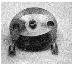
FIG. 111. Rotor used in equilibrium and rate of sedimentation methods for determining particle or molecular weight and size. Right foreground, cell with transparent crystal quartz windows. Left foreground, dummy cell necessary for balancing.
