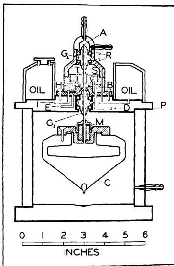
FIG. 103. Section of air-driven, vacuum-type centrifuge as described on page 241.
