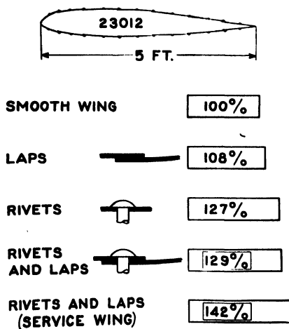
FIG. 127. Effects of rivets and laps at two hundred miles per hour. (N.A.C.A.)
