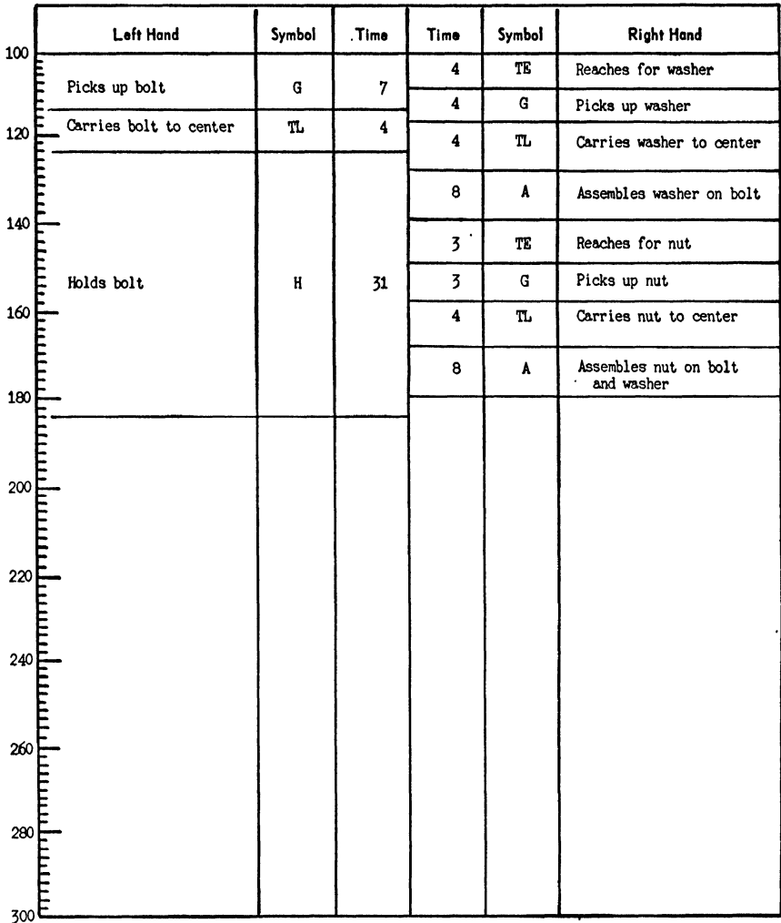
Figure 17-3. Simo Chart.
