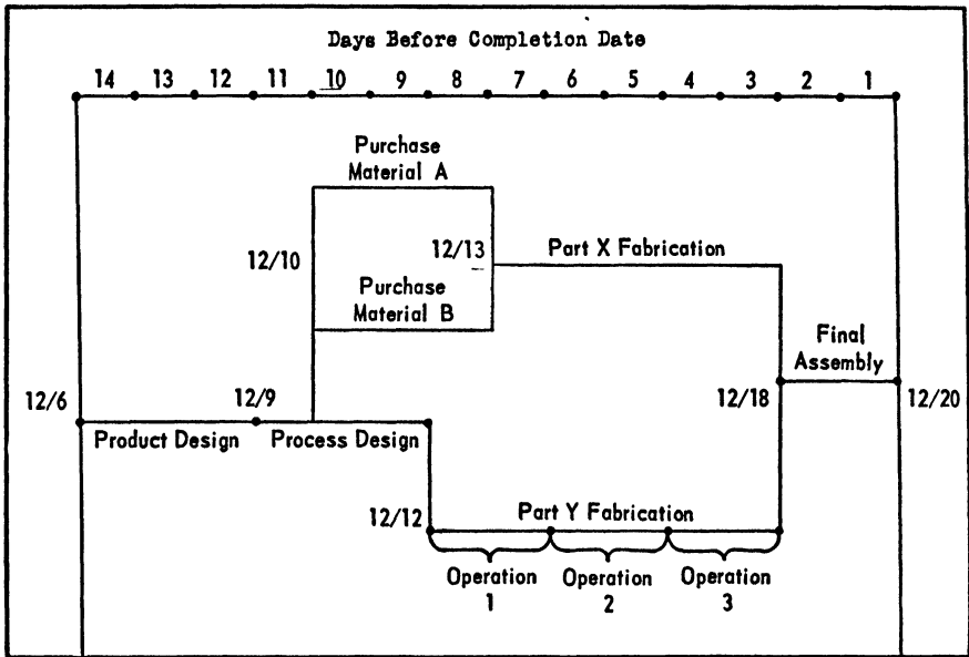
Figure 8-3. Schedule Computation.
