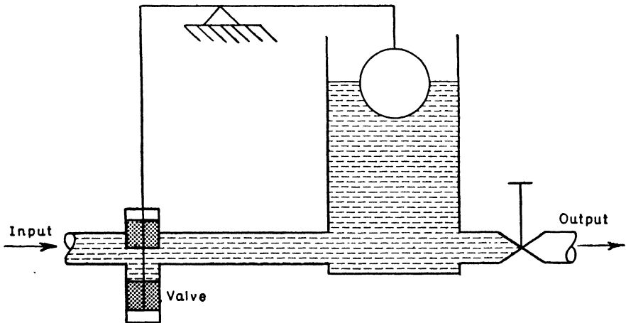
Figure 16-2. Closed-loop Control.
