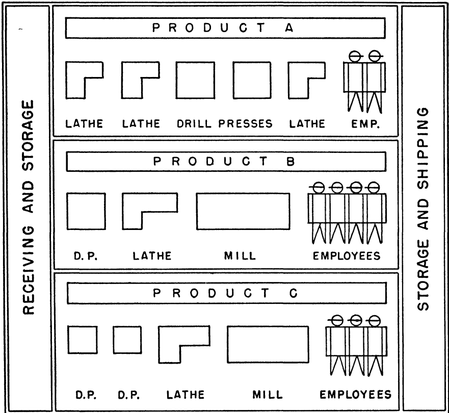
Figure 15-3. Layout by Product.
