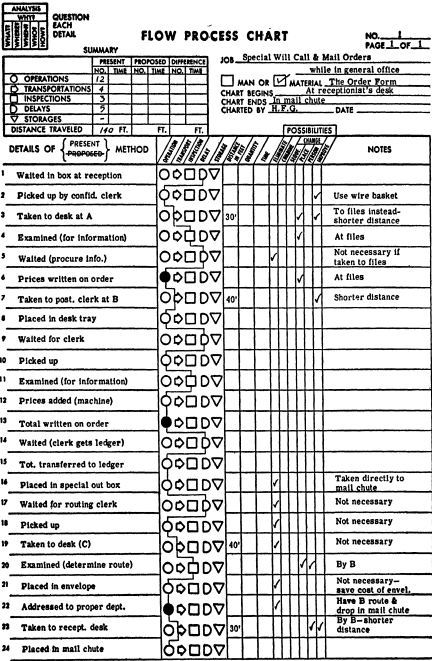
Figure 15-5. Process Flow Chart.
