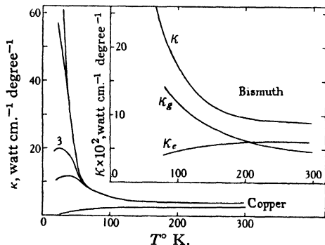
Fig. 33. Observed values of \kappa for copper. The trend of observed values of \kappa for bismuth, disregarding anisotropy. Curves show \kappa_e and \kappa_g as found experimentally.
