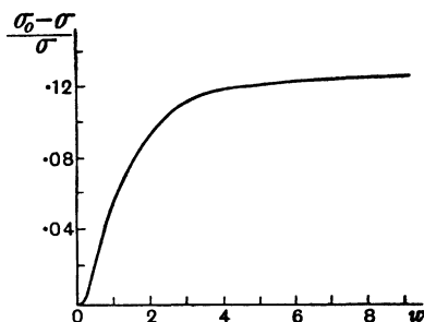
Fig. 30. The change in electrical resistance of a semi-conductor in a magnetic field. w = eHl/\{c(2\pi mkT)^{\frac{1}{2}}\} .
