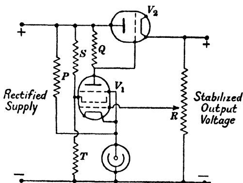
Fig. 6.11. Performance with V_1 , Mullard SP4B; V_2 , Osram KT41; Neon Mullard 7475; P , 250,000\ \Omega ; Q , 250,000\ \Omega ; R , 2\text{M}\Omega ; S , 40,000\ \Omega ; T , 50,000\ \Omega . Output voltage constant to \pm 0.2\% for current from 10 to 60 mA. Output current or voltage constant to \pm 0.5\% for A.C. inputs from 200 to 250 V.
