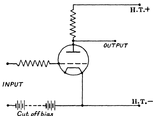
Fig. 7.9. Simple discriminator.
