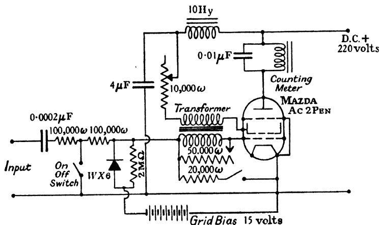
Fig. 8-10. Blocking oscillator.
