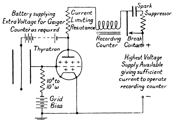
Fig. 9.4. Wynn-Williams external extinguishing circuit.
