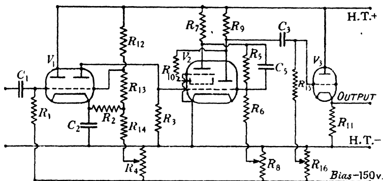
Fig. 7.11. Discriminator.
