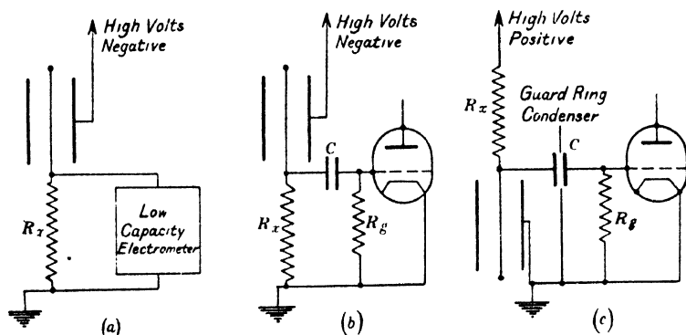
Fig. 9.2. Circuits for resistance extinguished counters.
