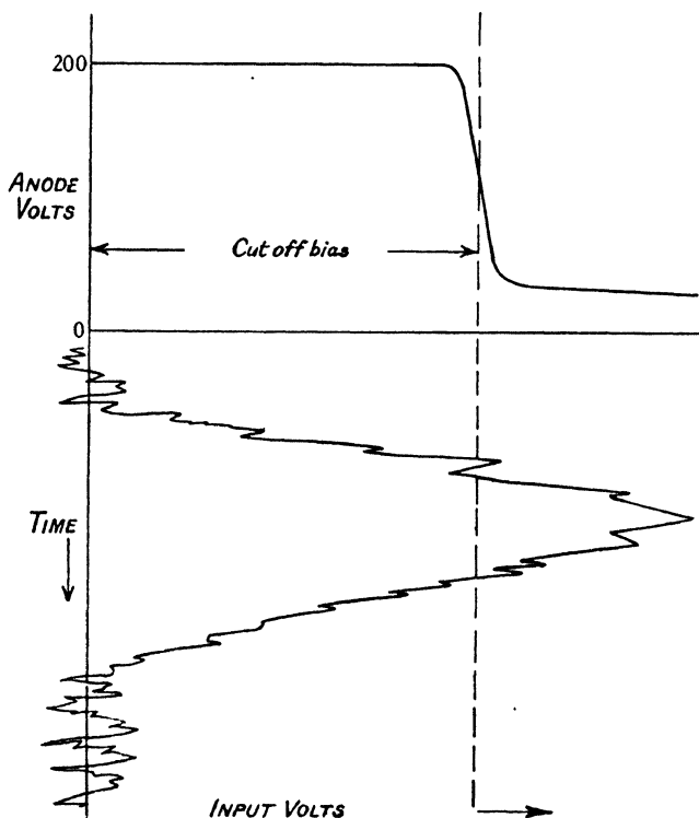
Fig. 7-10. Action of simple discriminator.
