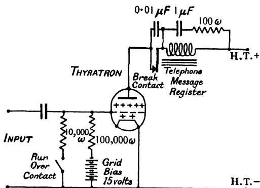
Fig. 8·8. Thyatron counter.
