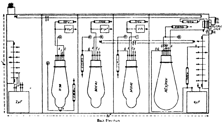
Fig. 4.14. Screened amplifier.
