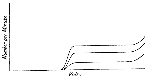
Fig. 9.1. Geiger counter "ideal" characteristic.
