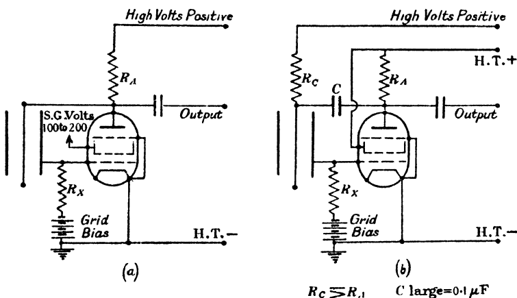
Fig. 9.3. Valve amplifying circuits for resistance extinction.
