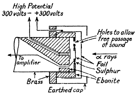
Fig. 2.3. Differential chamber.
