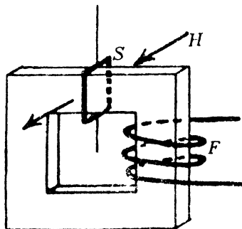
Fig. 5.2. Shire oscillograph.
