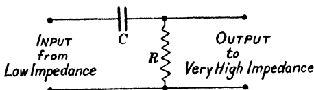
Fig. 11.3. Simple resistance-capacity filter.
