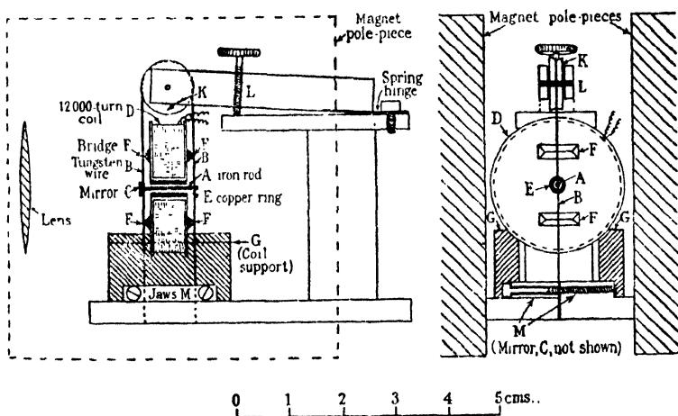
Fig. 5.1. Wynn-Williams oscillograph.
