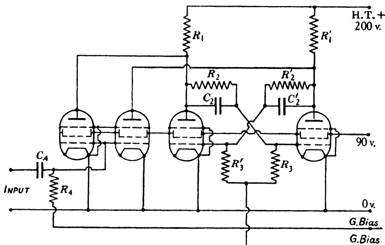
Fig. 8.4. Stevenson and Getting's scale-of-two unit. All valves Type 57.
