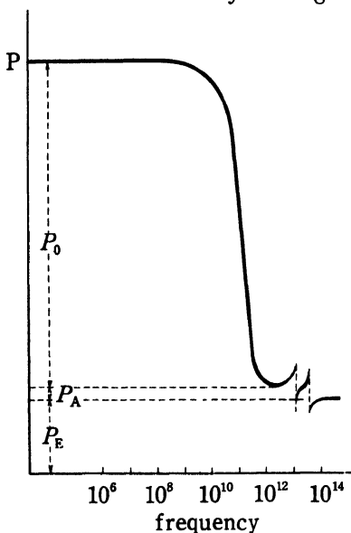
Fig. 1.14. Dependence of polarization on frequency.
