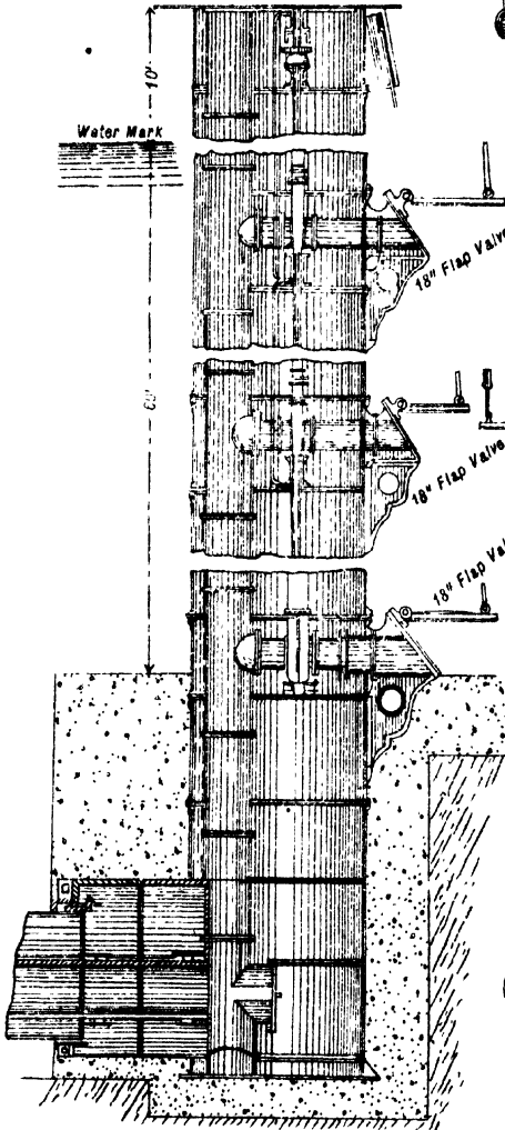
Fig. 5. SECTION.
