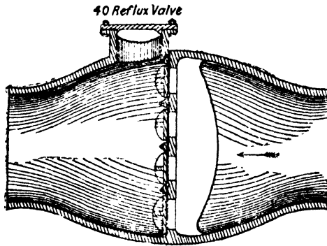
Vertical Section. Fig 60
