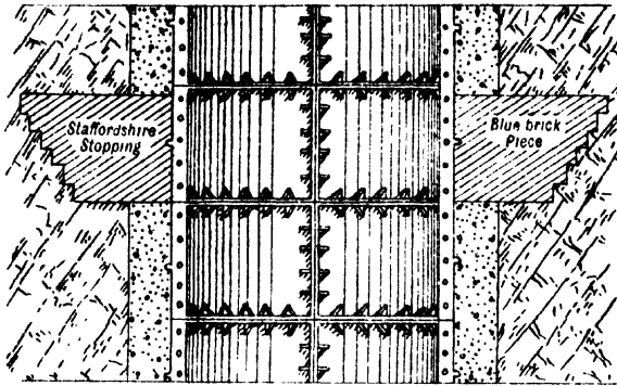
Fig. 5. SECTION.
