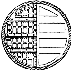
Vertical Section. Fig 60
