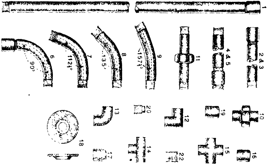
1 Tubes. 2 & 3 Make-up pieces 4 & 5 Long screws. 6 to 9 Bends. 10 & 11 Unions. 12 & 13 Elbows 14 Tees. 15 Crosses. 16 Sockets. 17 Tapers 18 Flanges 19 Caps 20 Plugs.
