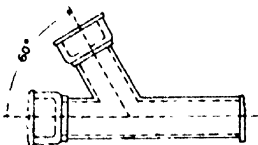
Angle Branch Pipes
