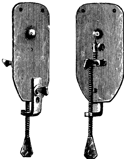
Fig. 4.—Leeuwenhoek's microscope (1673).
