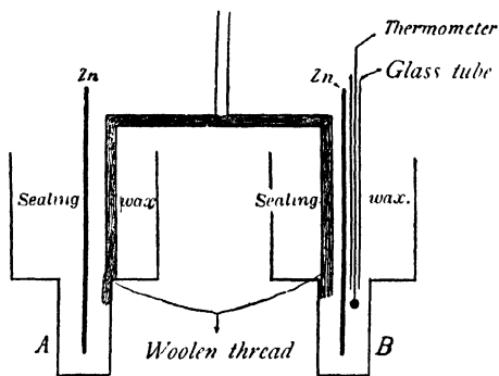
Transition cell
