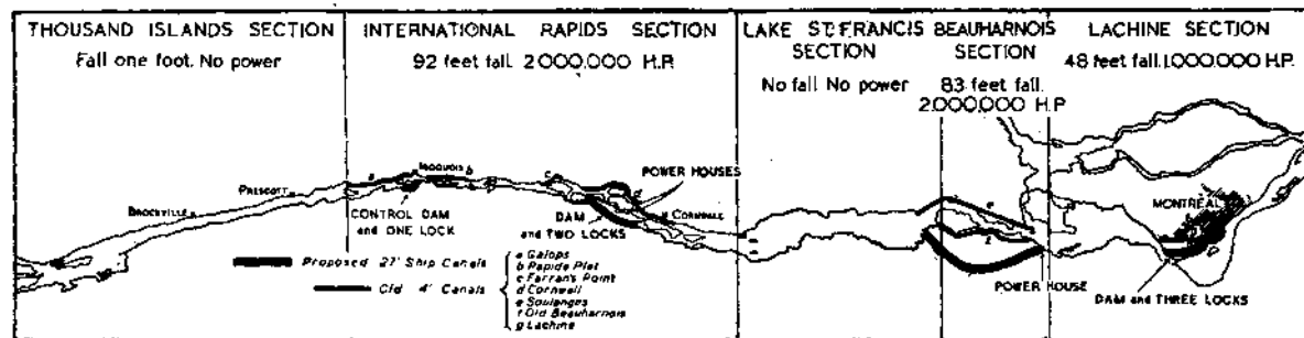
FIG. 1D6A.—Plan of St. Lawrence Deep Waterway Scheme,
